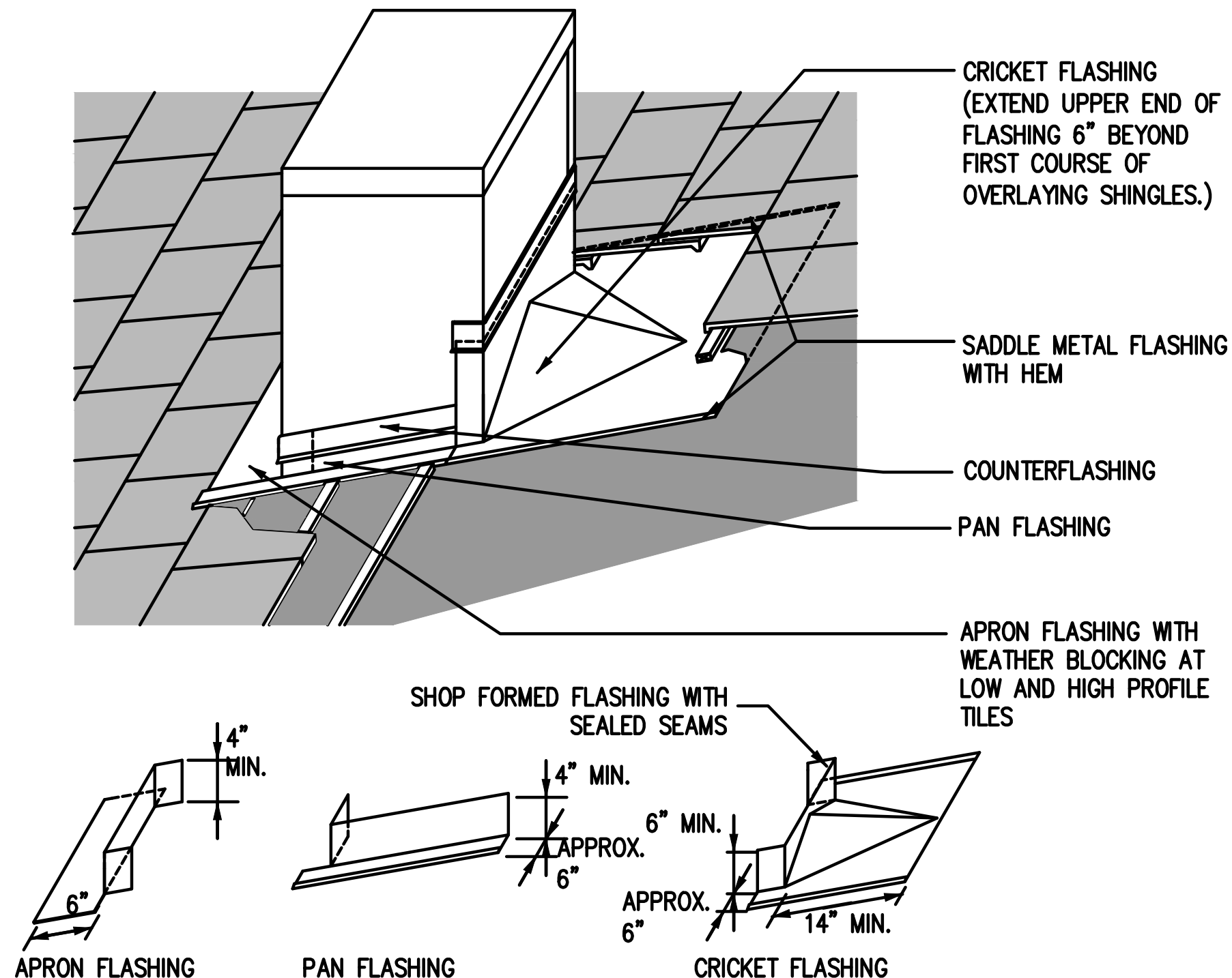
1 ROOF CURB FLASHING DETAIL A7 NOT TO SCALE
