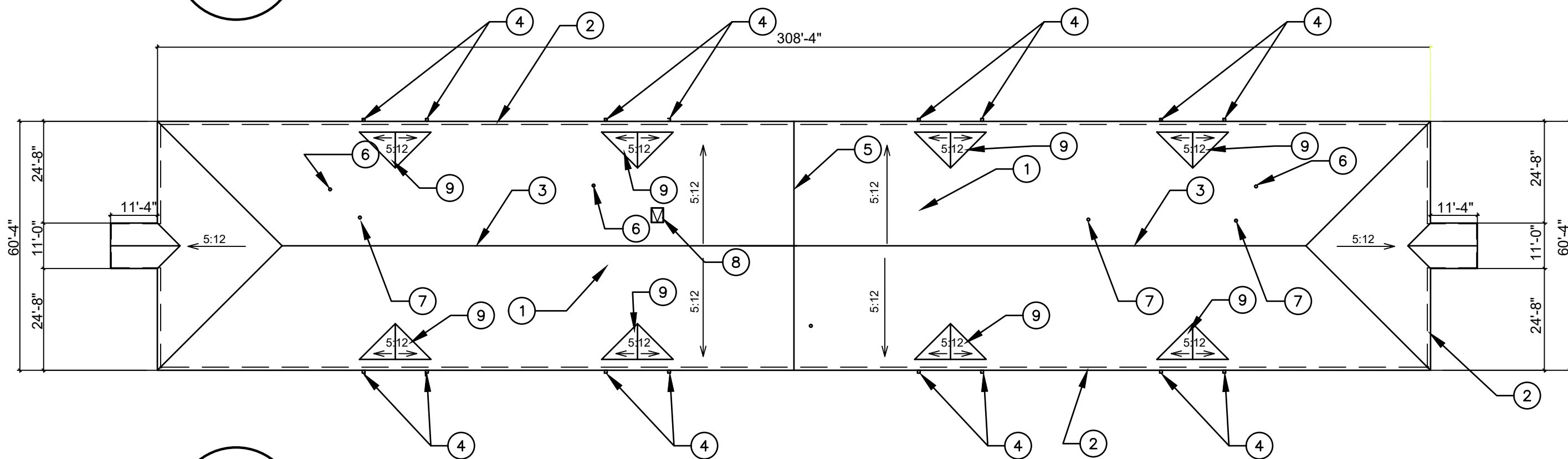
1 HP55 ROOF PLAN A4 NOT TO SCALE
