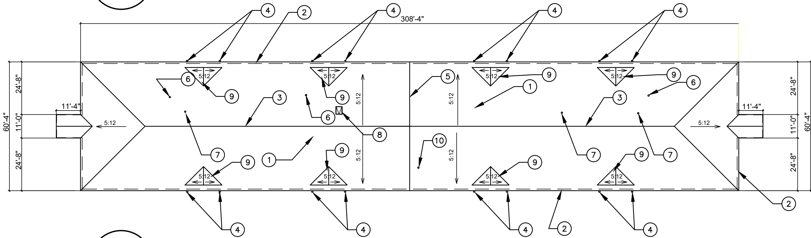
1 HP53 ROOF PLAN A3 NOT TO SCALE
