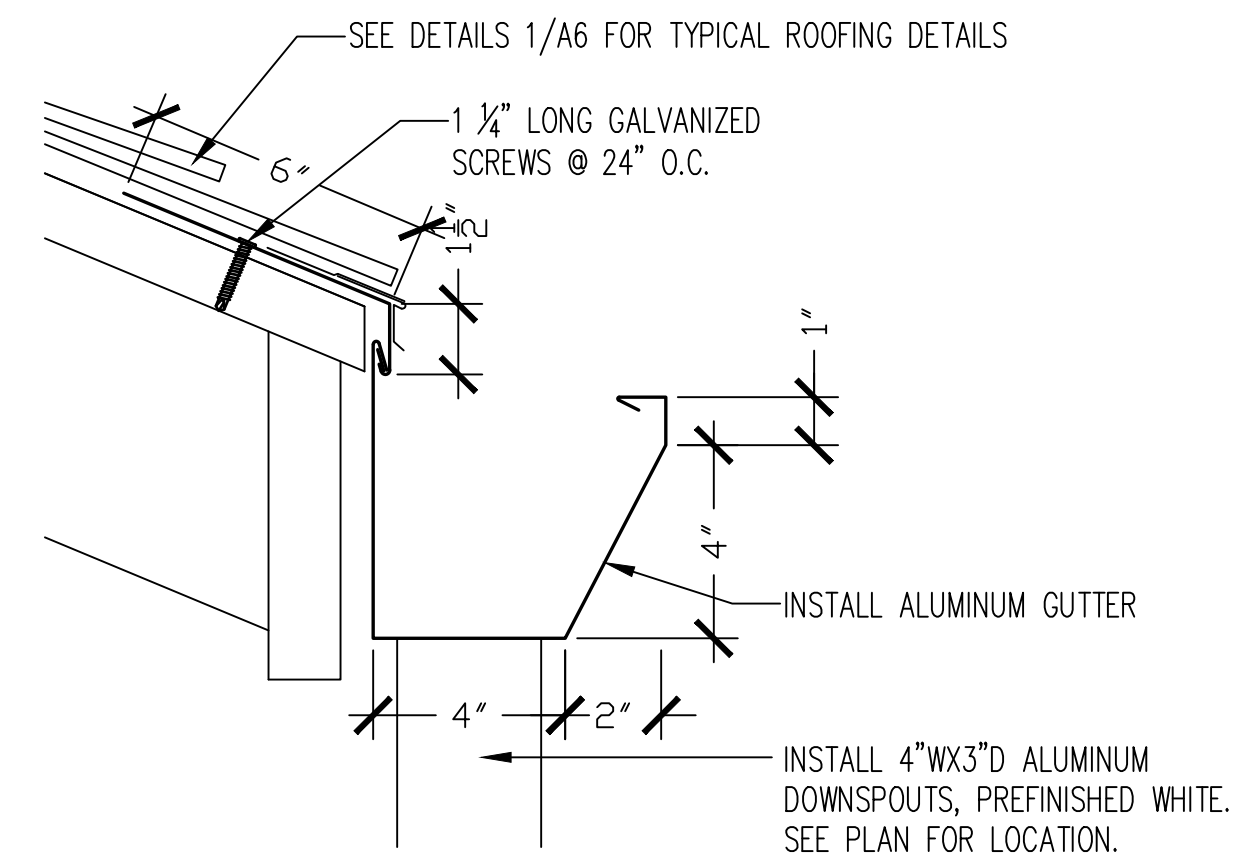
3 A6 TYPICAL GUTTER DETAIL 3" = 1'-0" 0 3" 6" 1'
