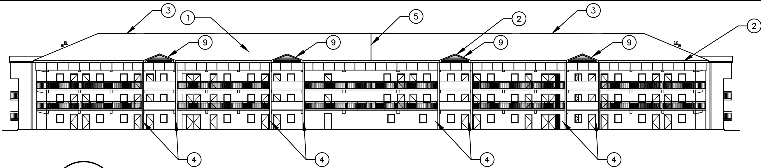
2 HP53 ELEVATION A3 NOT TO SCALE
