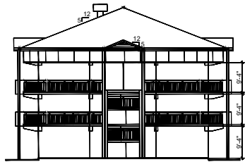
BLDG. HP255 - NORTH/SOUTH ELEVATION - EXISTING CONDITIONS NTS
