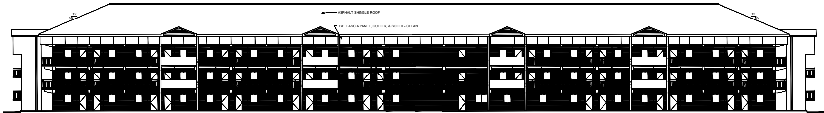
1 BLDG. HP265 - NORTH ELEVATION - EXISTING CONDITIONS NTS
