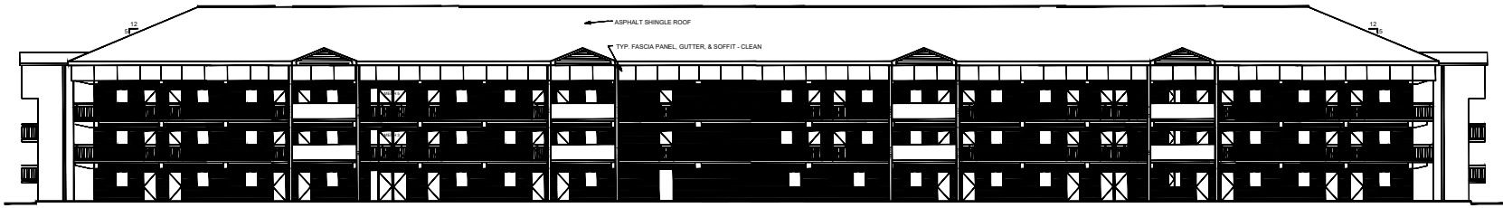
BLDG. HP255 - EAST ELEVATION - EXISTING CONDITIONS NTS
