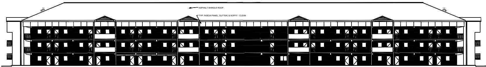
BLDG. HP255 - WEST ELEVATION - EXISTING CONDITIONS NTS
