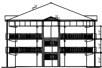
1 BLDG. HP265 - EAST/WEST ELEVATION - EXISTING CONDITIONS NTS
