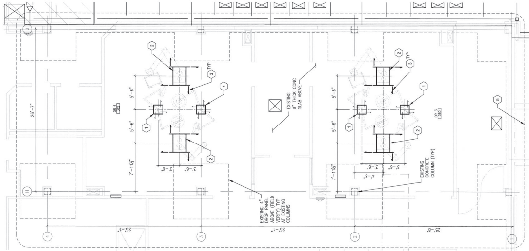
EXISTING MAIN ROOF STRUCTURE ABOVE SHOWN TOC EL. 138'-8" FIELD VERIFY
