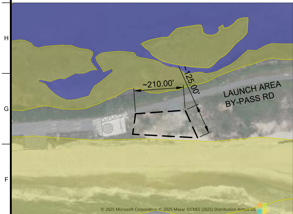
E1 LAYDOWN AREA 1 1" = 200'-0"
