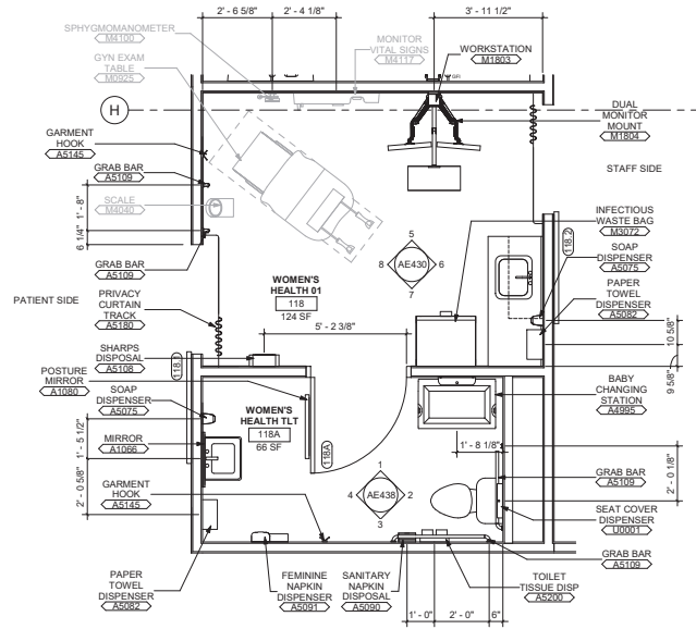
3 WMN'S HEALTH EXAM ROOM AND TOILET - ENLARGED FLOOR PLAN 12' x 10'
