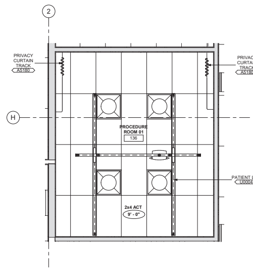
2 TYP PROCEDURE ROOM - ENLARGED REFLECTED CEILING PLAN 12' x 10'
