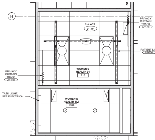
4 WMN'S HEALTH EXAM ROOM AND TOILET - REFLECTED CEILING PLAN 12' x 10'
