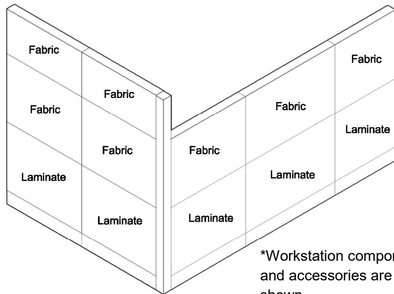
Exterior Isometric of Tile Layout for TYP-01 Panel Supported Workstation
