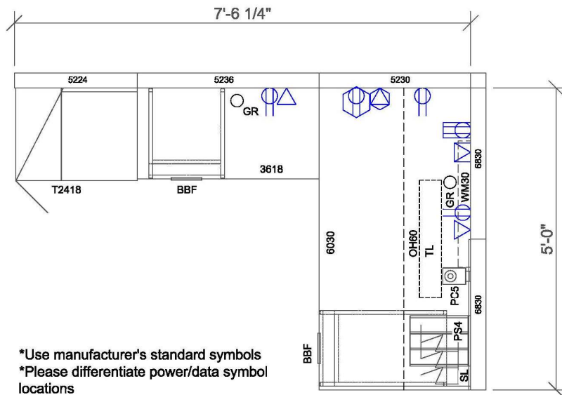
Electric Plan for TYP-01 Panel Supported Workstation
