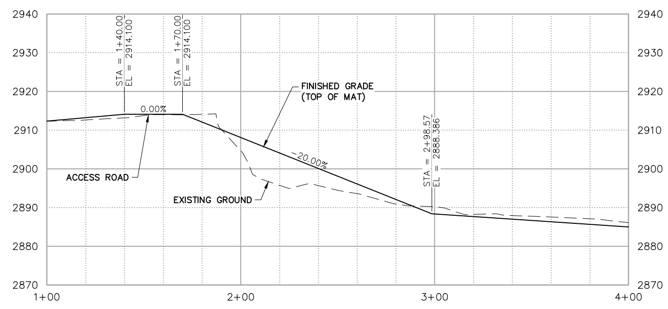
PROFILE SPILLWAY
