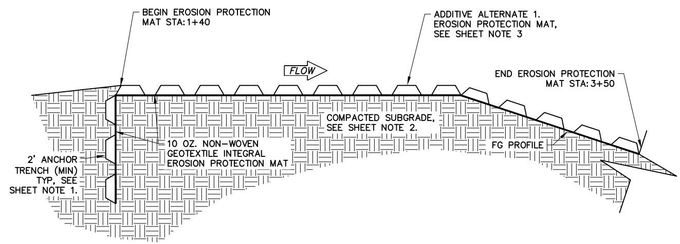
A SECTION EROSION PROTECTION MAT
