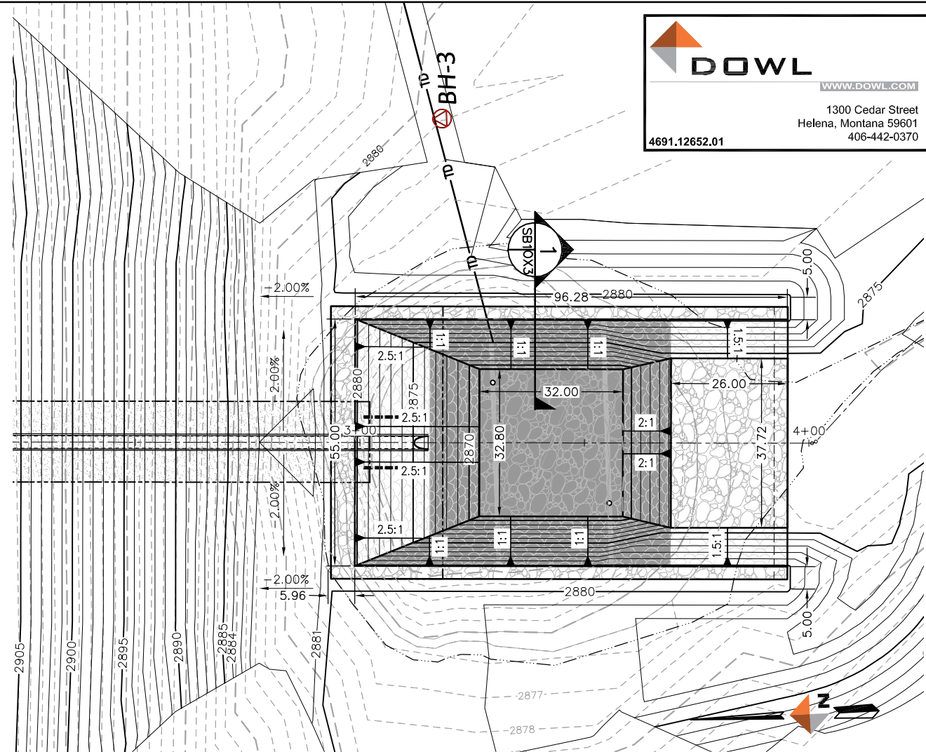
PLAN RIPRAP STILLING BASIN
