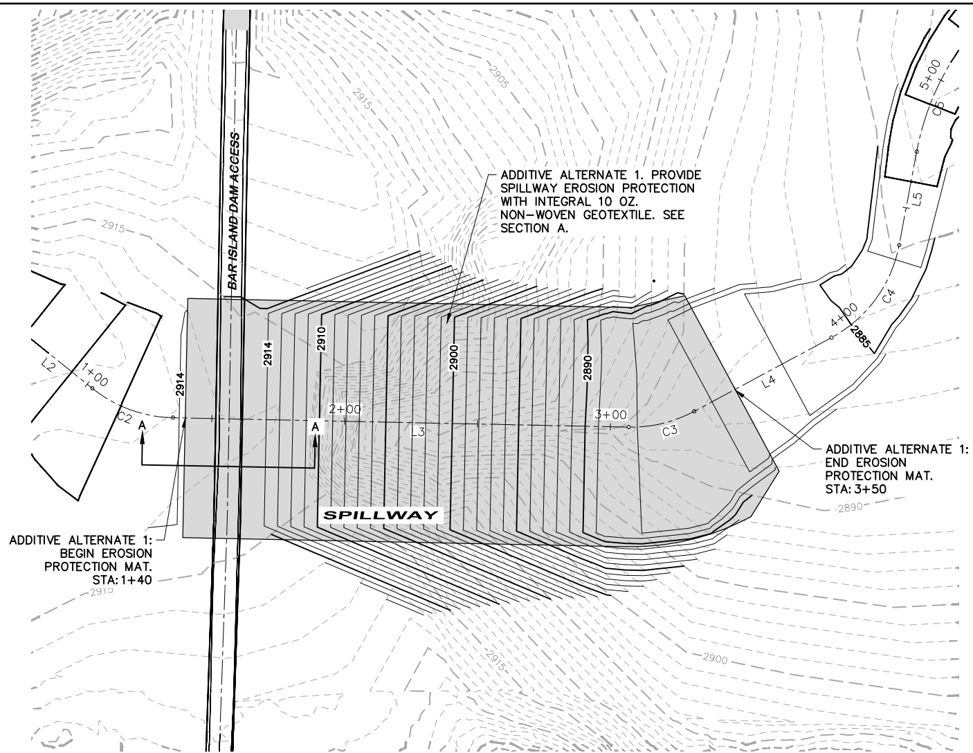
PLAN SPILLWAY
