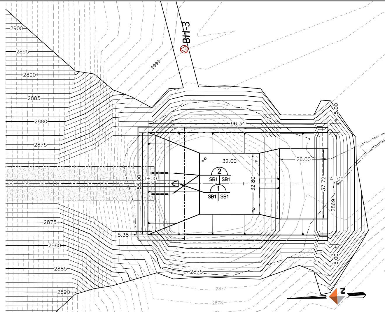
PLAN STILLING BASIN EXCAVATION
