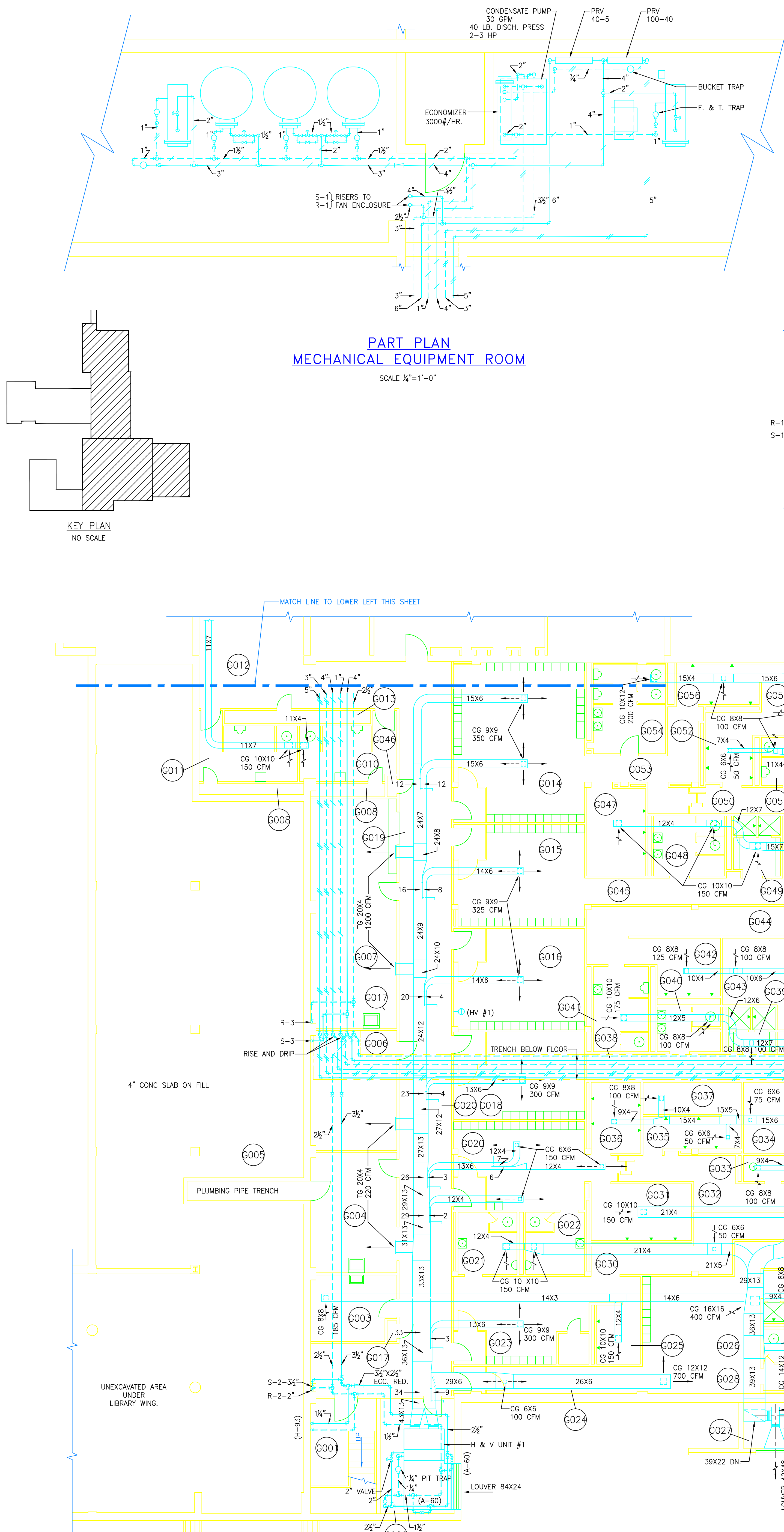
GROUND FLOOR PLAN-NORTH PORTION SCALE 1/8"=1'-0"
