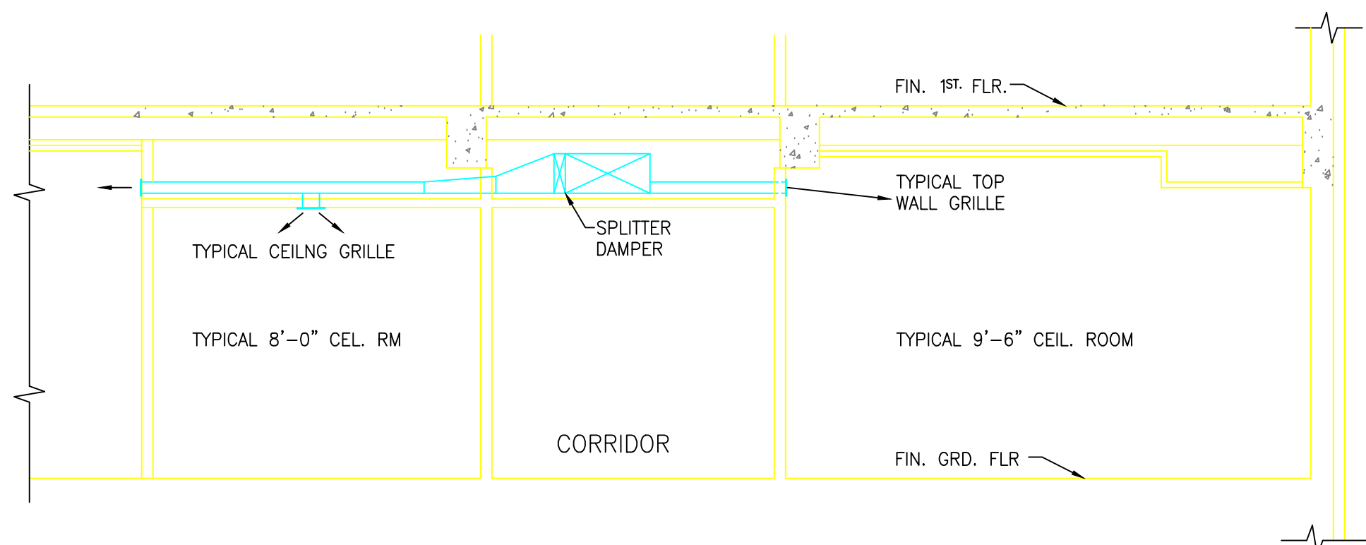
TYPICAL SECTION—GROUND FLOOR CORRIDOR
