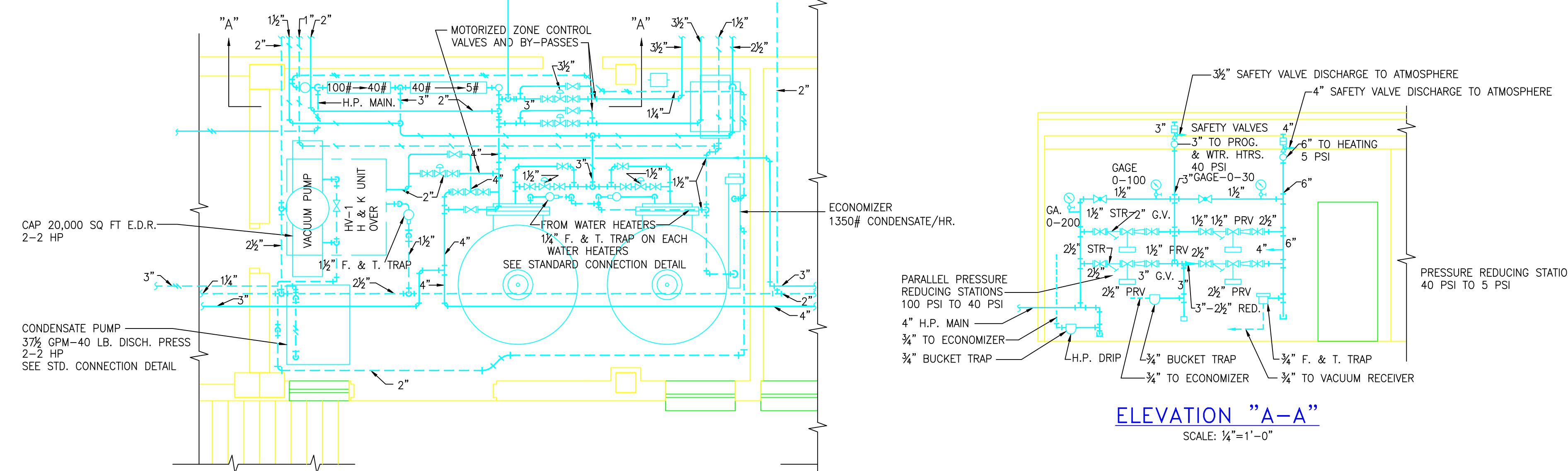
PLAN OF MECHANICAL EQUIPMENT ROOM
