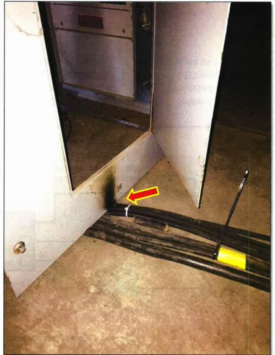
208V and 480V cables damaged
