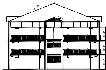
BLDG. FC574 - NORTH/SOUTH ELEVATION - EXISTING CONDITIONS NTS
