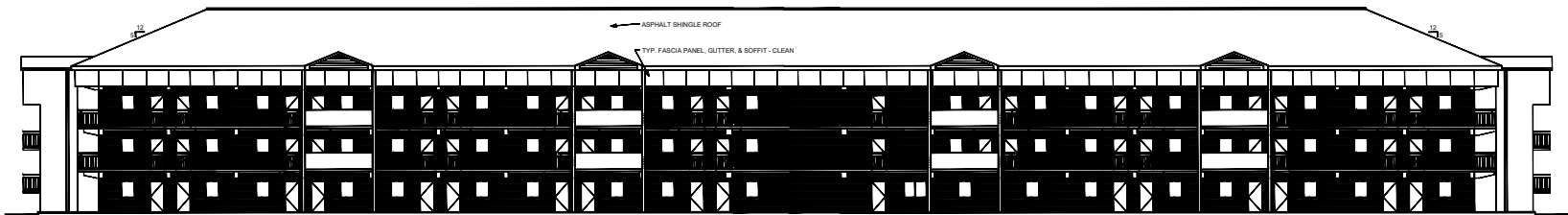
BLDG. FC574 - EAST ELEVATION - EXISTING CONDITIONS NTS
