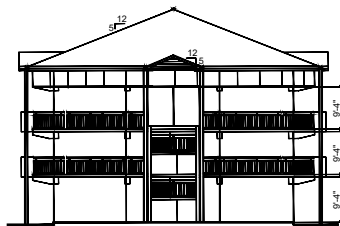
BLDG. FC573 - NORTH/SOUTH ELEVATION - EXISTING CONDITIONS NTS
