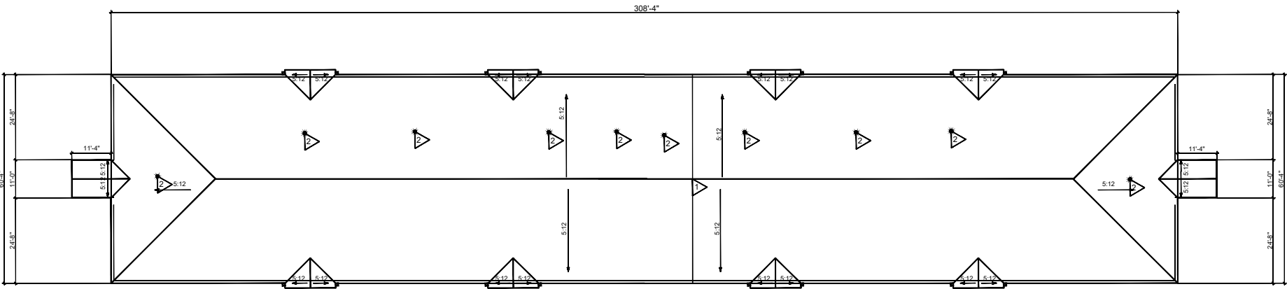
1 BLDG. FC525 - ROOF PLAN - EXISTING CONDITIONS NTS
