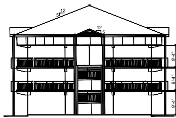
1 BLDG. FC525 - NORTH/SOUTH ELEVATION - EXISTING CONDITIONS NTS
