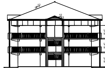
1 BLDG. FC520 - NORTH/SOUTH ELEVATION - EXISTING CONDITIONS NTS
