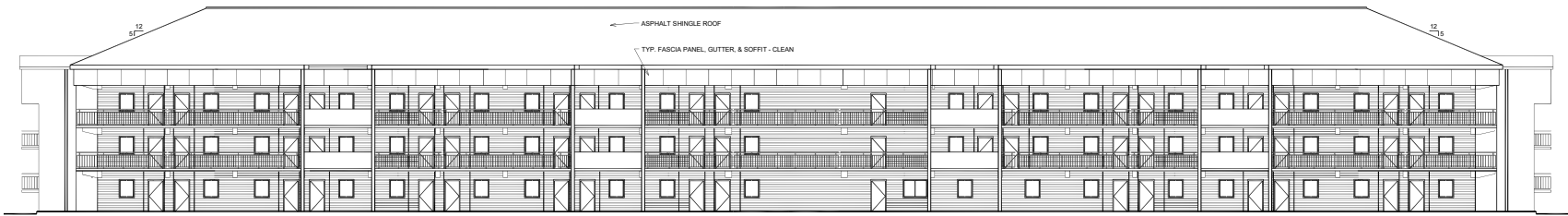
BLDG. FC571 - EAST ELEVATION - EXISTING CONDITIONS NTS
