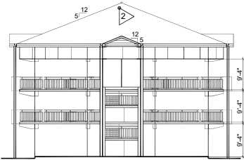
BLDG. FC571 - NORTH/SOUTH ELEVATION - EXISTING CONDITIONS NTS
