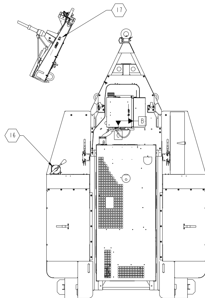
UNIT A GENSET G1
