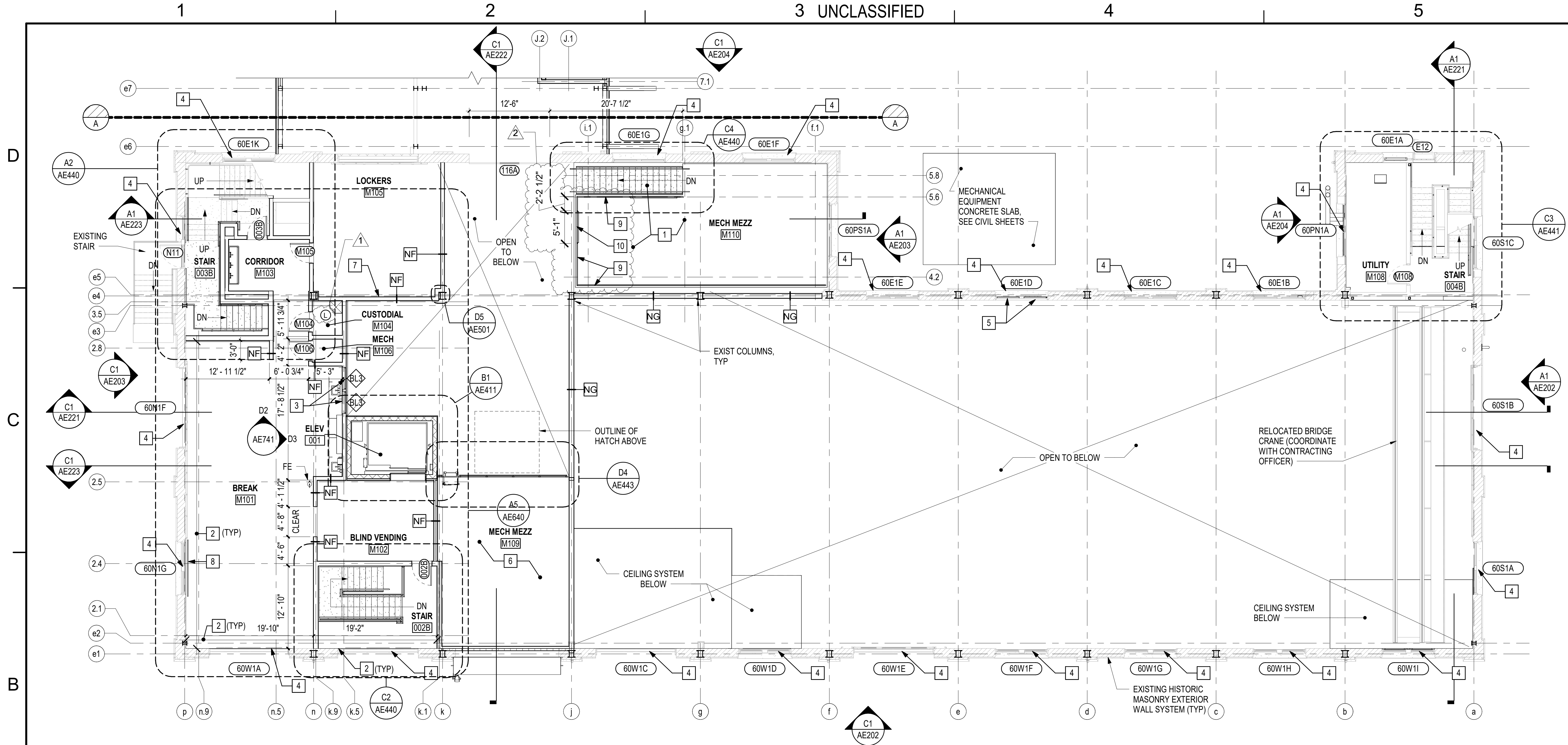
B1 FIRST FLOOR MEZZANINE PART PLAN - WEST SCALE: 1/8" = 1'-0"
