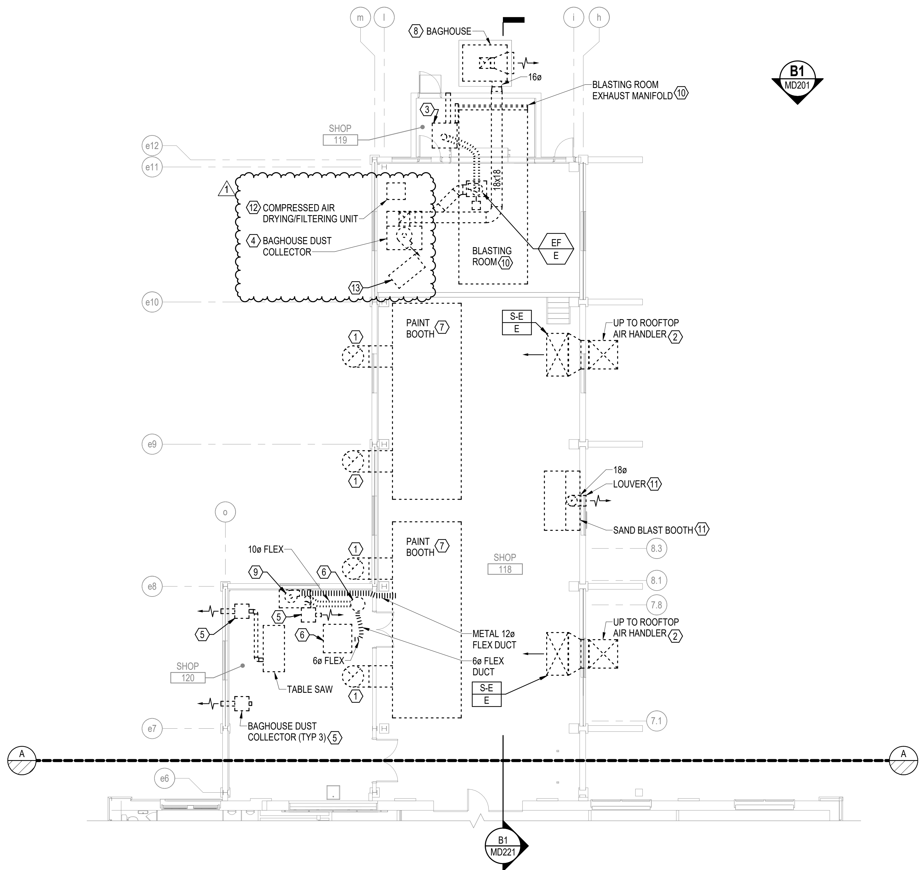
A1 FIRST FLOOR MECHANICAL DUCTWORK REMOVALS PLAN - EAST SCALE: 1/8" = 1'-0"
