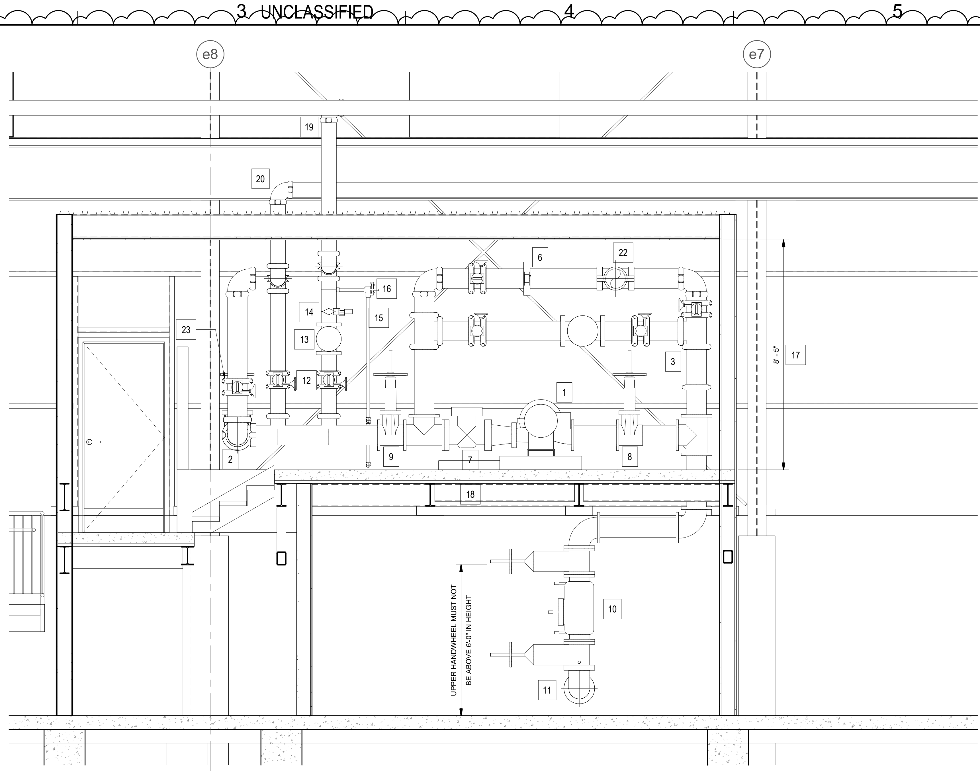
B2 FIRE PUMP ROOM SECTION SCALE: 1/2" = 1'-0"
