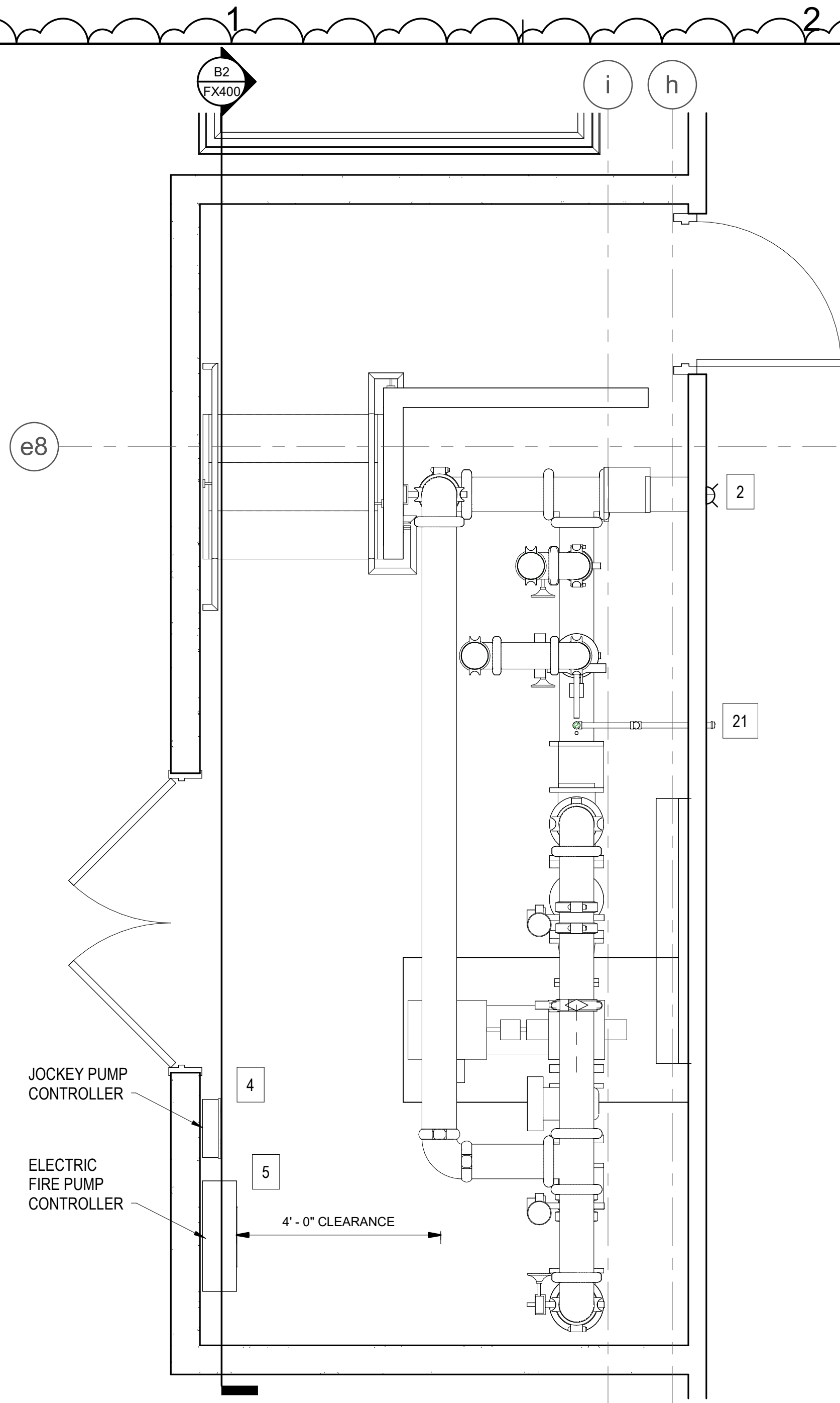
B1 ENLARGED FIRE PUMP ROOM SCALE: 1/2" = 1'-0"
