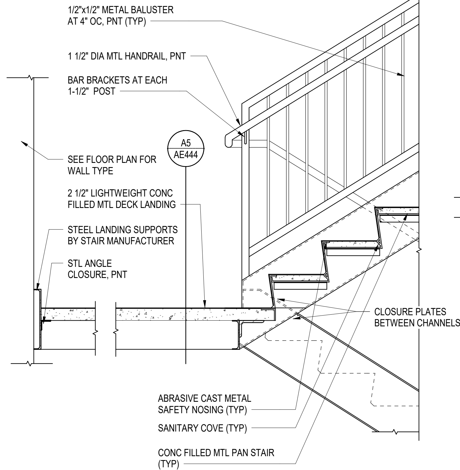
C2 STAIR LANDING DETAIL (TYP) SCALE: 1" = 1'-0" (AE442)
