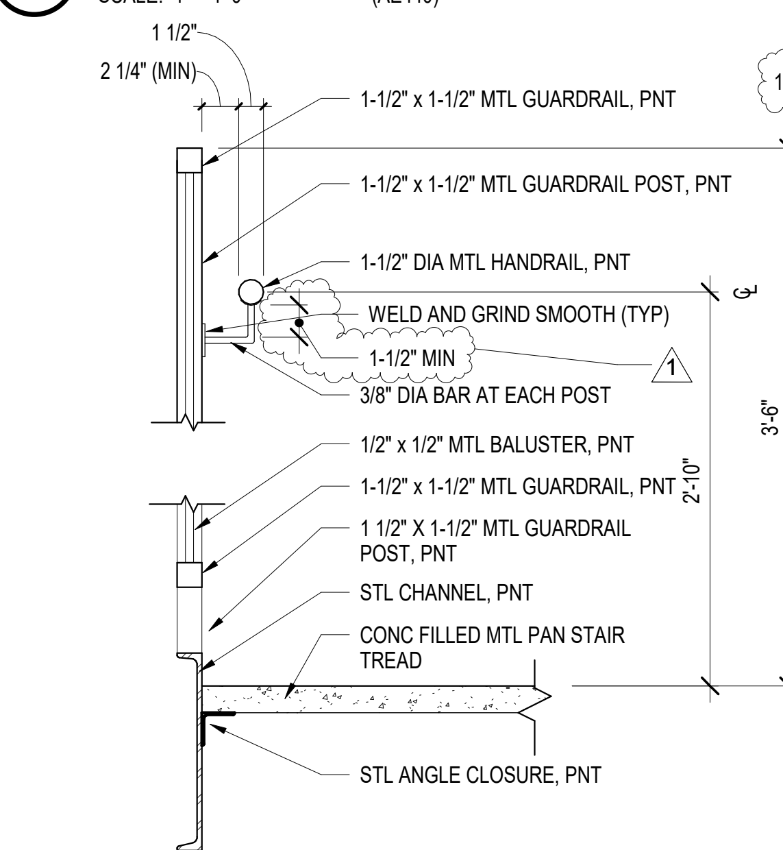
B4 STAIR LANDING FLOOR LEVEL EDGE DETAIL (TYP) SCALE: 1 1/2" = 1'-0" (AE444)
