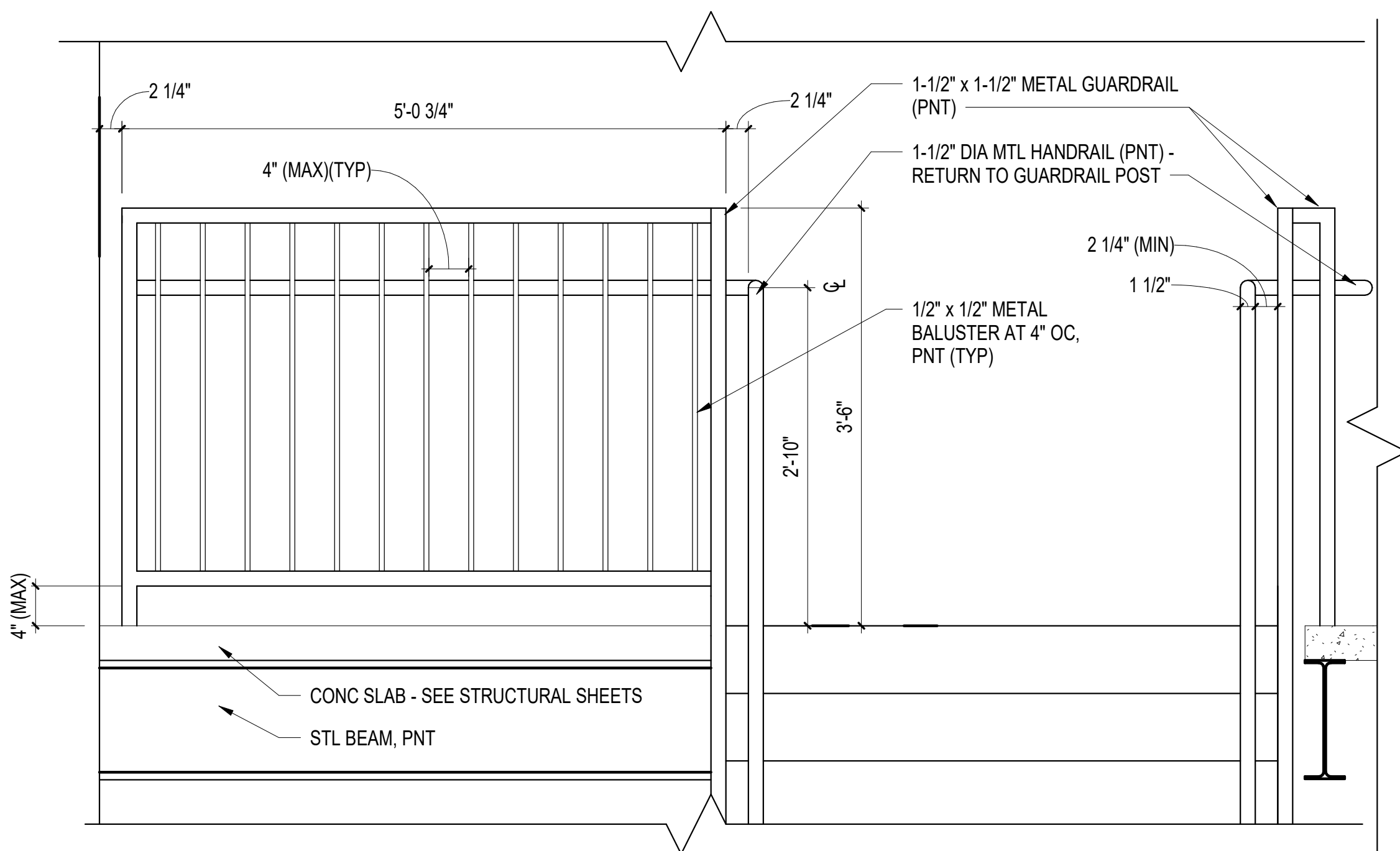
C4 STAIR TOP LANDING DETAIL (TYP) SCALE: 1" = 1'-0" (AE440)
