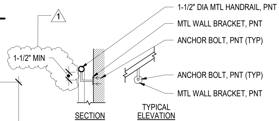
C5 STAIR RAILING DETAIL (TYP) SCALE: 1" = 1'-0" (AE444)
