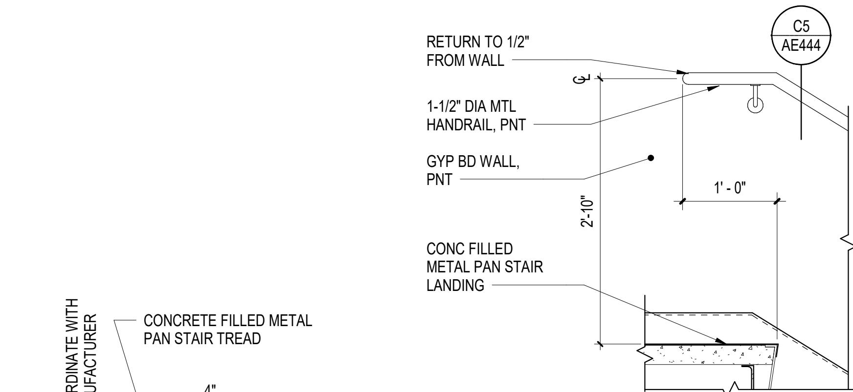
A2 STAIR HANDRAIL DETAIL (TYP) SCALE: 1" = 1'-0" (AE442)
