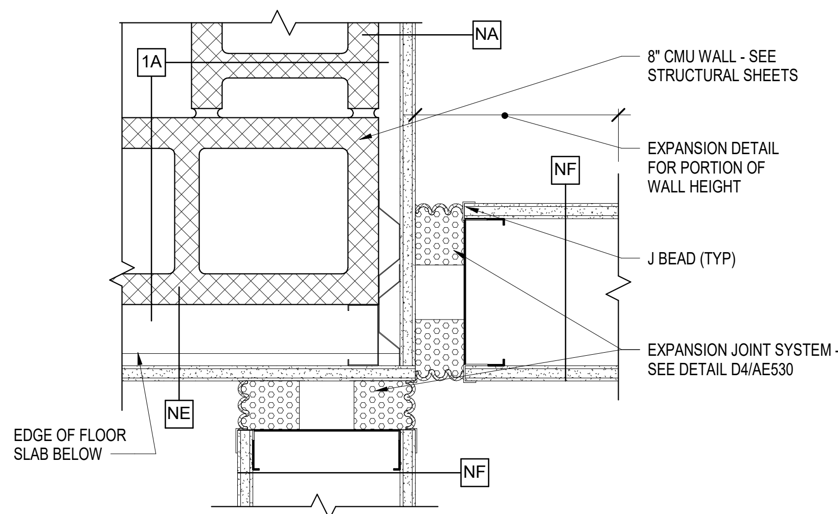
B4 ELEVATOR/FLOOR EXPANSION JOINT PLAN DETAIL 1 SCALE: 3" = 1'-0" (AE411)
