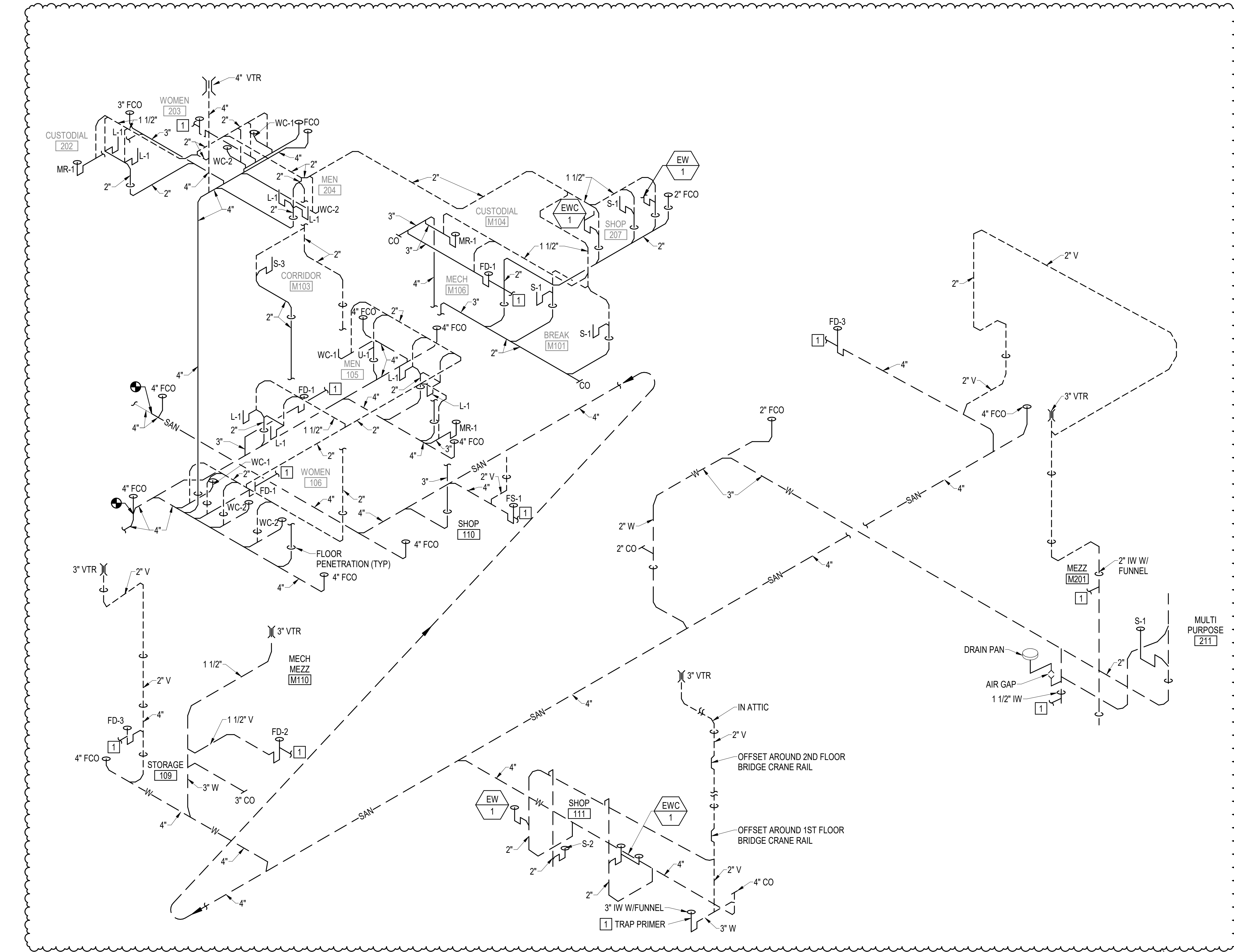
C1 SANITARY AND VENT PLUMBING RISER DIAGRAM SCALE: NOT TO SCALE
