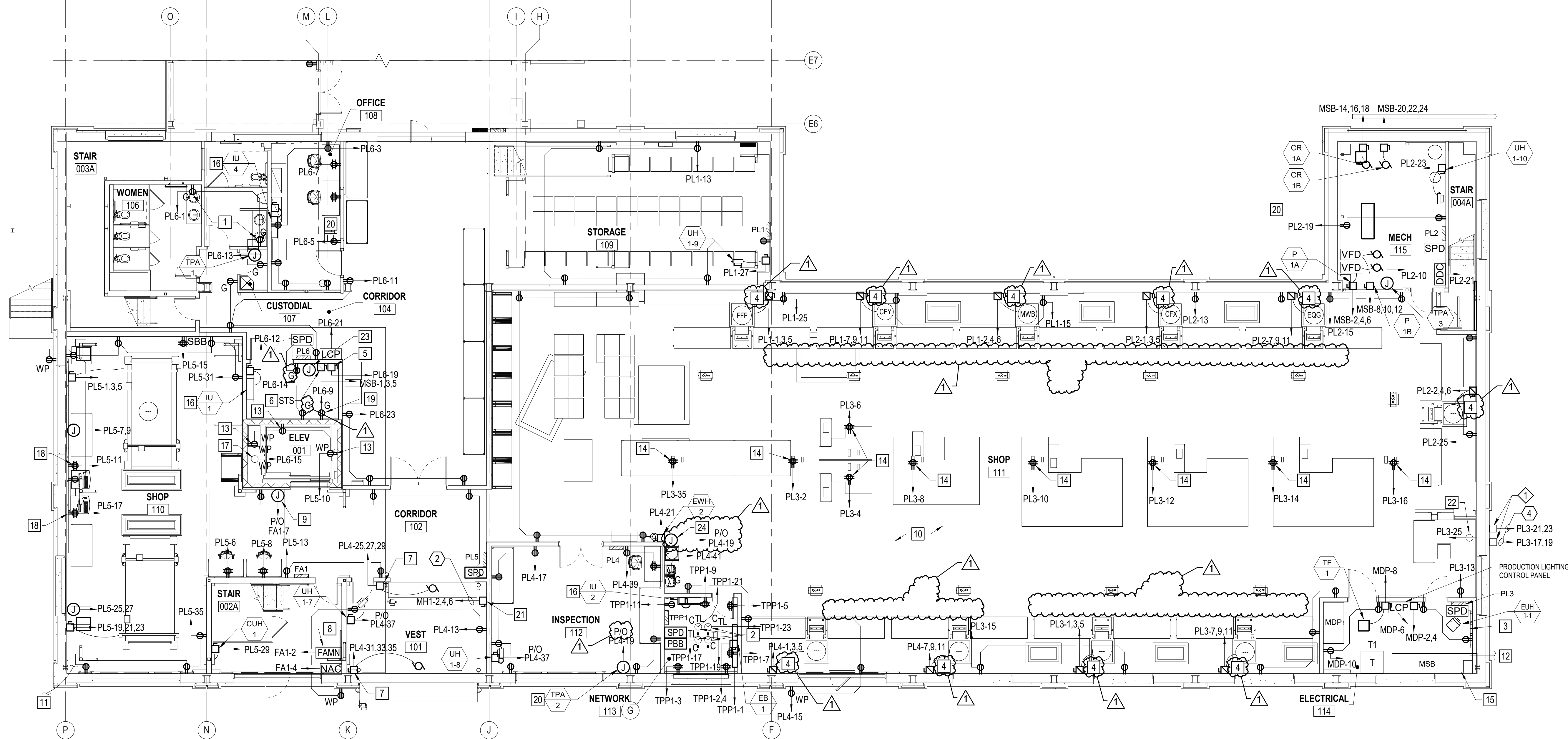
B1 FIRST FLOOR POWER PART PLAN - WEST SCALE: 1/8" = 1'-0"
