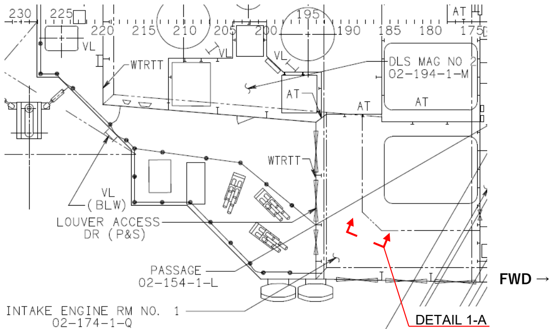
PLAN VIEW 02 LEVEL DECK WEATHER, FR 175 – 230, STBD
