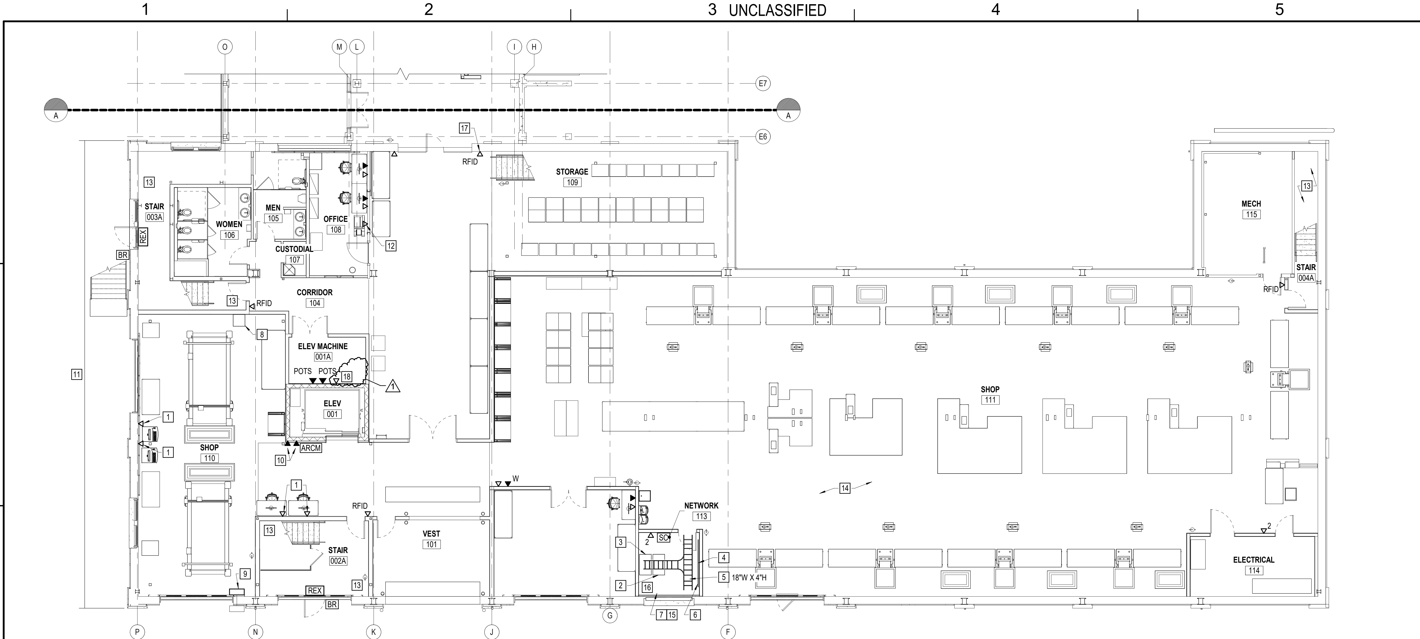
B1 FIRST FLOOR TECHNOLOGY AND SECURITY PART PLAN - WEST SCALE: 1/8" = 1'-0"
