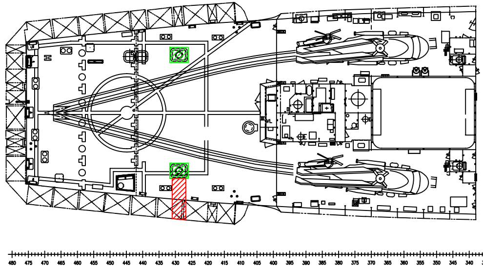
PLAN VIEW MAIN DECK
