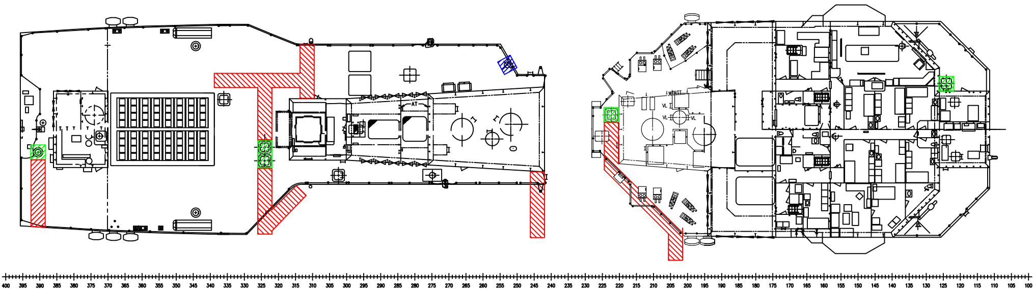
PLAN VIEW 02 LEVEL
