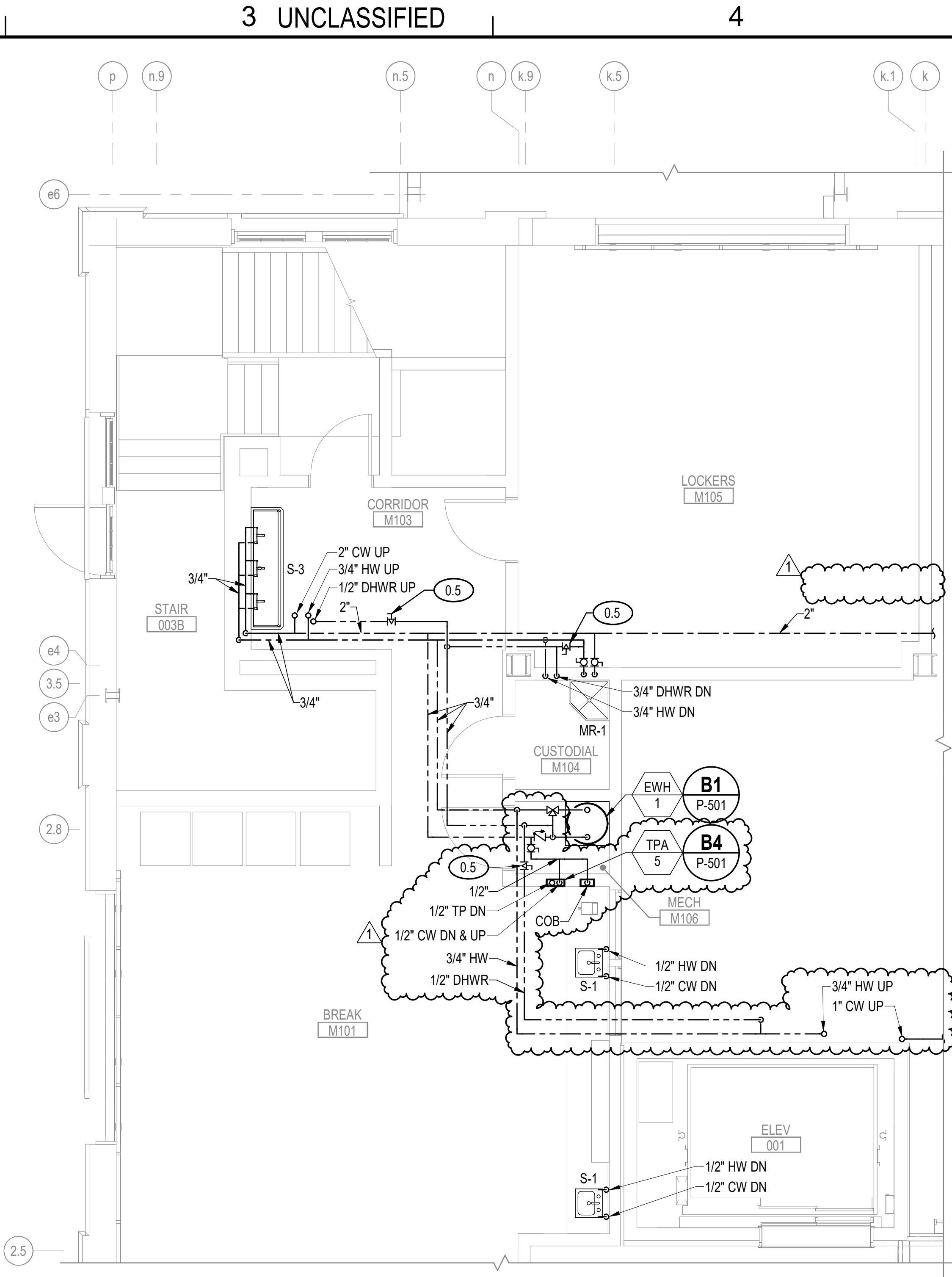
A3 ENLARGED FIRST FLOOR MEZZANINE DOMESTIC WATER SUPPLY PART PLAN SCALE: 1/4" = 1'-0" (P-106)
