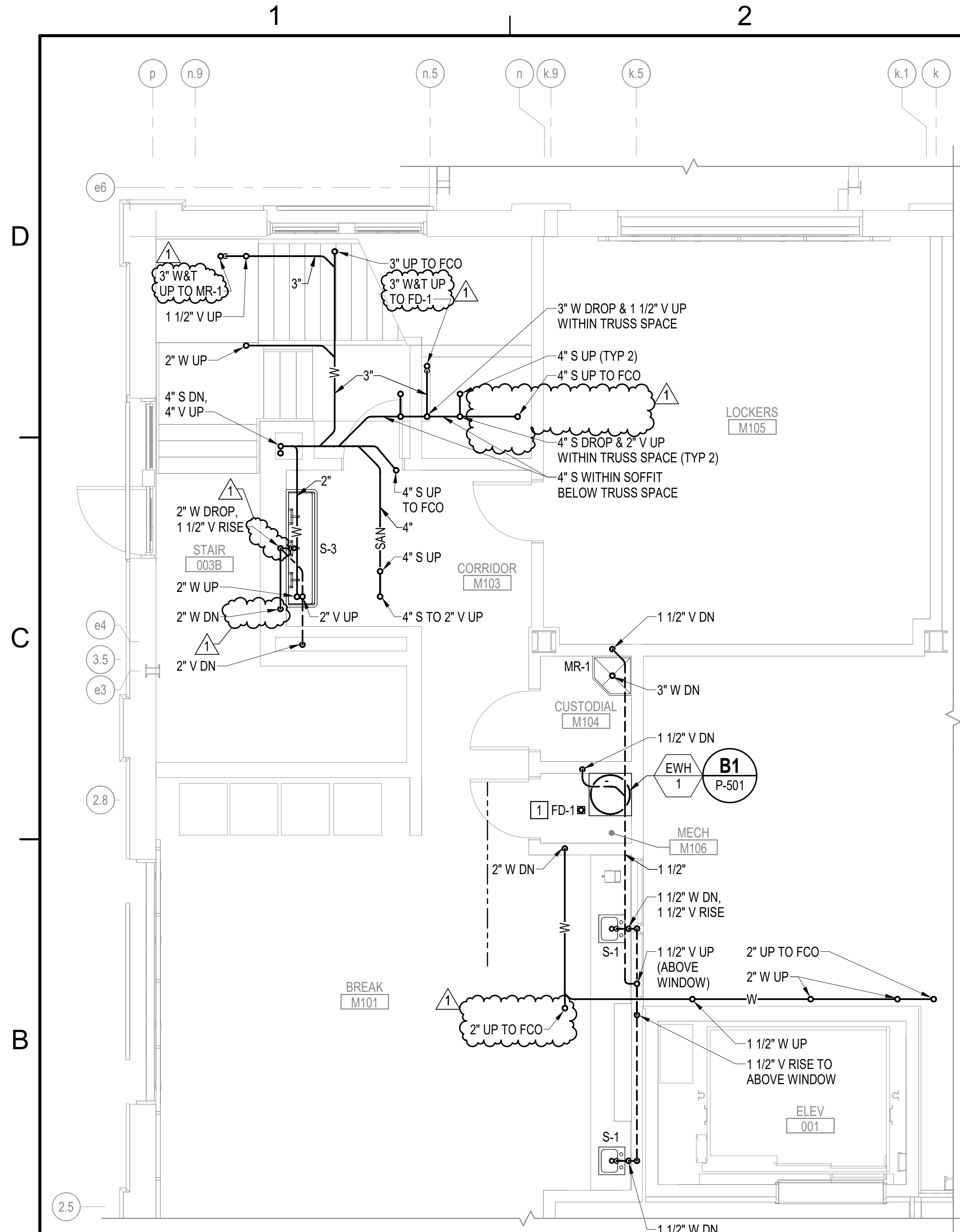
A1 ENLARGED FIRST FLOOR MEZZANINE SANITARY WASTE AND VENT PART PLAN SCALE: 1/4" = 1'-0" (P-106)
