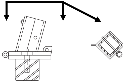
DETAIL 4-C Toggle Pin of Stanchion Base to Stanchion
