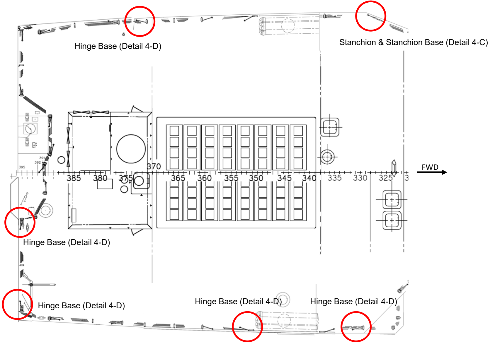
PLAN VIEW 2-A 02 LVL WEA DECK, FR 322 – 396 PORT & STBD
