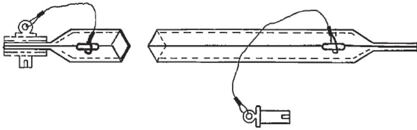
DETAIL 4-A Toggle Pin of Brace to Brace Clip & Stanchion
