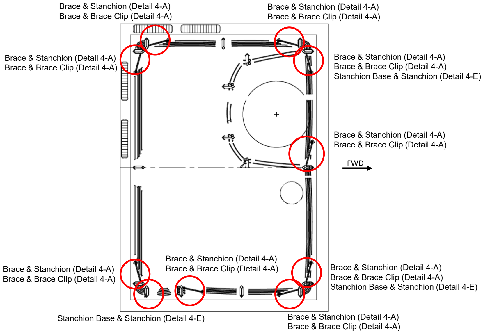
PLAN VIEW 3-A 02 1/2 LVL DECK, FR 370 - 386, PORT & STBD
