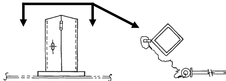
DETAIL 4-E Toggle Pin of Stanchion Base to Stanchion
