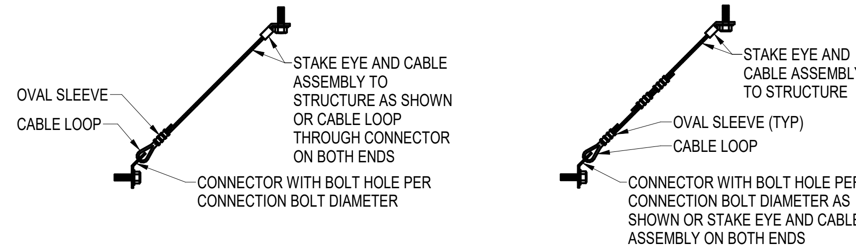
D4 ATFP CABLE BRACING ASSEMBLY DETAIL SCALE: NOT TO SCALE
