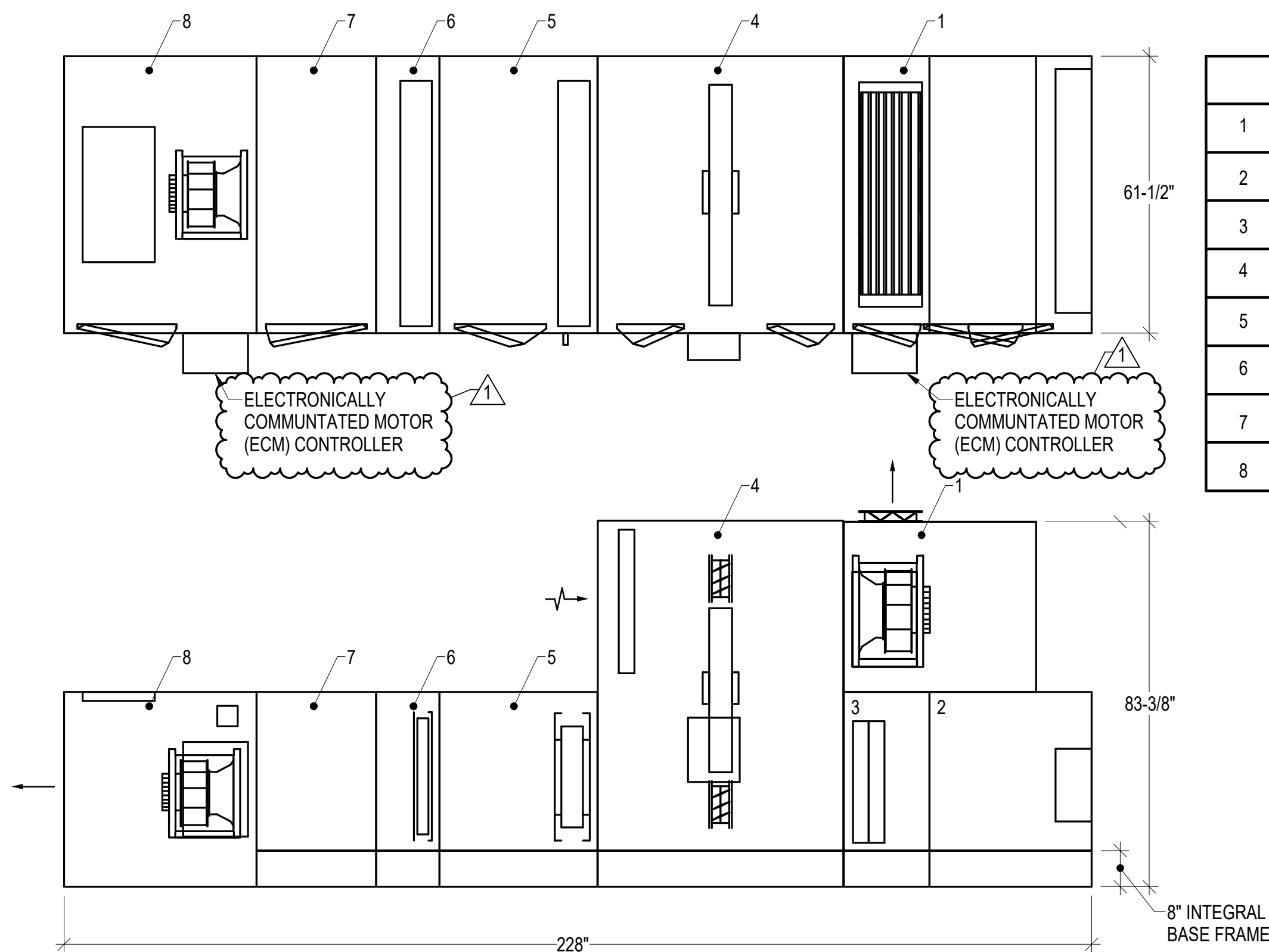
C1 DOAS-1 AIR HANDLING UNIT DIAGRAM (BOD) SCALE: NOT TO SCALE (MH102, MP104)
