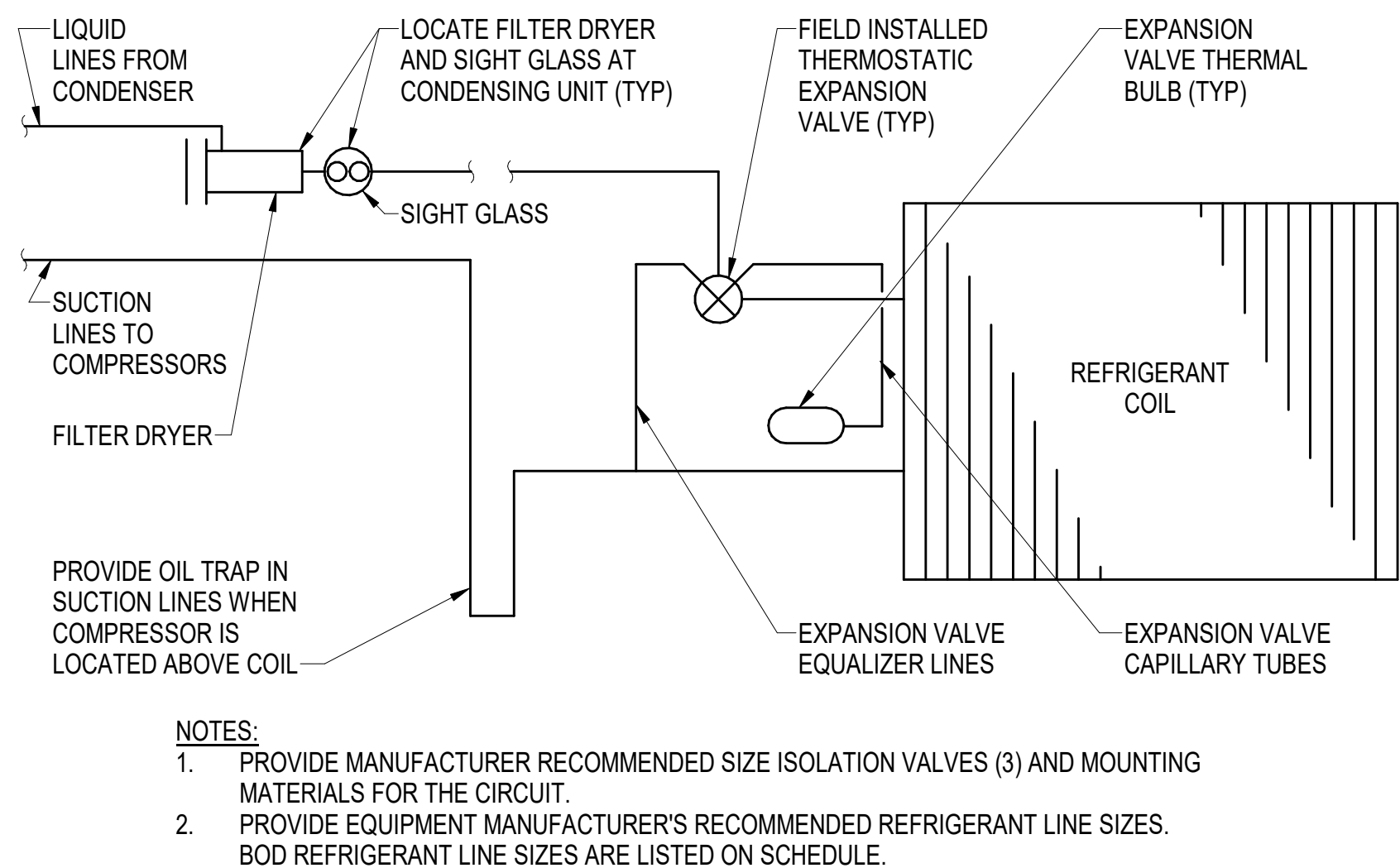
A2 DUCTED SPLIT SYSTEMS BCU-1/CU-1, BCU-2/CU-2, AND BCU-3/CU-3 REFRIGERANT COIL PIPING SCHEMATIC - SINGLE CIRCUIT SCALE: NOT TO SCALE (MP104, MP105, MP106)
