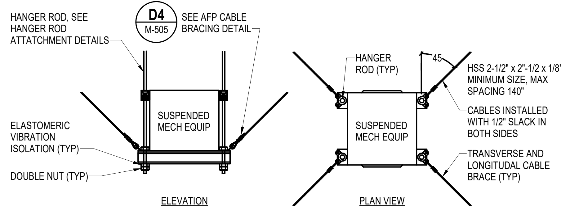
D4 ATFP CABLE BRACING ASSEMBLY DETAIL SCALE: NOT TO SCALE
