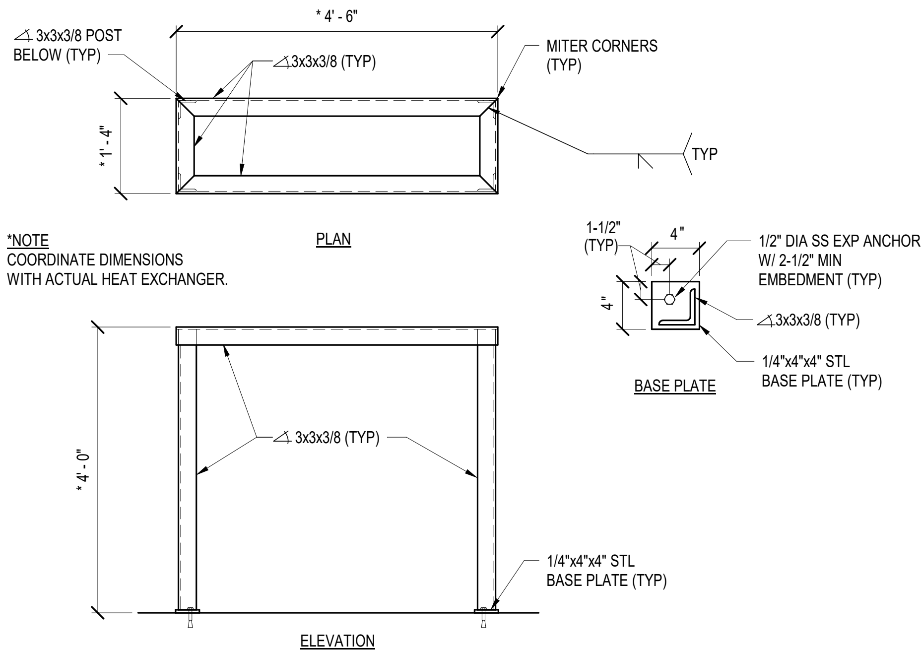
A2 HEAT EXCHANGER SUPPORT FRAME DETAIL SCALE: 3/4" = 1'-0" (M-504)
