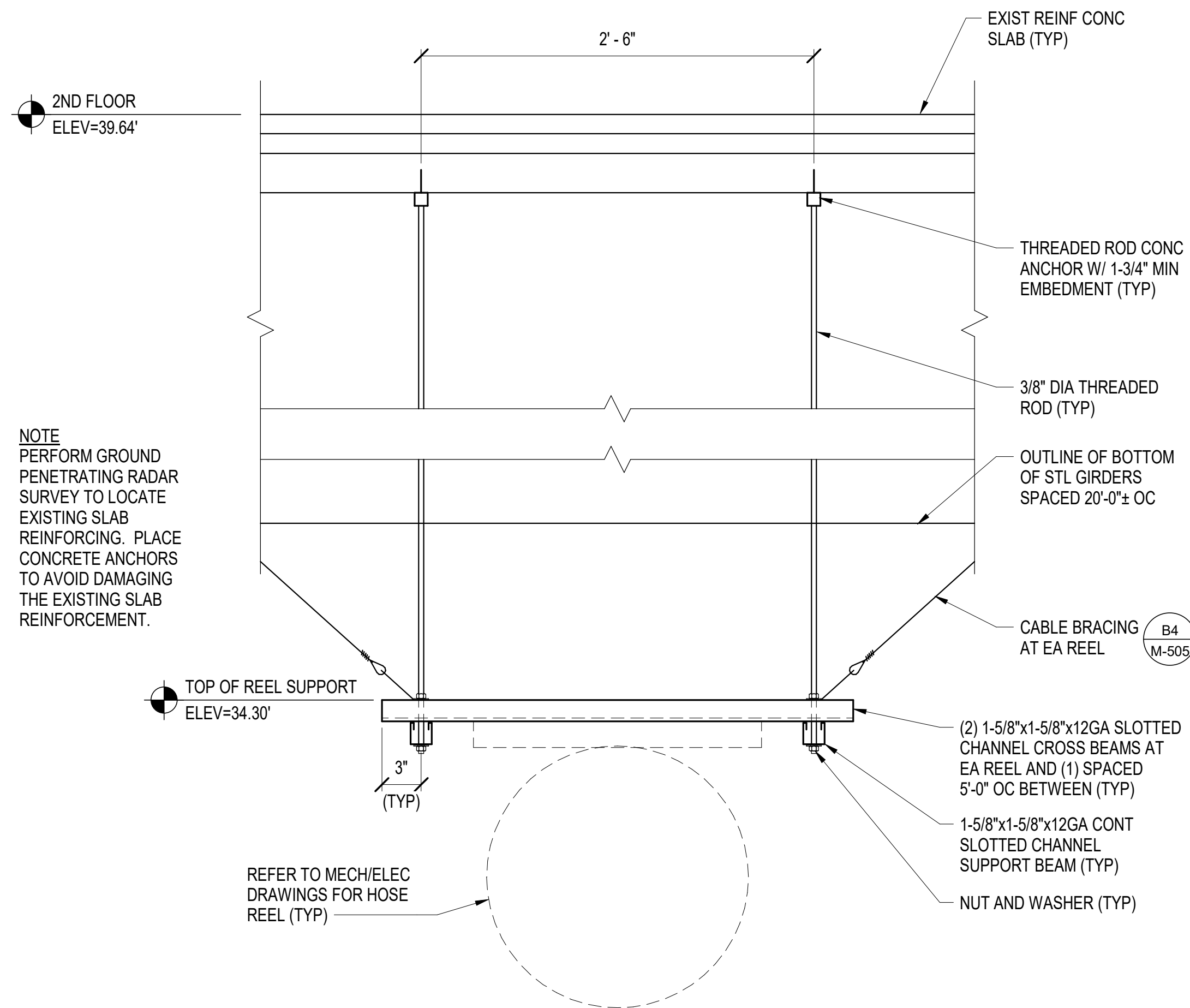
C4 COMPRESSED AIR/ELECTRICAL HOSE REEL SUPPORT DETAIL SCALE: 1 1/2" = 1'-0" (EP104) (SF103)
