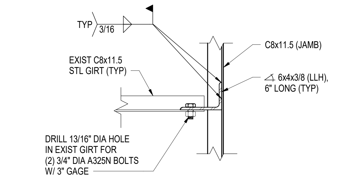
A4 TYP EXIST GIRT TO C8x11.5 DOOR JAMB SCALE: 1 1/2" = 1'-0" (SF503)
