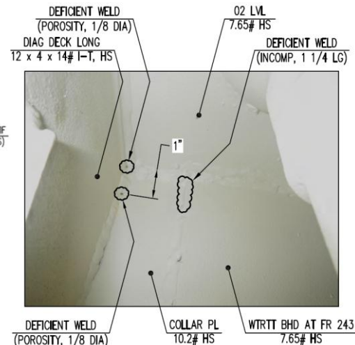
DET 1-B DEFICIENT WELD ON COLLAR PLATE
