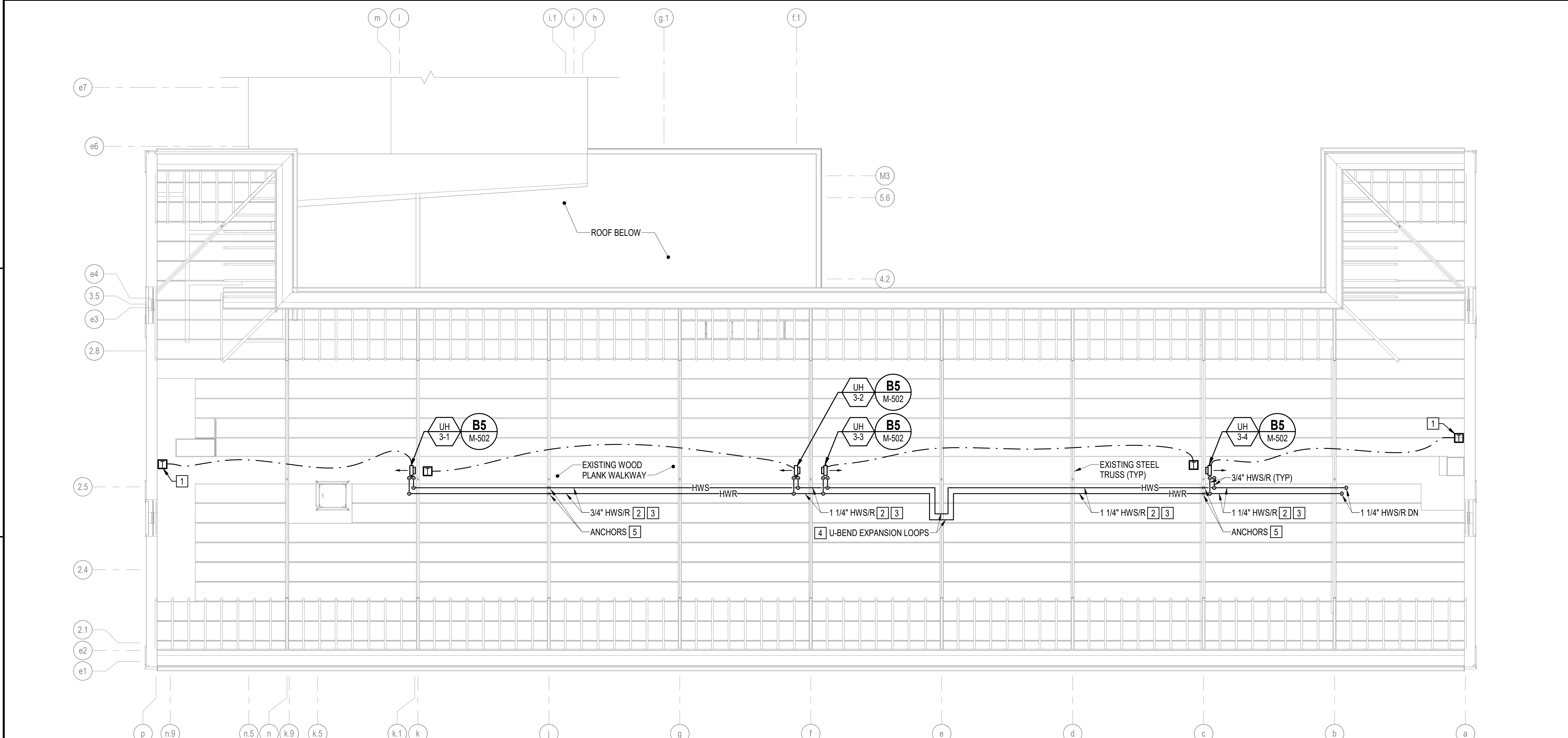
B1 ATTIC MECHANICAL PIPING PLAN - WEST SCALE: 1/8" = 1'-0"
