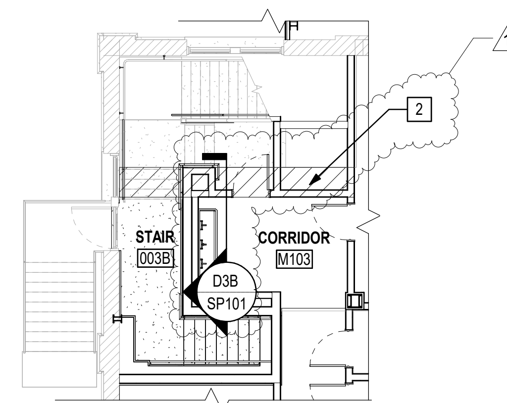
A3 NORTHEAST STAIR FIREPROOFING PLAN SCALE: 1/8" = 1'-0" (90.1 Appendix G 105)
