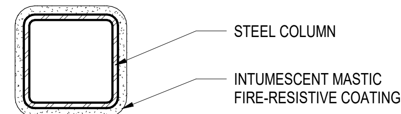
C3 1 HOUR RATED HSS COLUMNS UL X771 SCALE: 3" = 1'-0"
