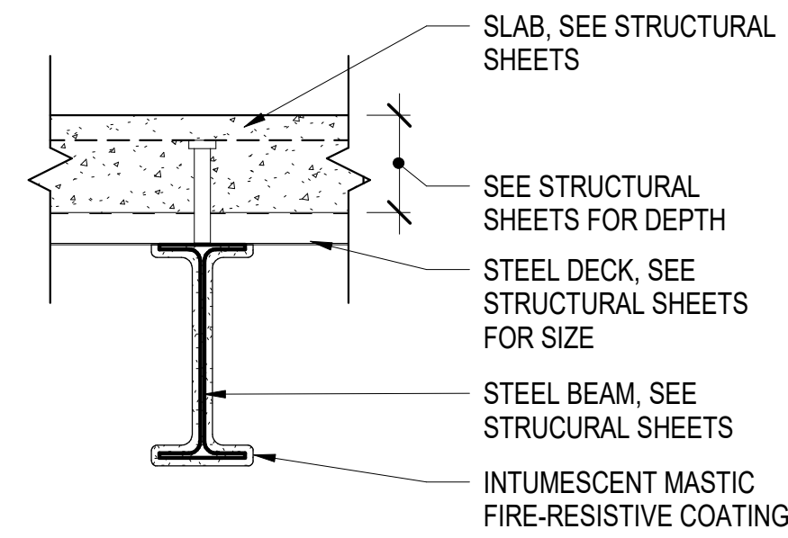
D1 1 HOUR RATED FLOOR ASSEMBLY UL D925 SCALE: 1 1/2" = 1'-0"
