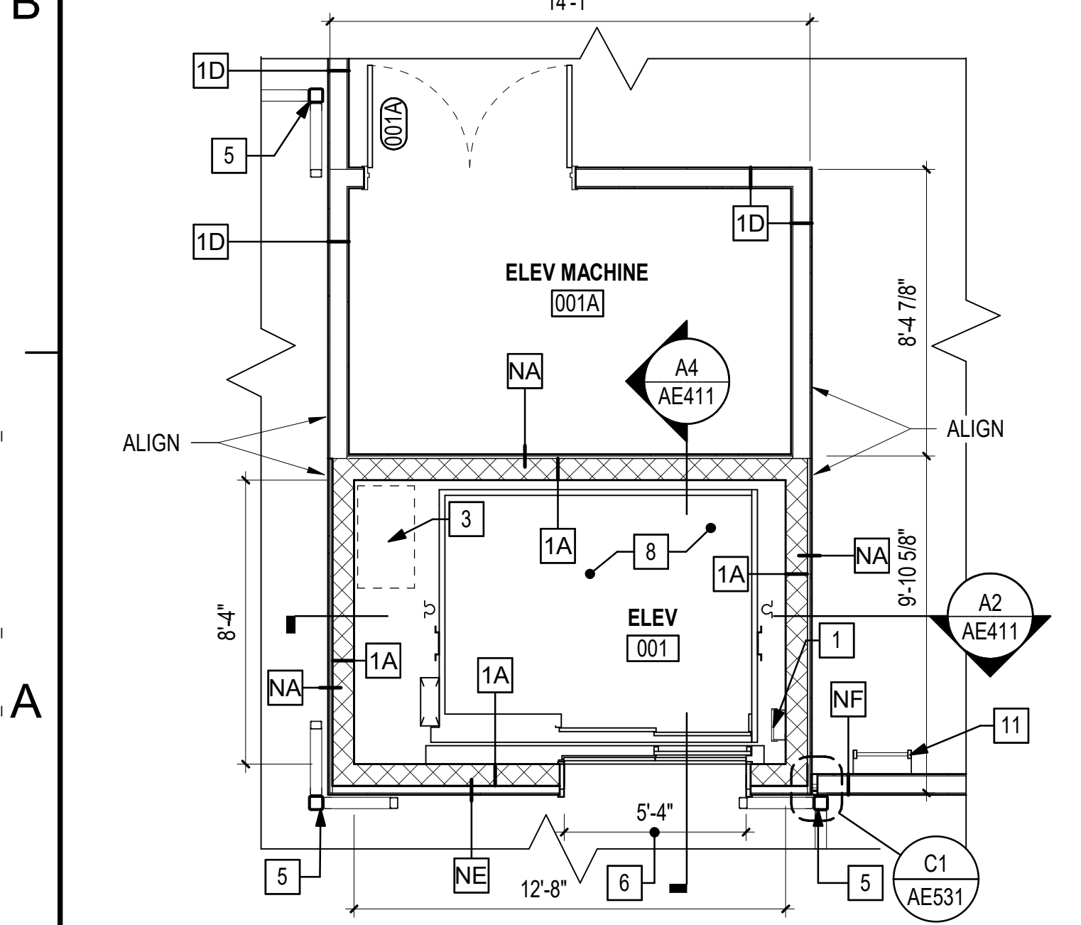
A1 ELEV 001 FIRST FLOOR PLAN SCALE: 1/4" = 1'-0" (AE102)
