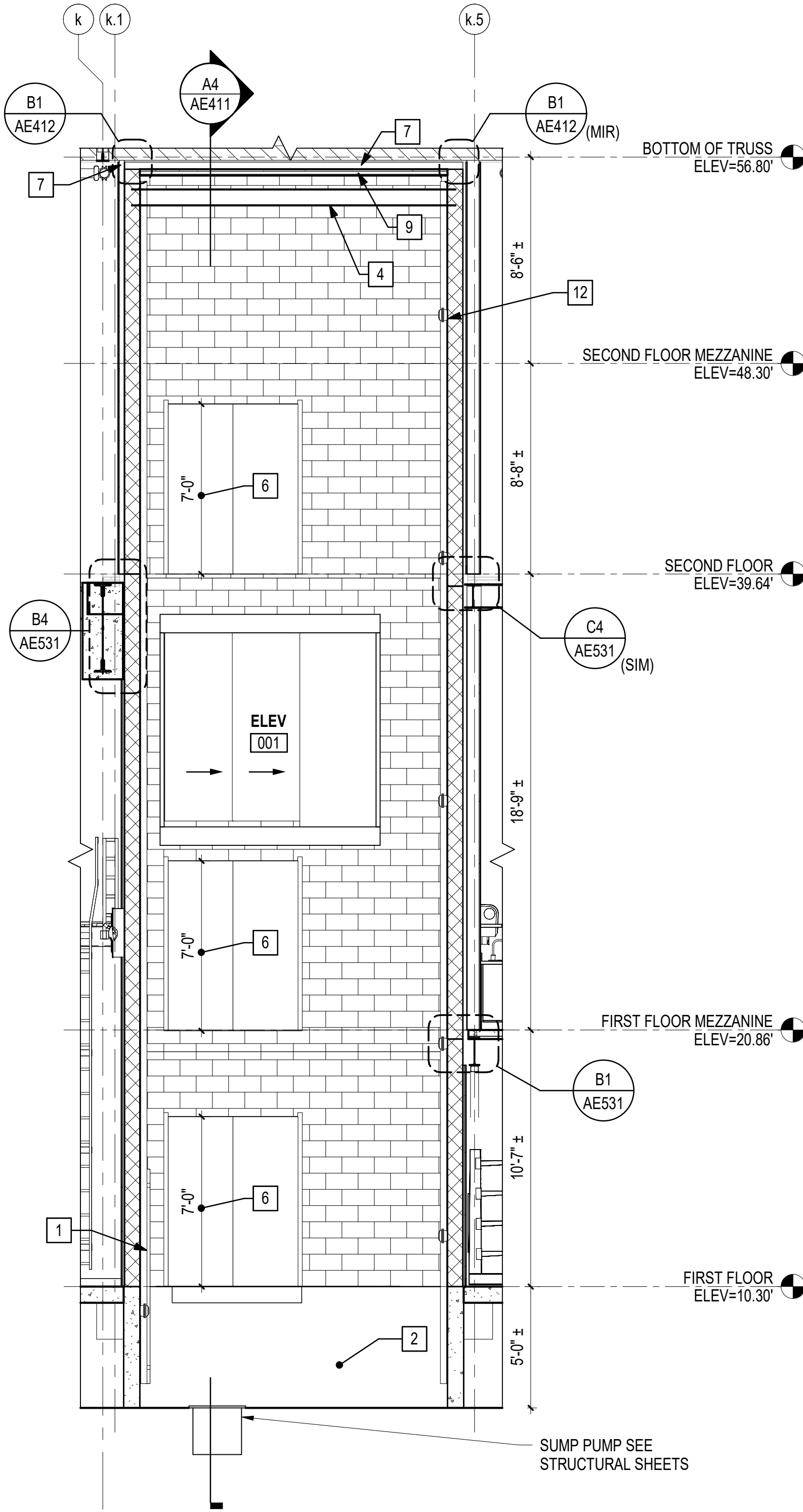
A2 ELEVATOR SECTION 1 SCALE: 1/4" = 1'-0" (AE411)
