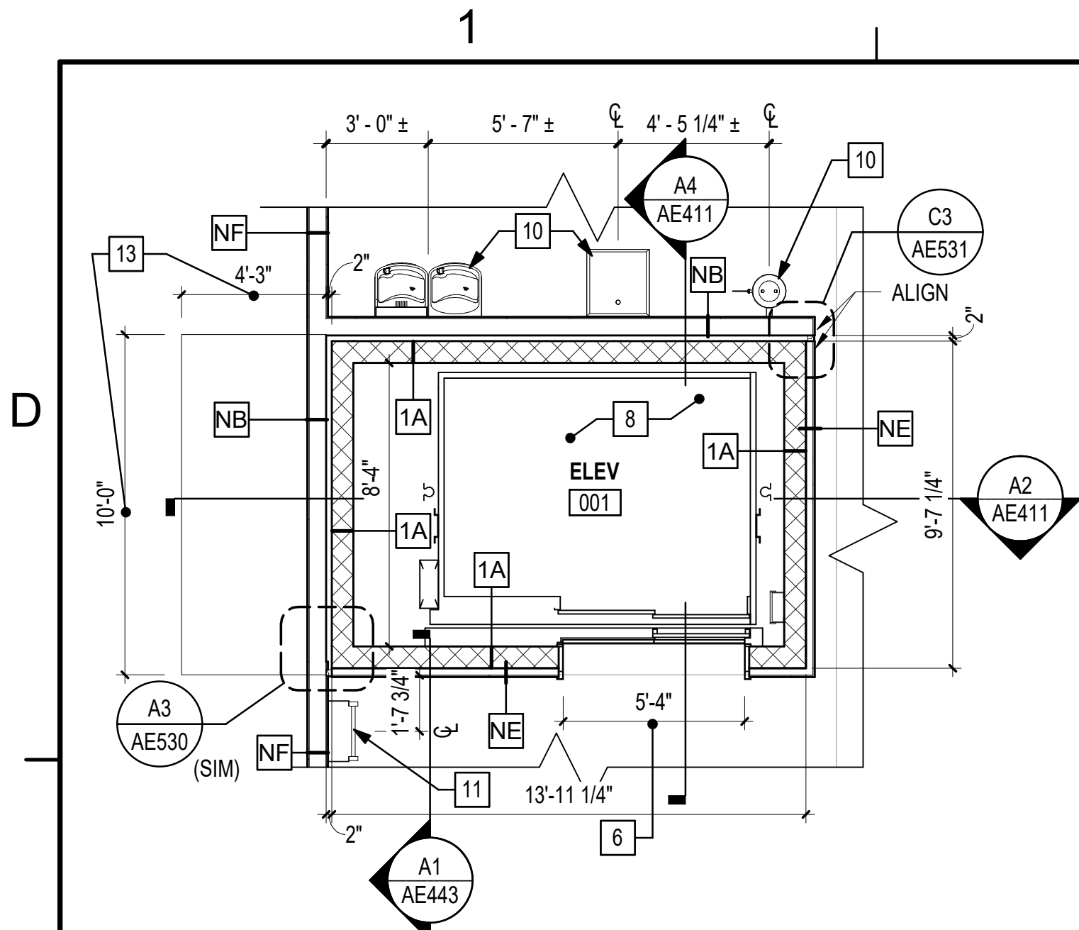
C1 ELEV 001 SECOND FLOOR PLAN SCALE: 1/4" = 1'-0" (AE105)
