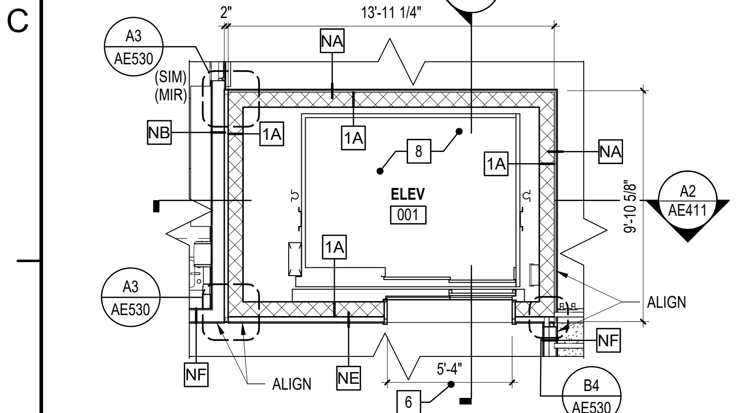
B1 ELEV 001 FIRST FLOOR MEZZANINE PLAN SCALE: 1/4" = 1'-0" (AE104)
