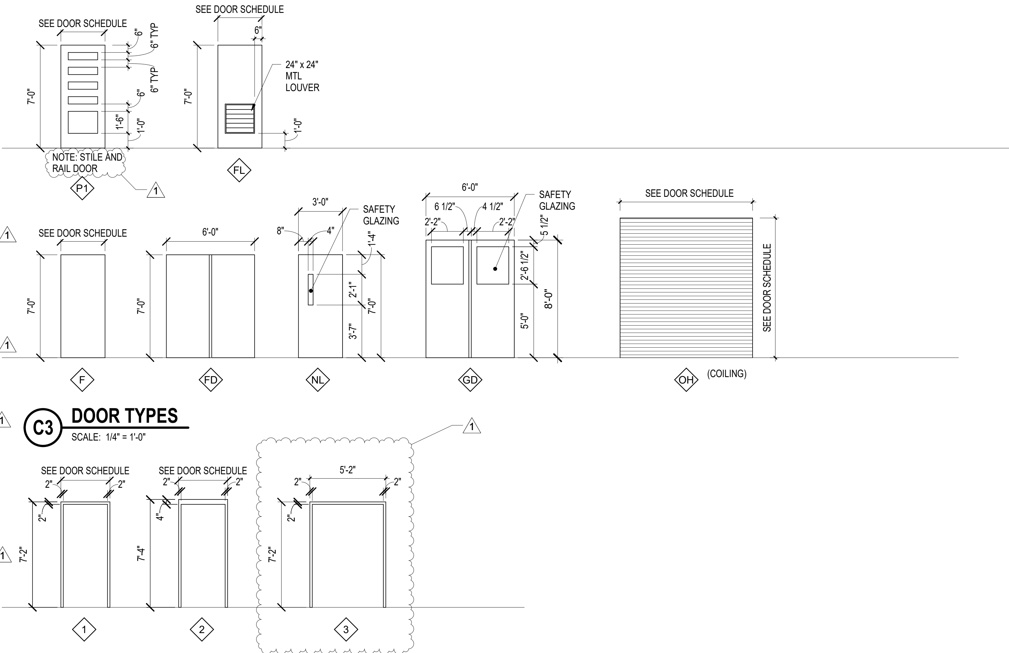
B3 FRAME TYPES SCALE: 1/4" = 1'-0"
