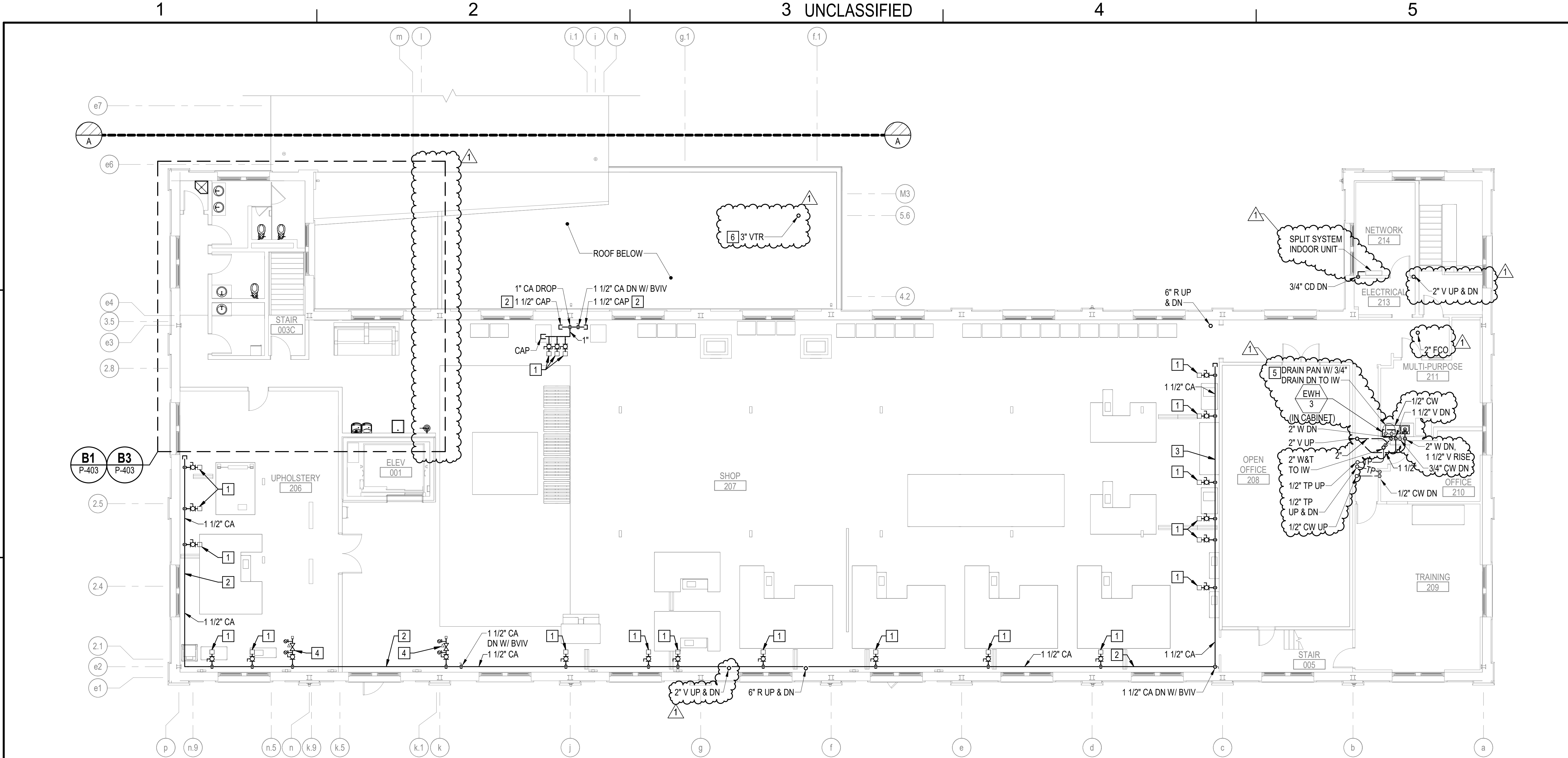
B1 SECOND FLOOR PLUMBING PLAN - WEST SCALE: 1/8" = 1'-0"
