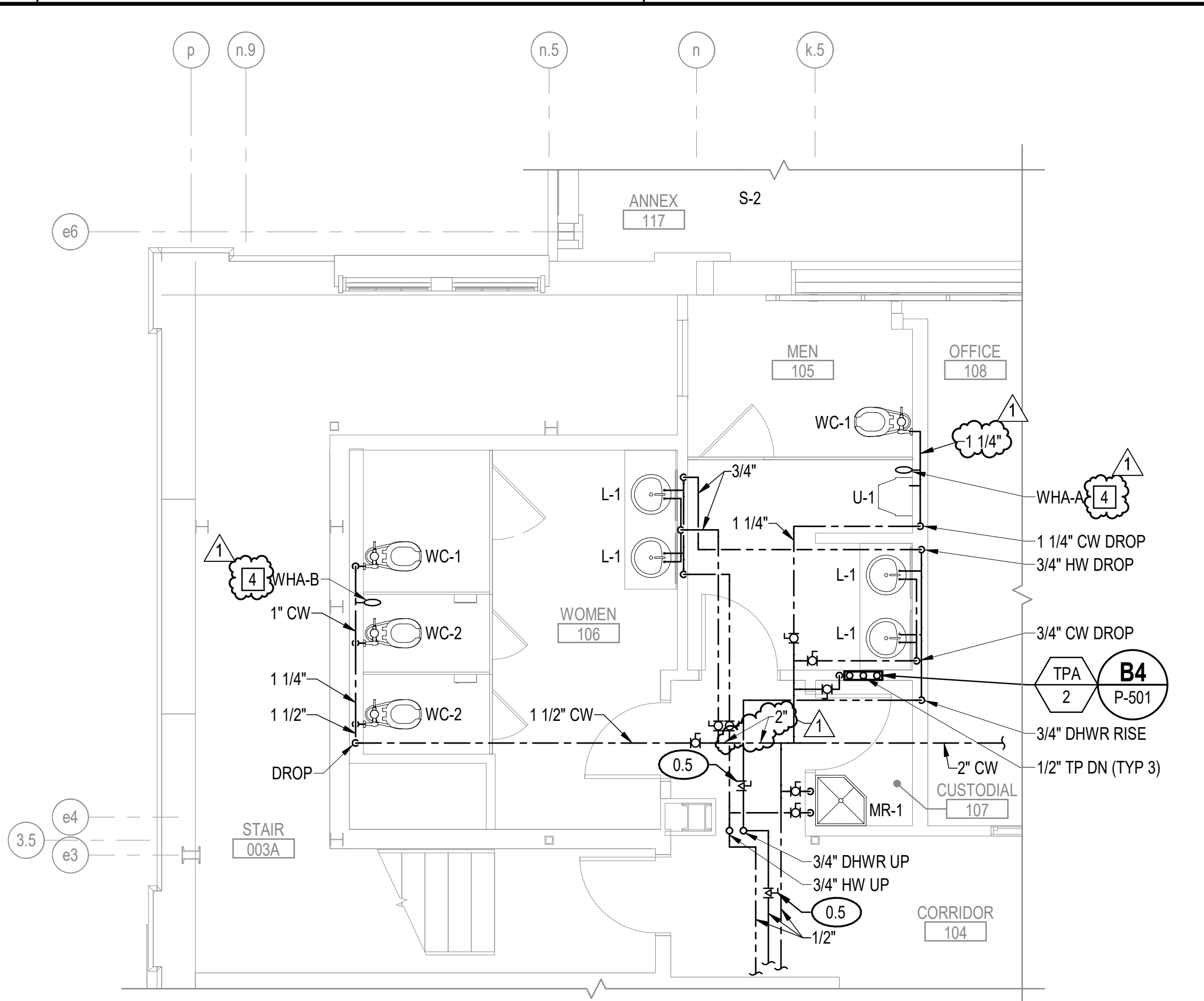
C3 ENLARGED FIRST FLOOR DOMESTIC WATER SUPPLY PART PLAN SCALE: 1/4" = 1'-0" (P-104)
