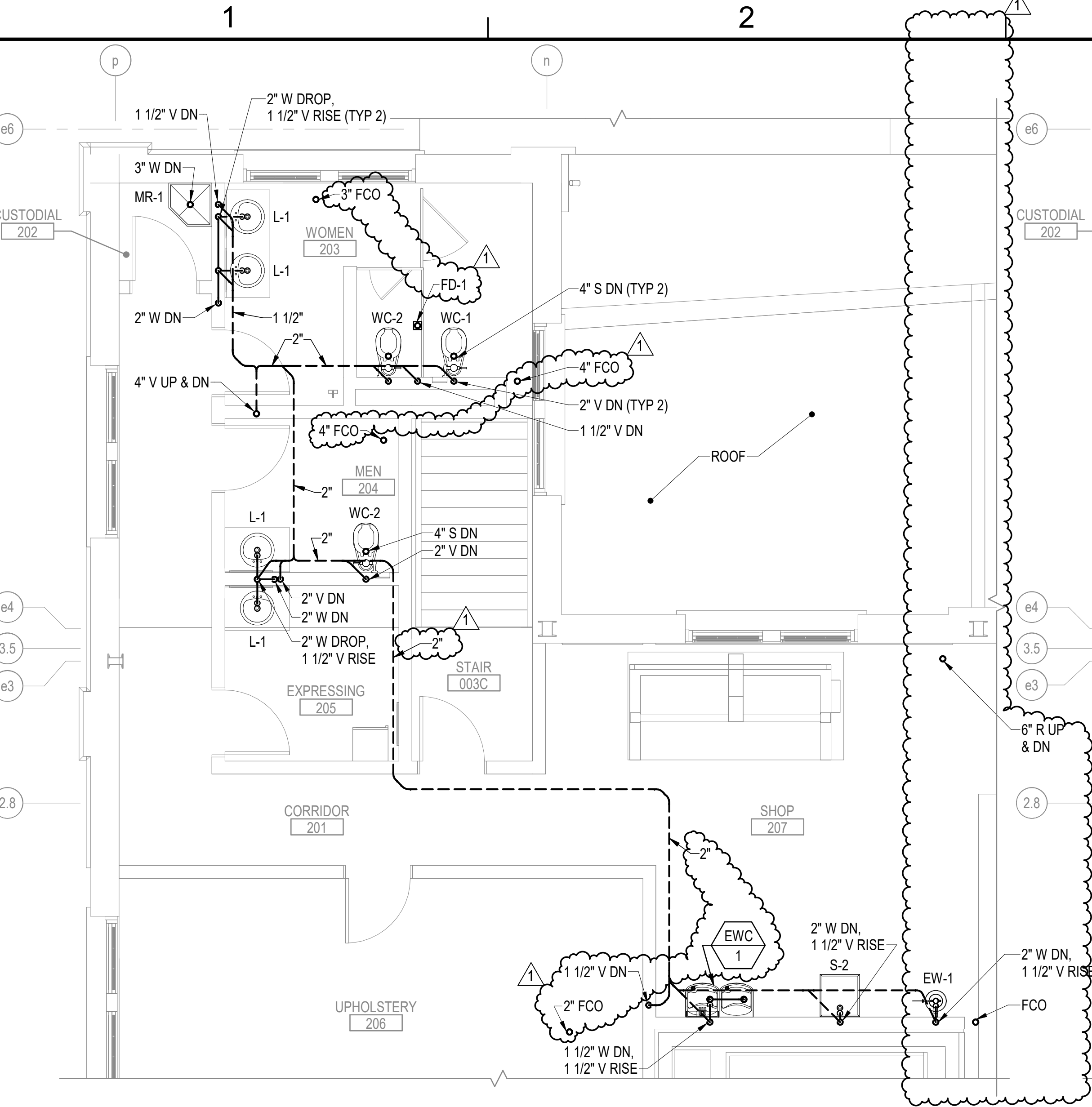
B1 ENLARGED SECOND FLOOR SANITARY WASTE AND VENT PART PLAN SCALE: 1/4" = 1'-0" (P-107)
