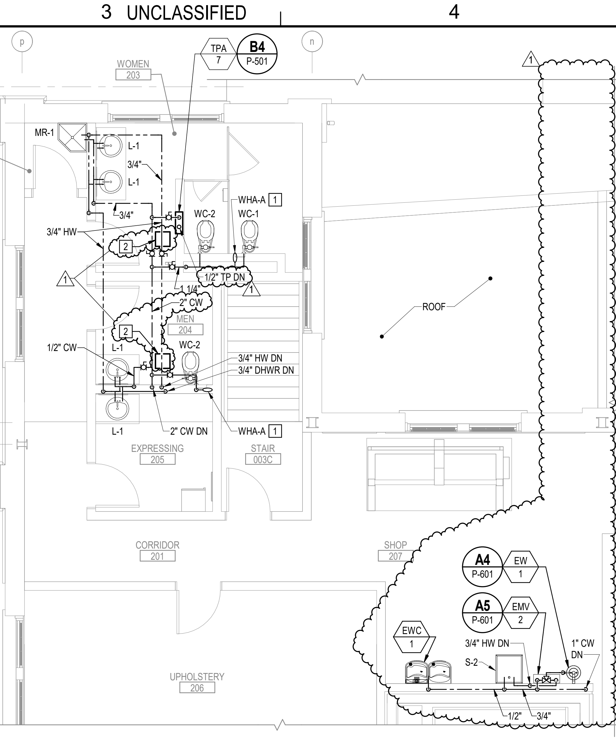
B3 ENLARGED SECOND FLOOR DOMESTIC WATER SUPPLY PART PLAN SCALE: 1/4" = 1'-0" (P-107)
