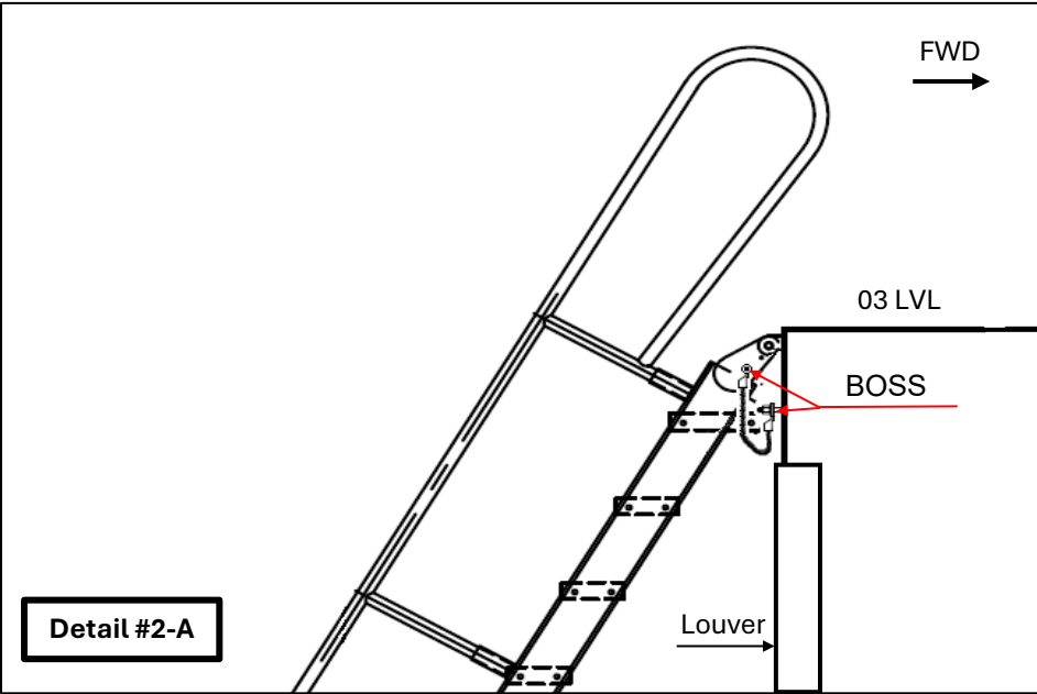
TOP SIDE INCLINED LADDER
