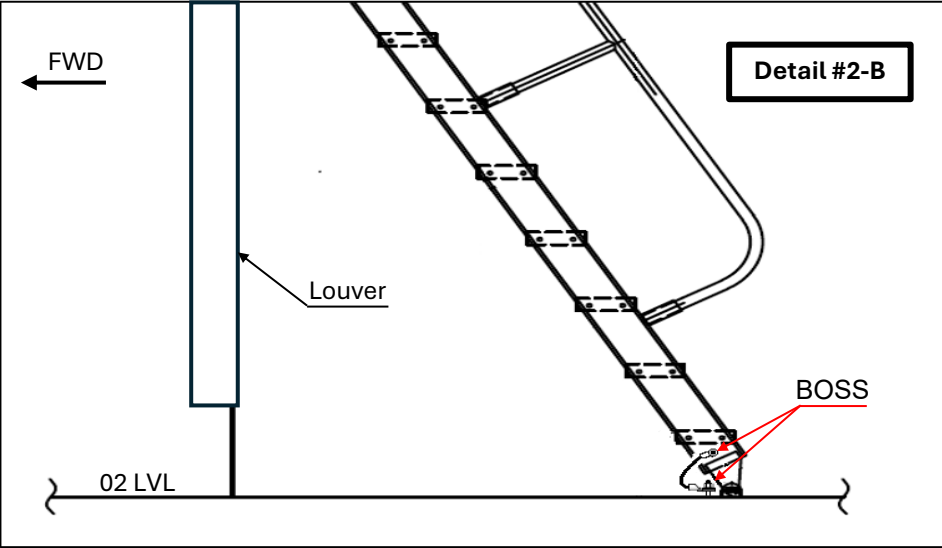
BOTTOM SIDE INCLINED LADDER
