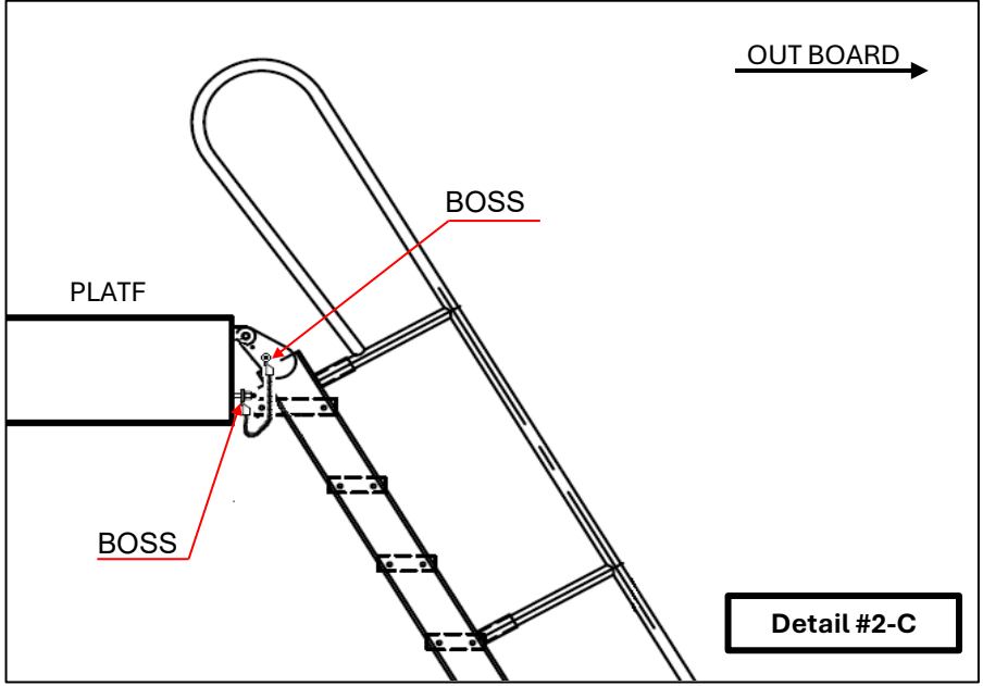
TOP SIDE INCLINED LADDER
