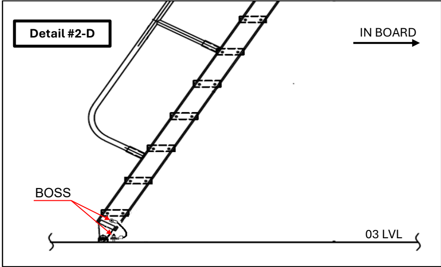
BOTTOM SIDE INCLINED LADDER
