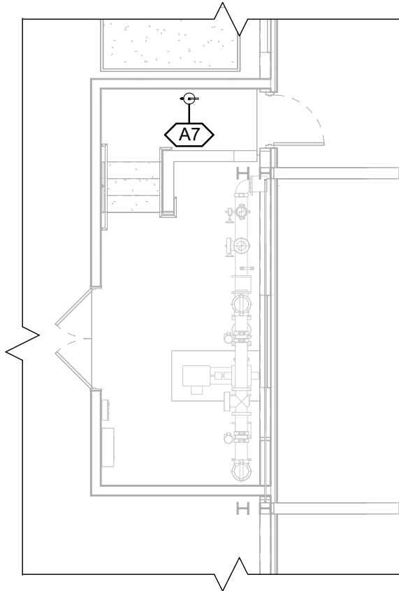
B4 FIRST FLOOR MEZZANINE FIRE PUMP ROOM FF&E PART PLAN SCALE: 1/8" = 1'-0" (90.1 Appendix G 105)
