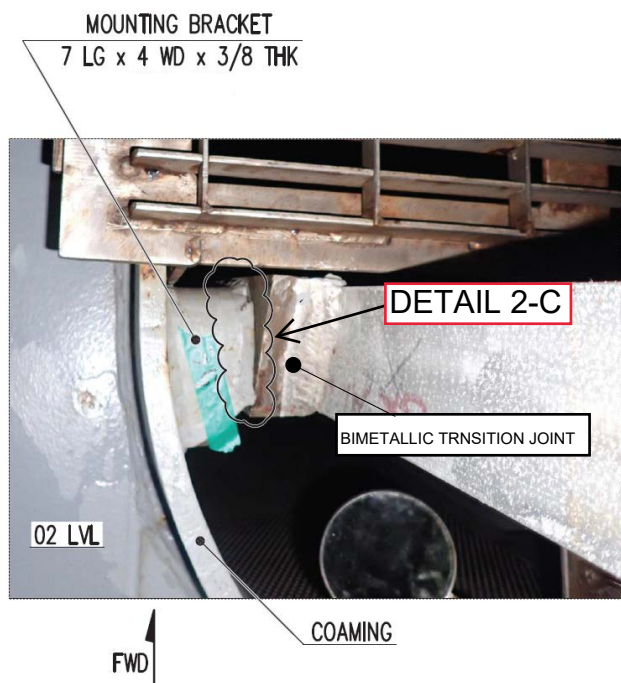
PLAN 2-B BIMETALLIC TRANSITION JOINT 02 LEVEL, STBD
