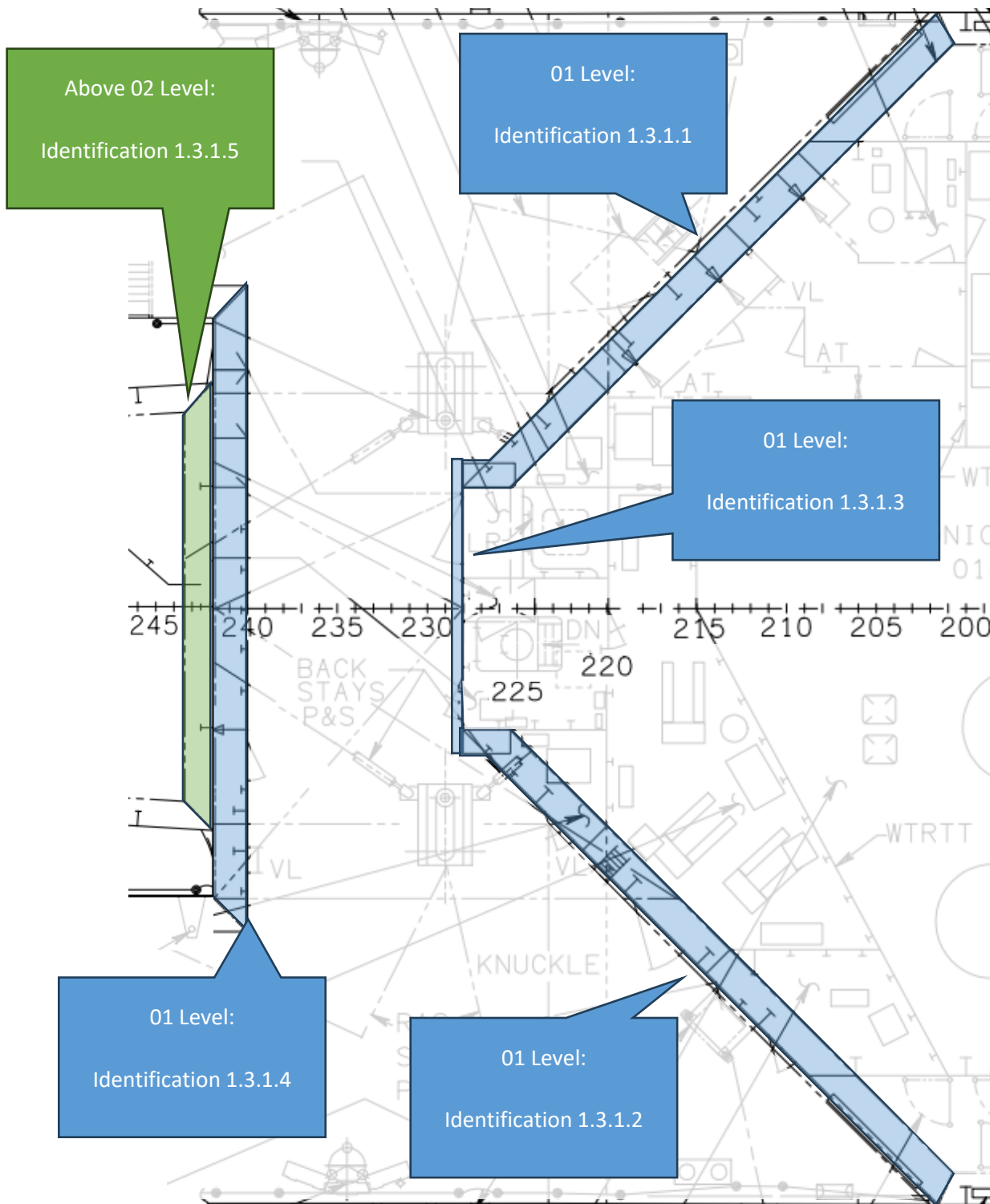
PLAN VIEW 01 Level and 02 Level Weather Frames Between 200 and 242
