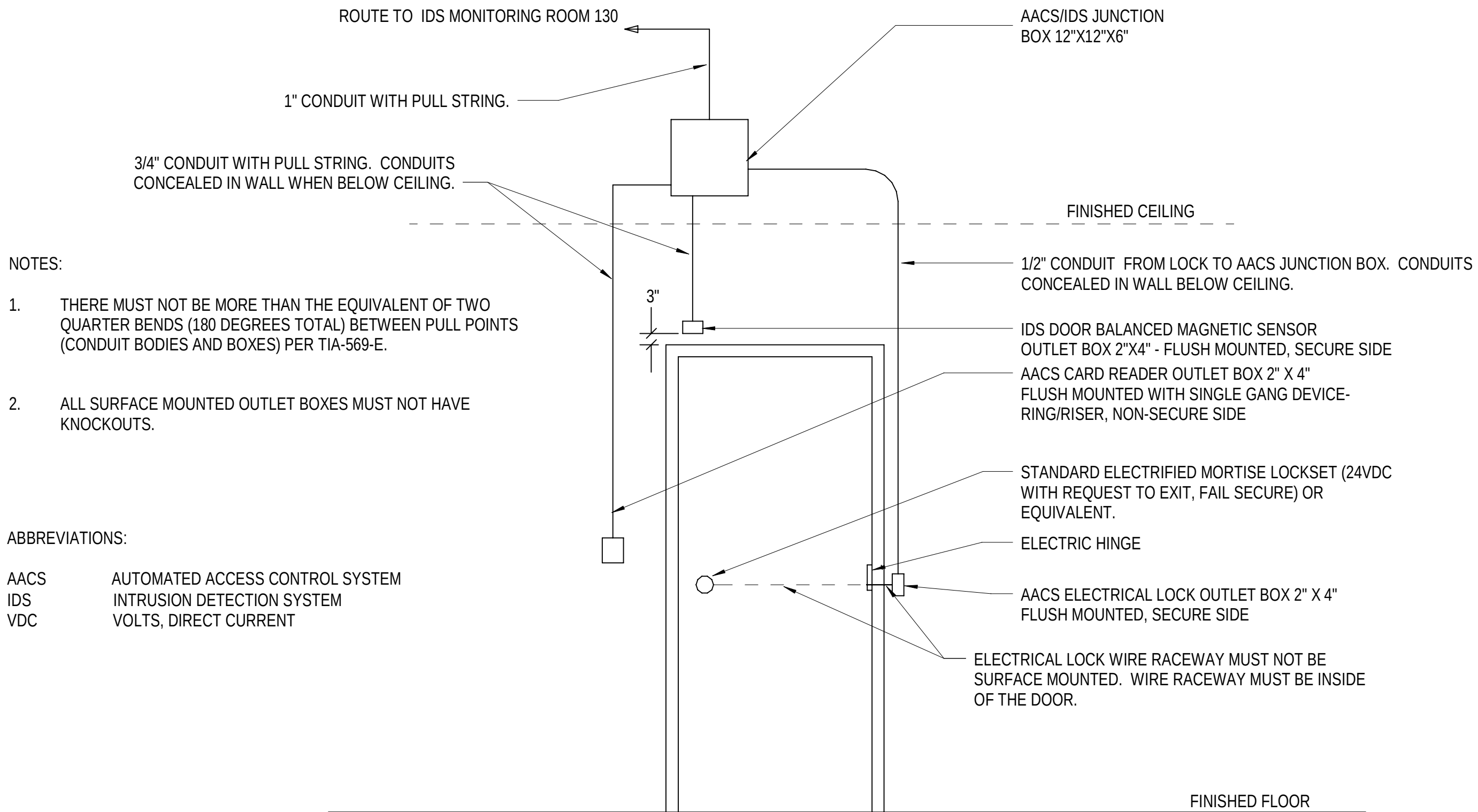
A1 SECURED SINGLE DOOR W/ CARD READER NOT TO SCALE
