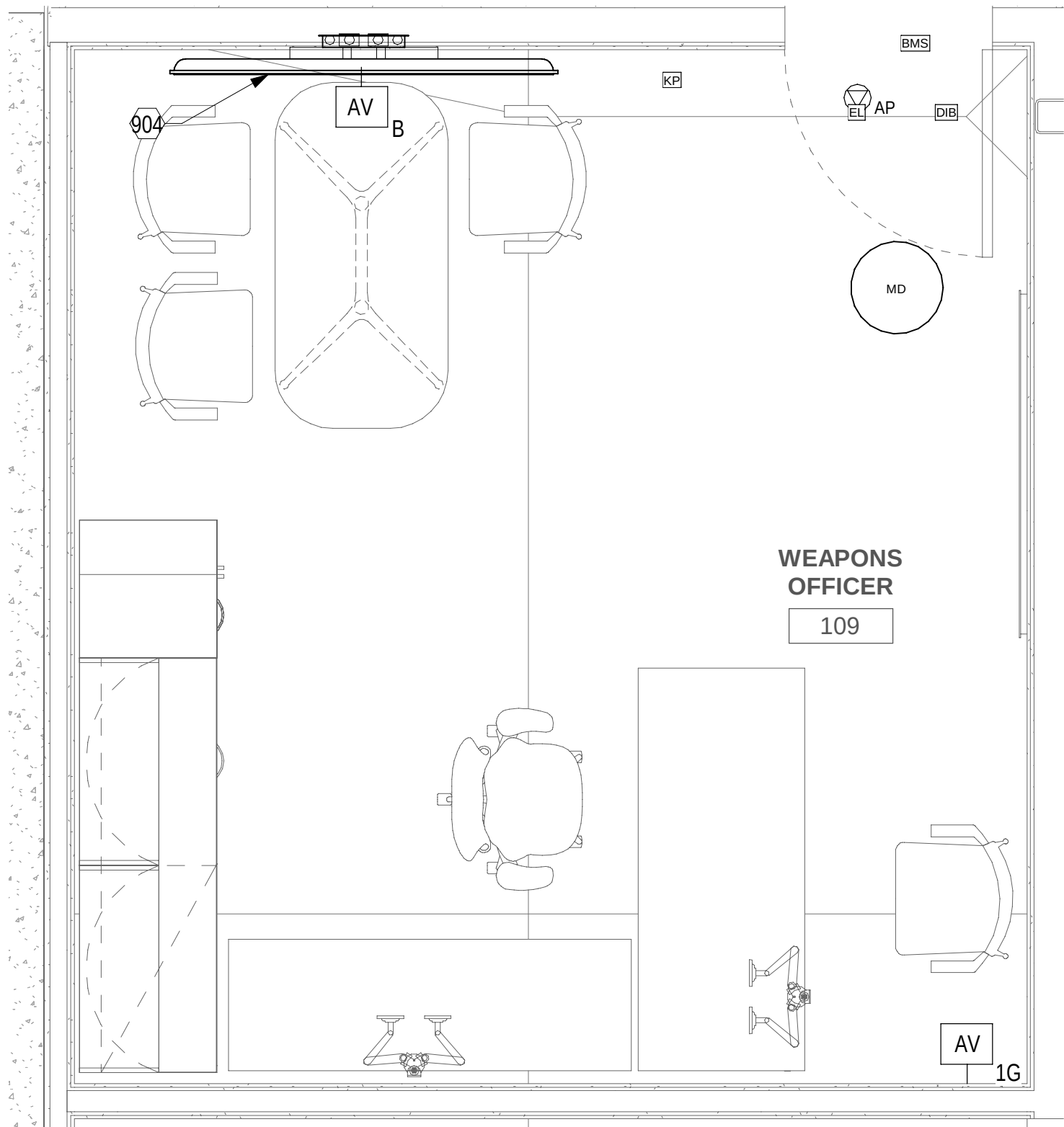
A3 AUDIO VISUAL ENLARGED PLAN - ROOM 109 1/2" = 1'-0" (TA101)
