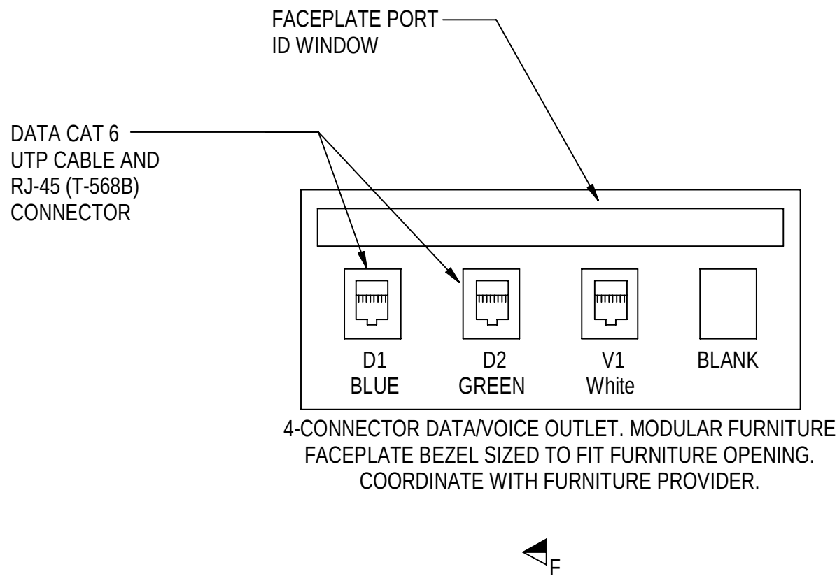
D2 MODULAR FURNITURE AND VOICE OUTLET NTS
