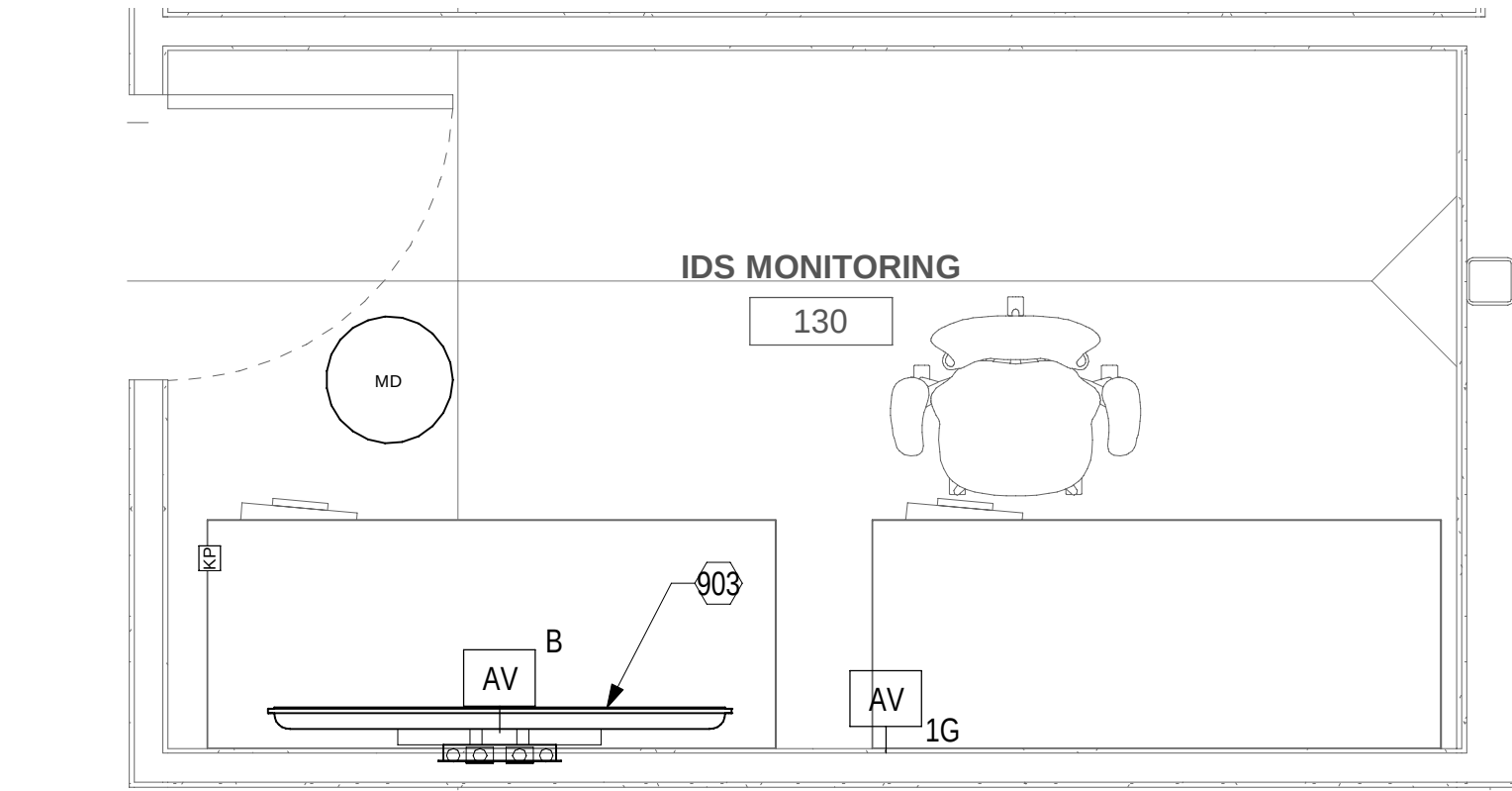
C3 AUDIO VISUAL ENLARGED PLAN - IDS MONITORING 1/2" = 1'-0" (TA101)
