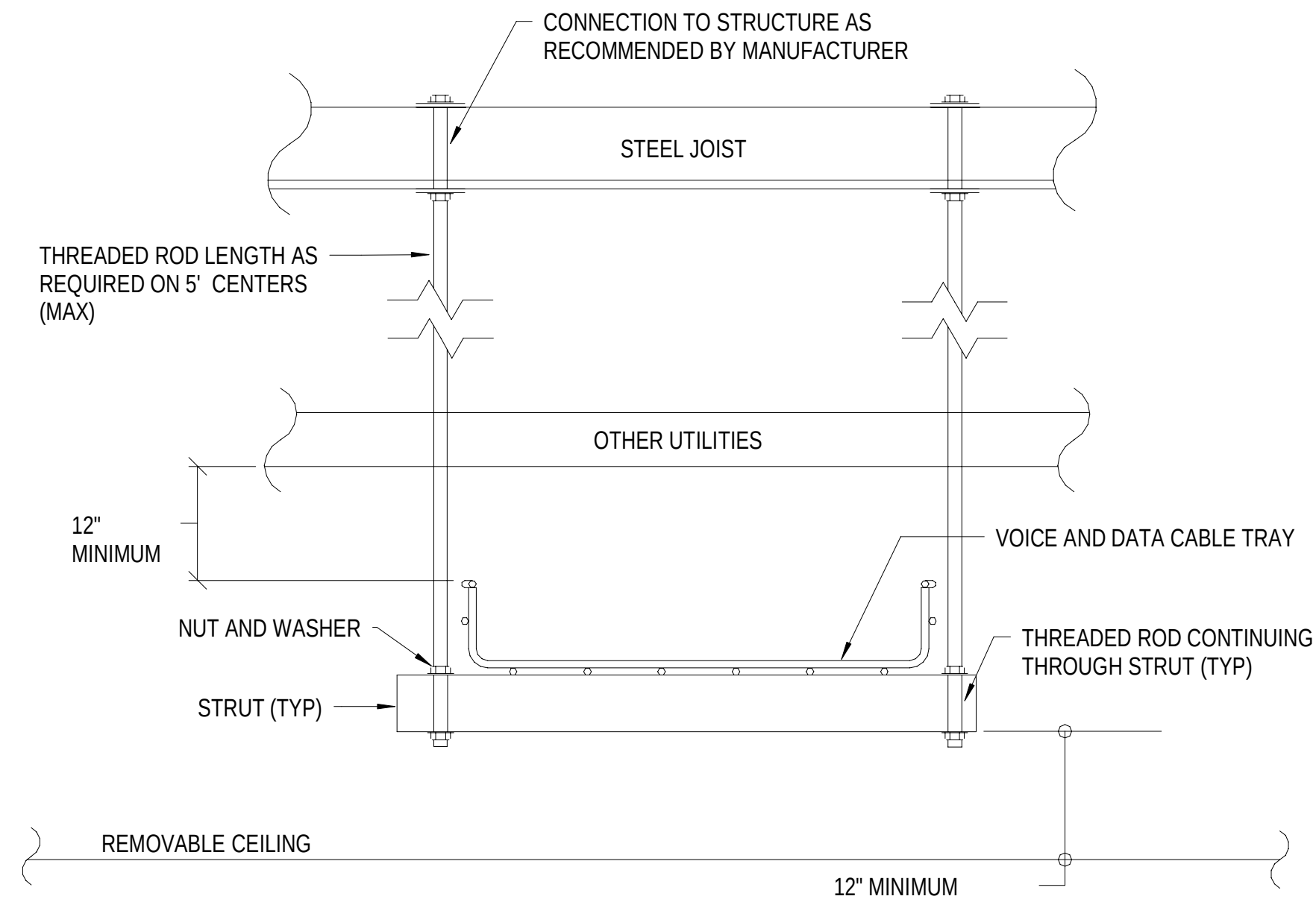
ABOVE CEILING MOUNTED CABLE TRAY
