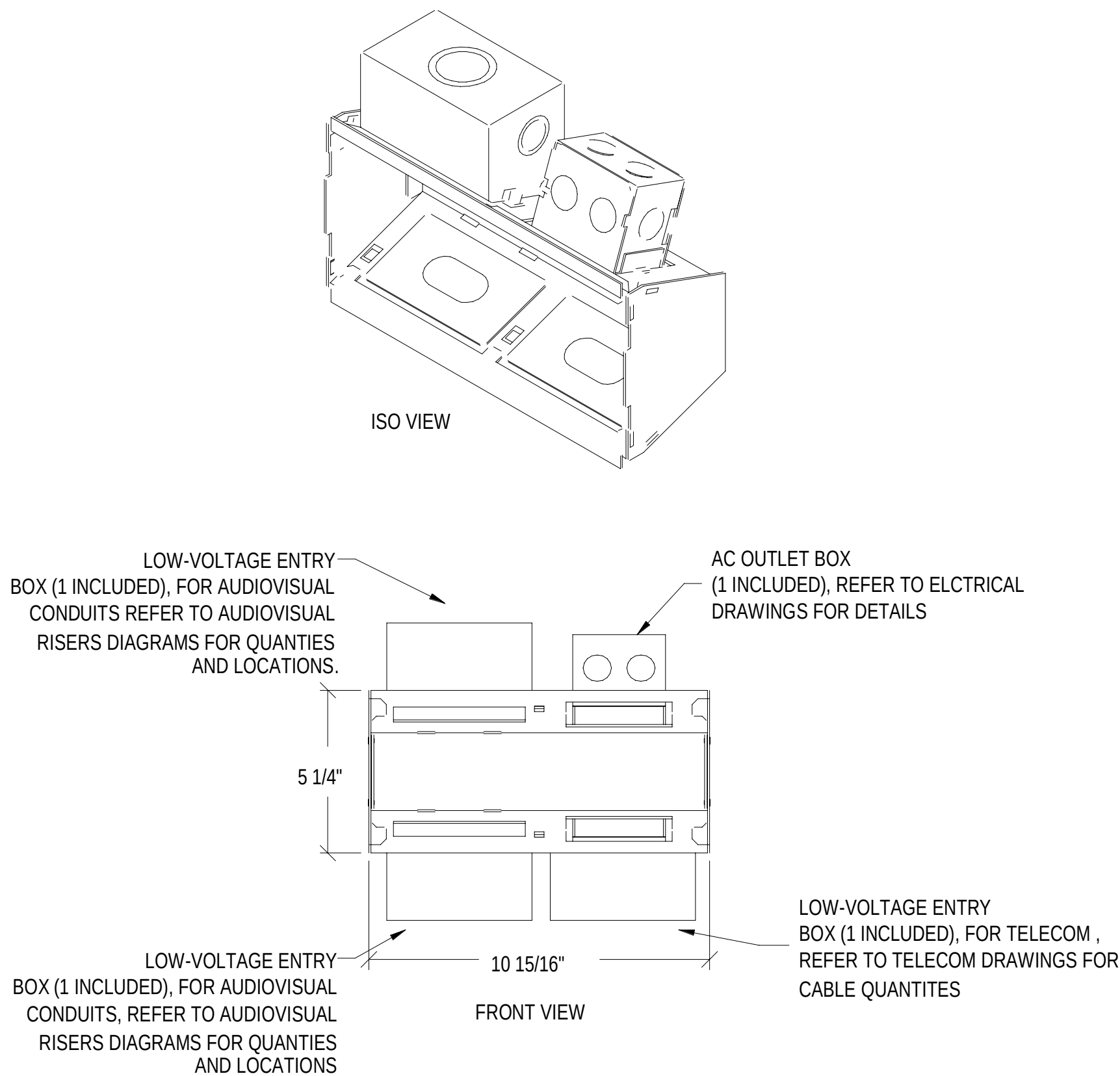
A3 PWB-100 DETAIL NTS
