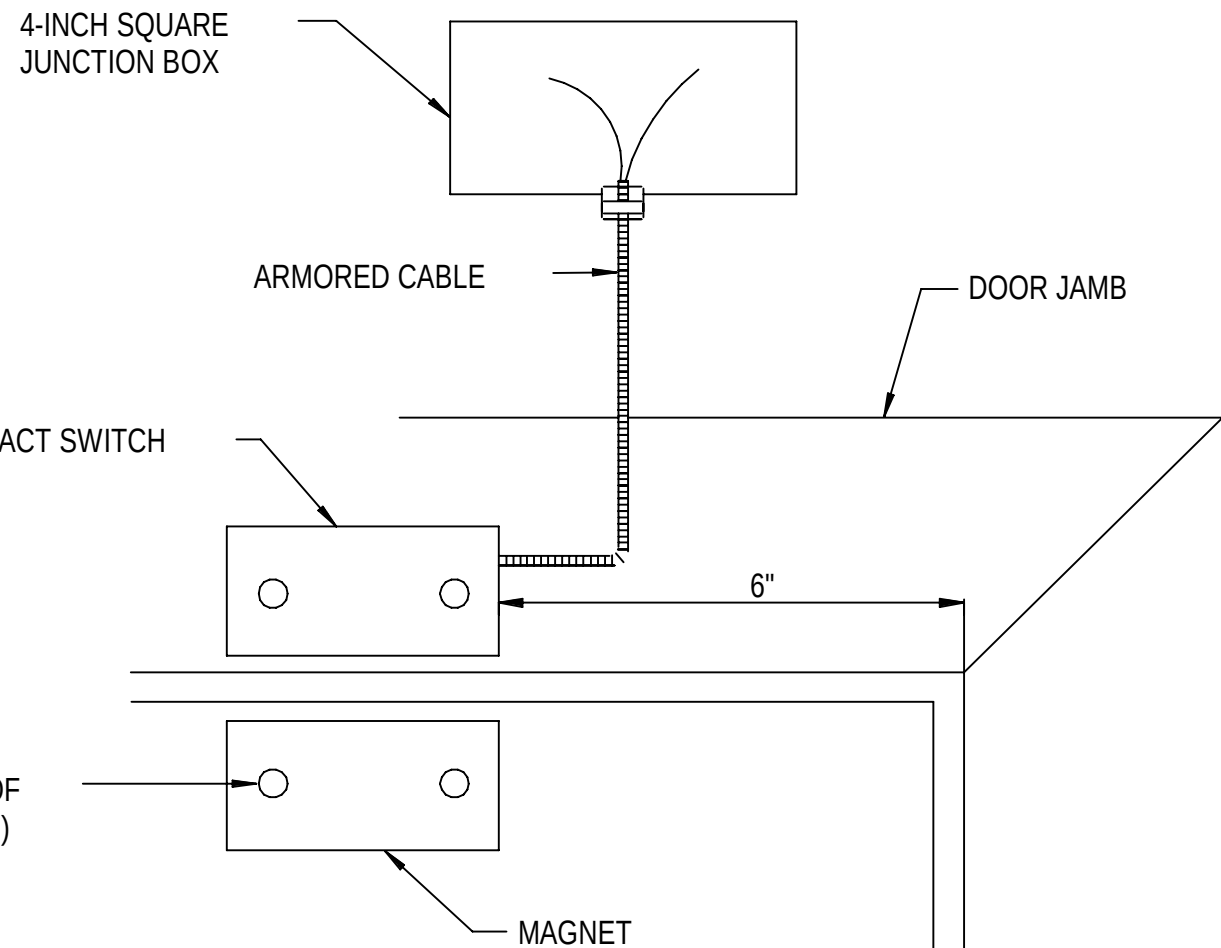
A3 SCREW MOUNT DOOR CONTACT NTS
