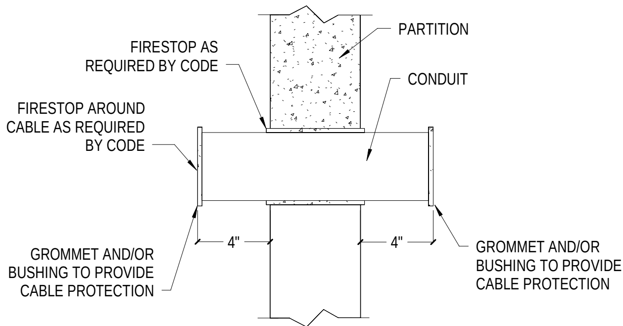
C1 TYPICAL SLEEVE IN RATED WALL NTS
