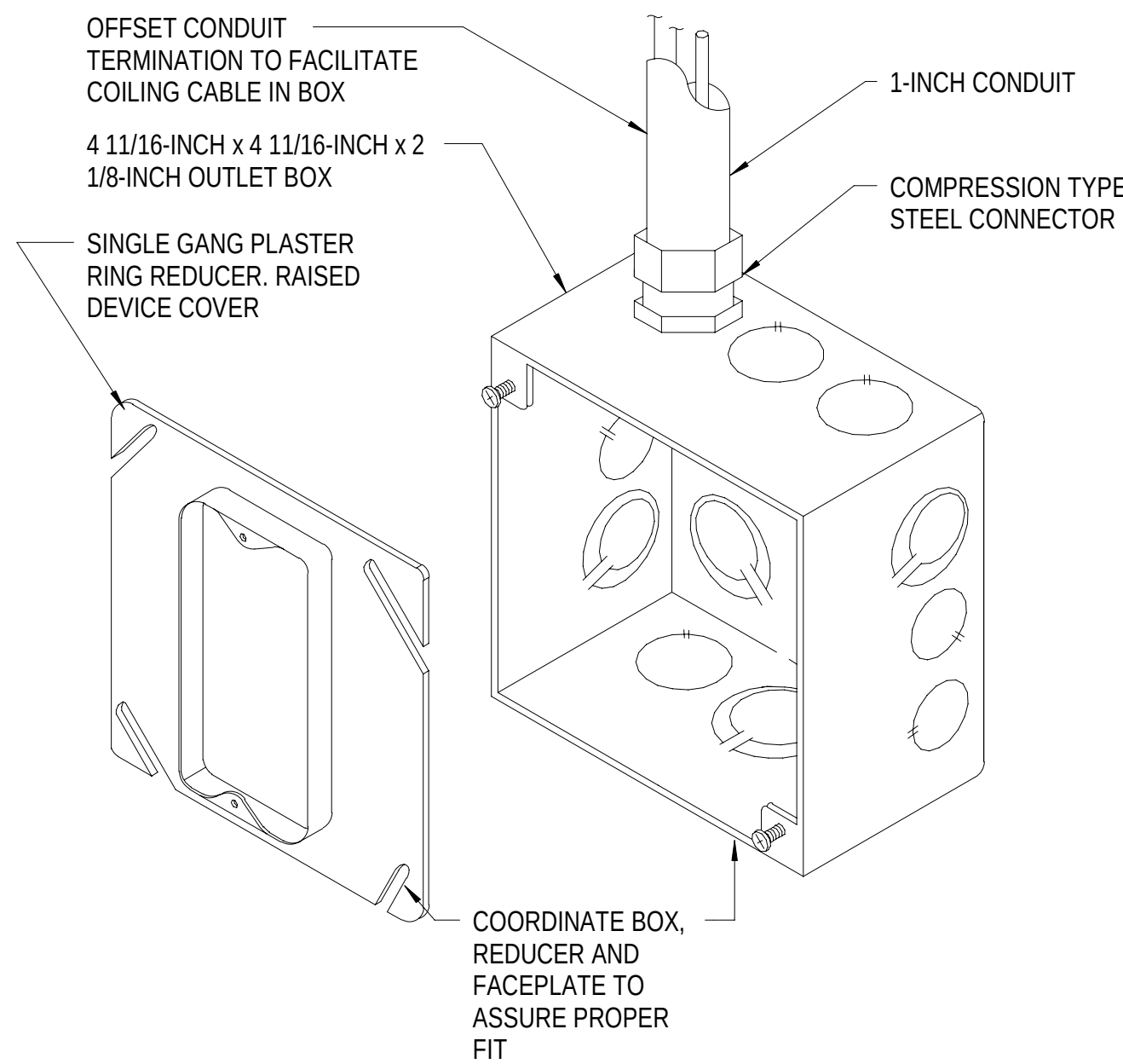
A1 WALL MOUNTED OUTLET BOX DETAIL NTS
