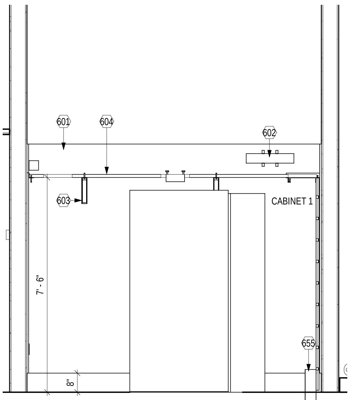
A1 TELECOM 105 EAST ELEVATION 1/2" = 1'-0" (T-102)
