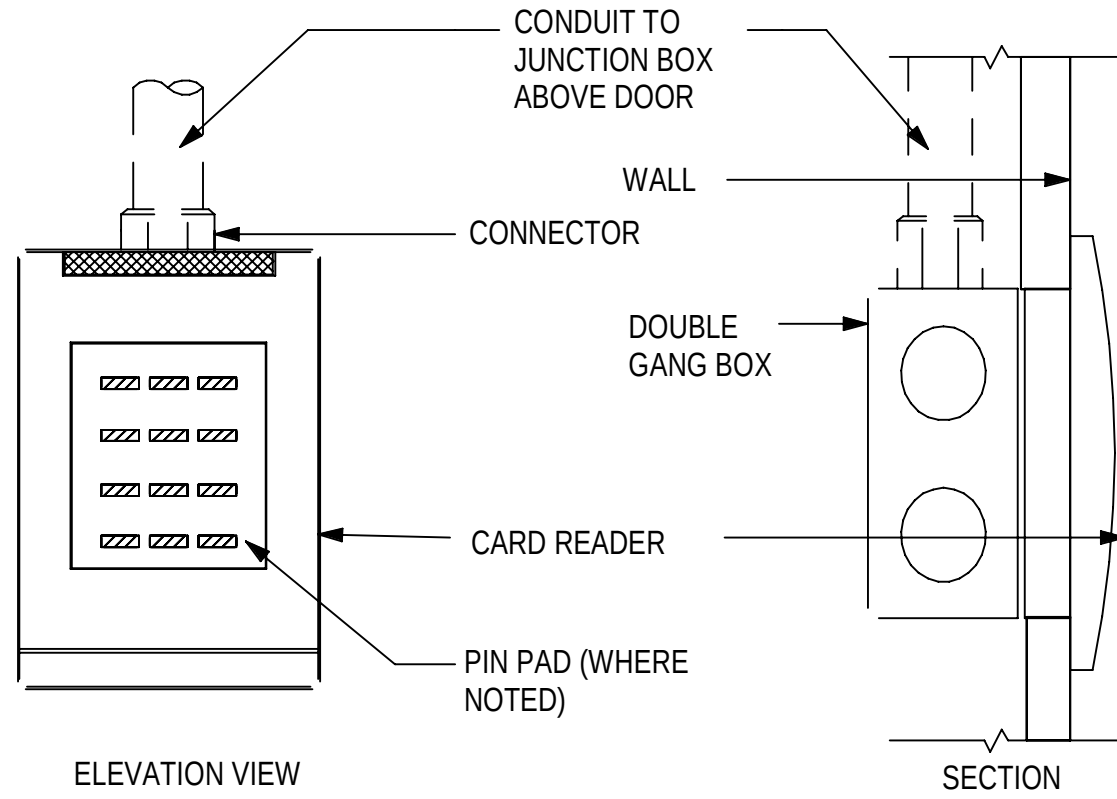
C3 CARD READER W/ PIN PAD NTS
