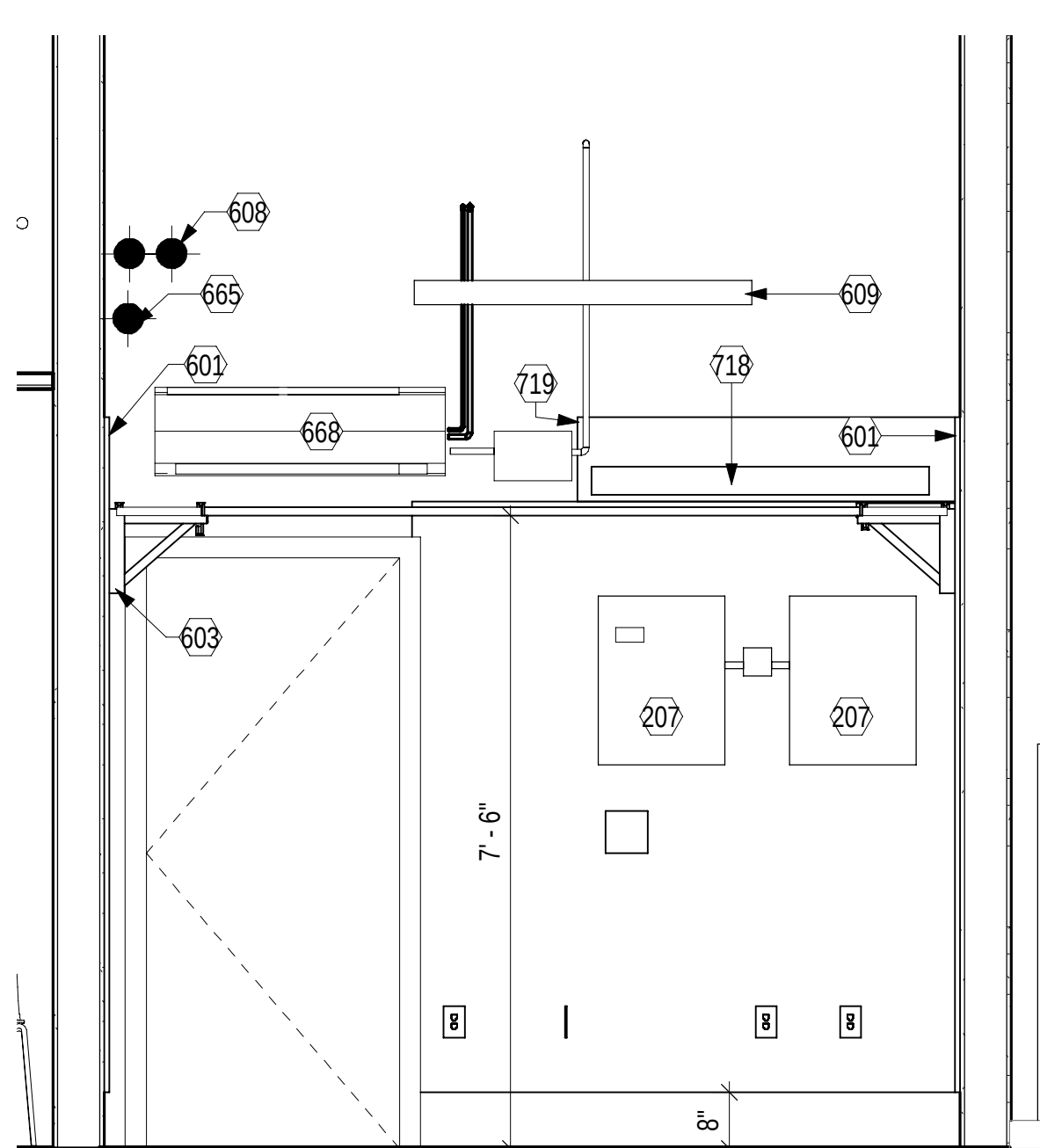
C3 TELECOM 105 - NORTH ELEVATION 1/2" = 1'-0" (T-102)
