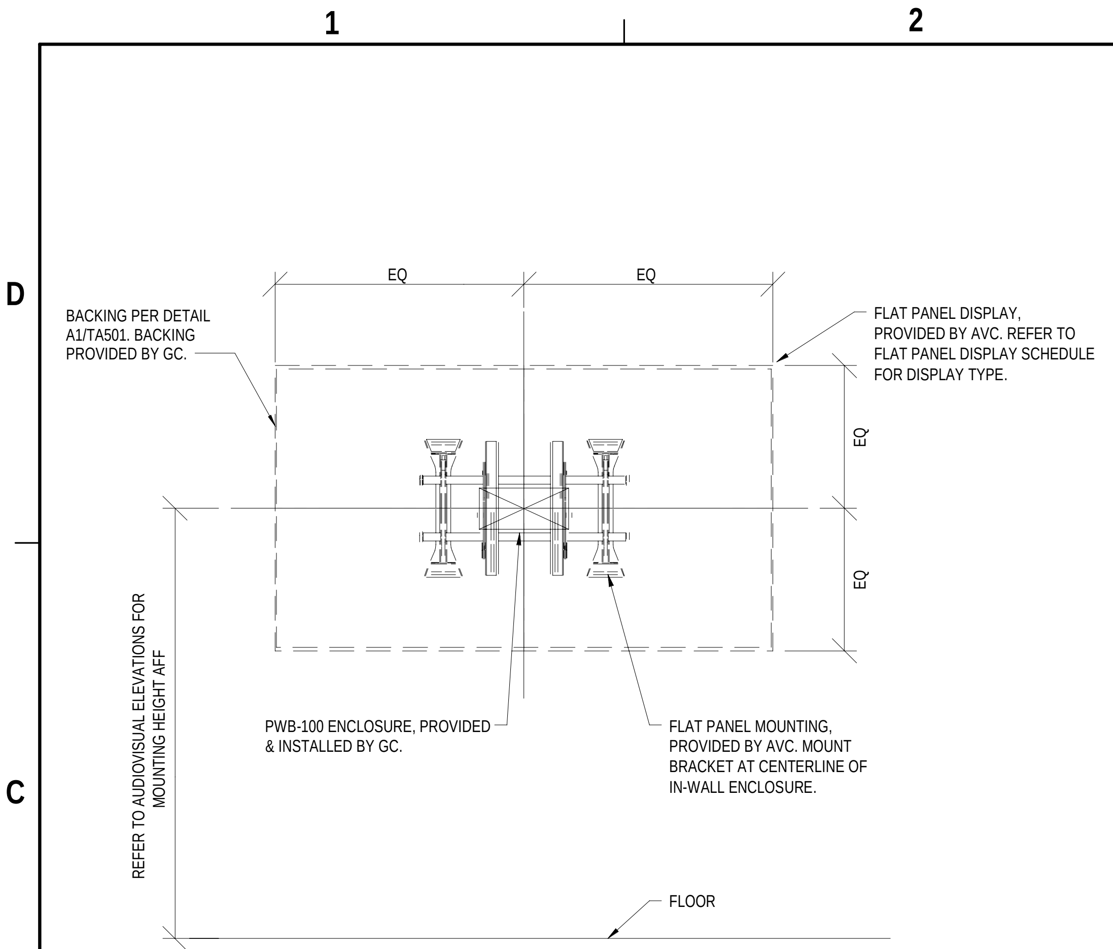
C1 FLAT PANEL DISPLAY BRACKET DETAIL NTS
