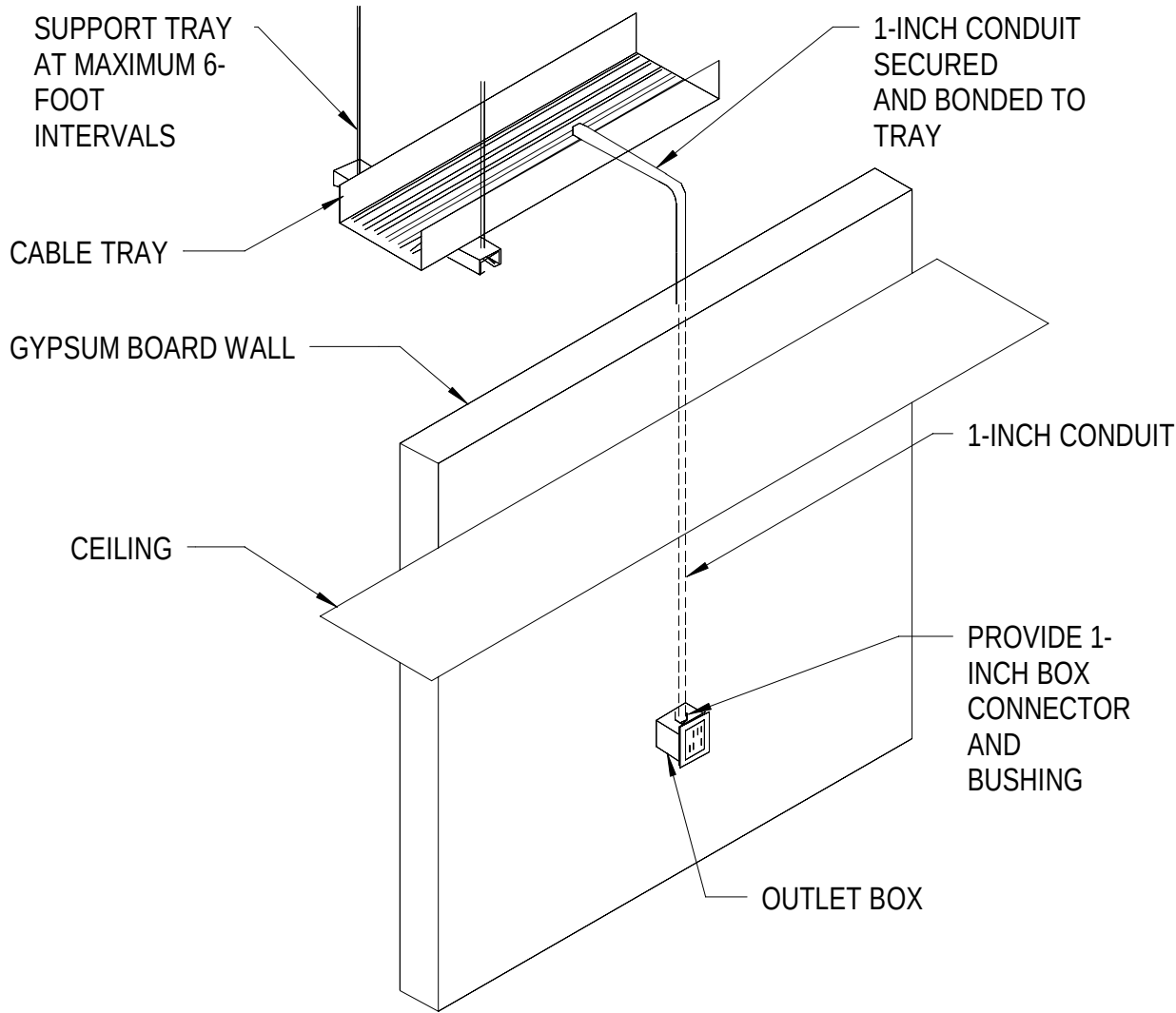
A2 TYPICAL OUTLET DROP NTS
