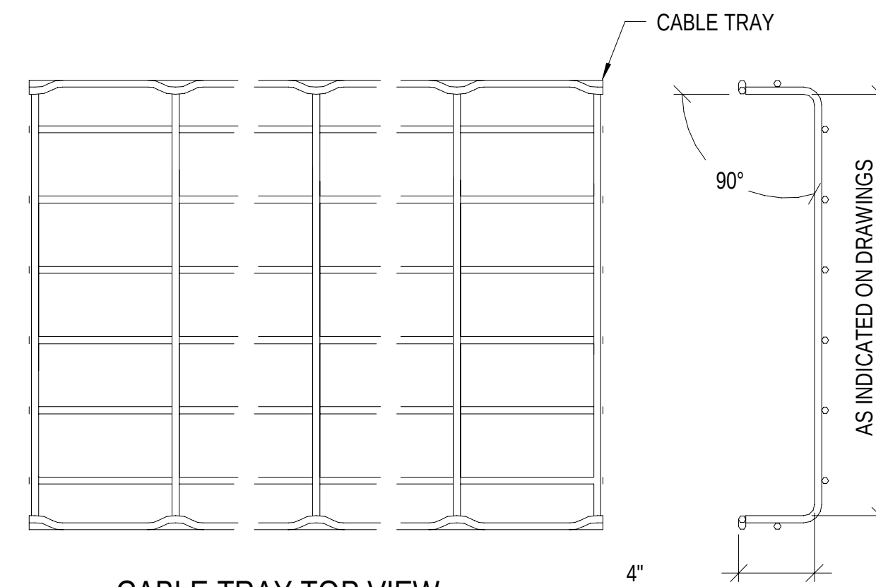
CABLE TRAY TOP VIEW
