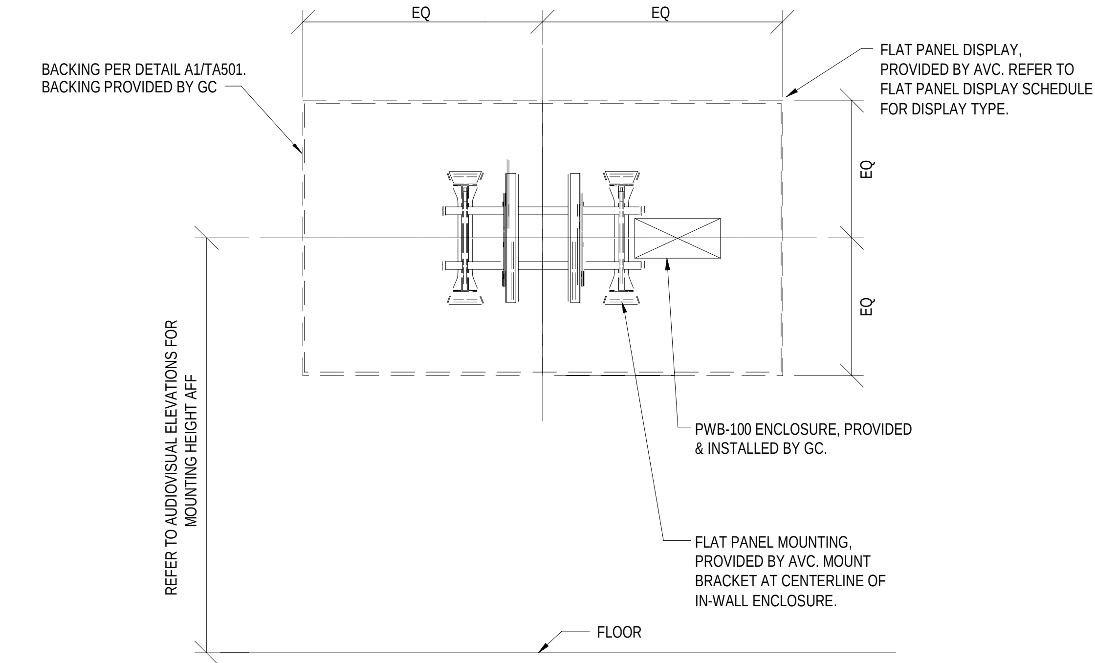
C3 FLAT PANEL DISPLAY BRACKET DETAIL ROOM 126 NTS
