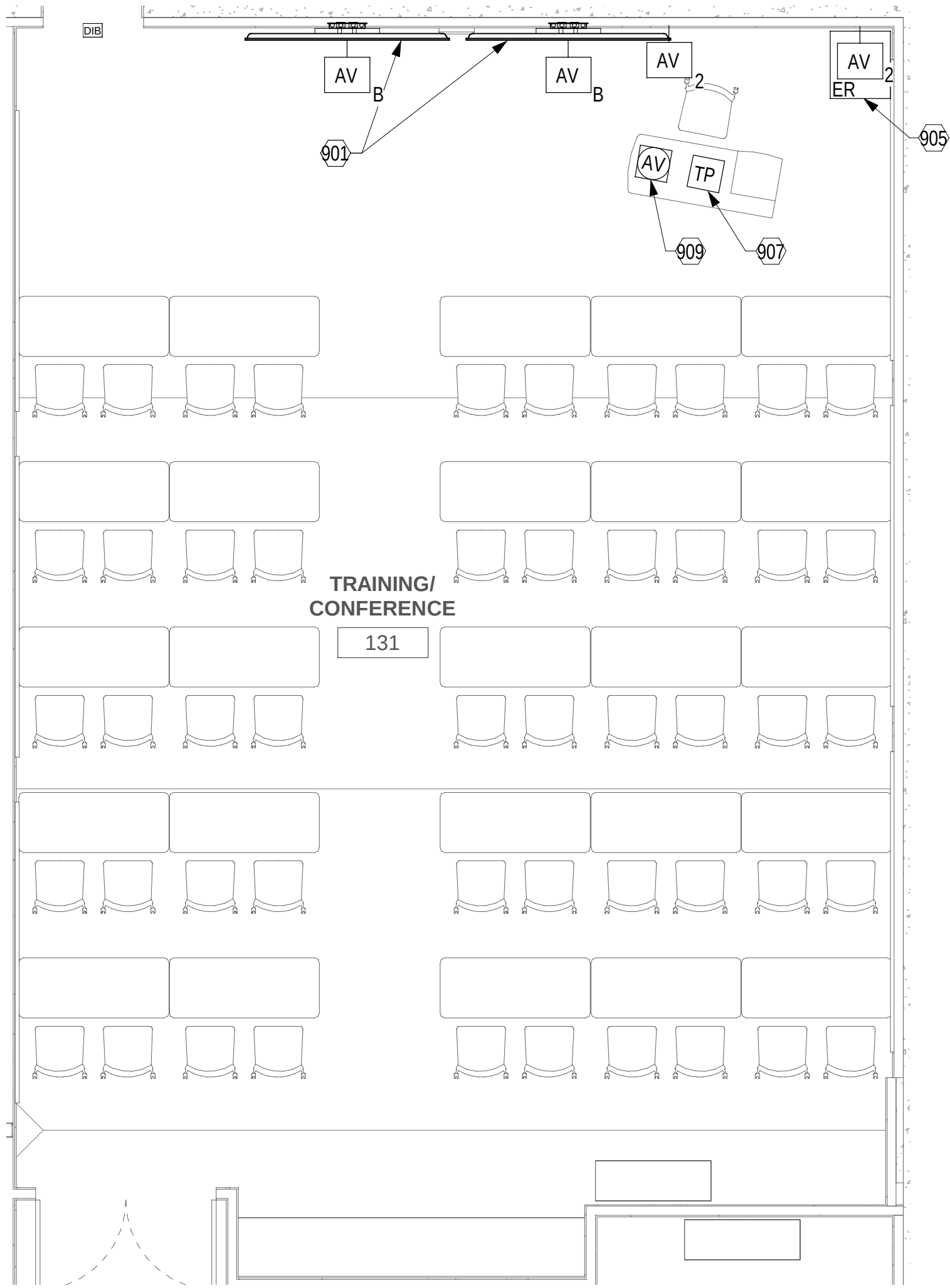
A1 AUDIO VISUAL ENLARGED PLANS - ROOM 131 1/4" = 1'-0" (TA101)
