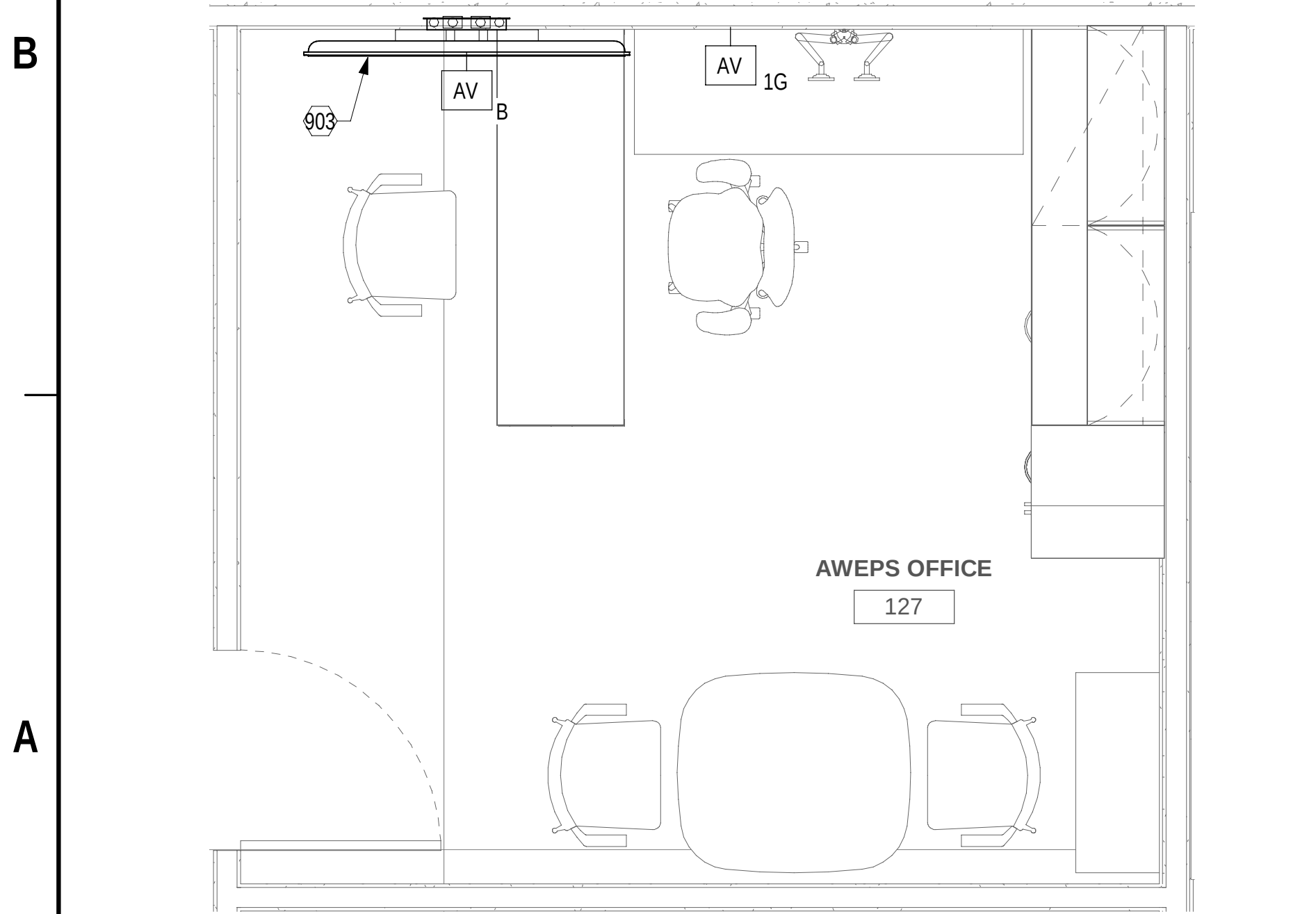
A1 AUDIO VISUAL ENLARGED PLAN - ROOM 127 1/2" = 1'-0" (TA101)
