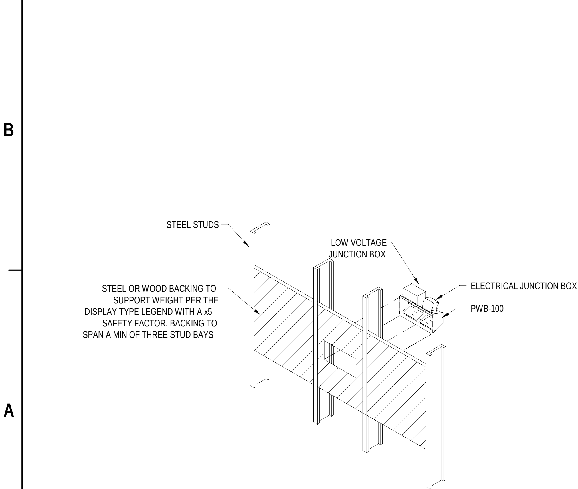
A1 BLOCKING DETAIL NTS
