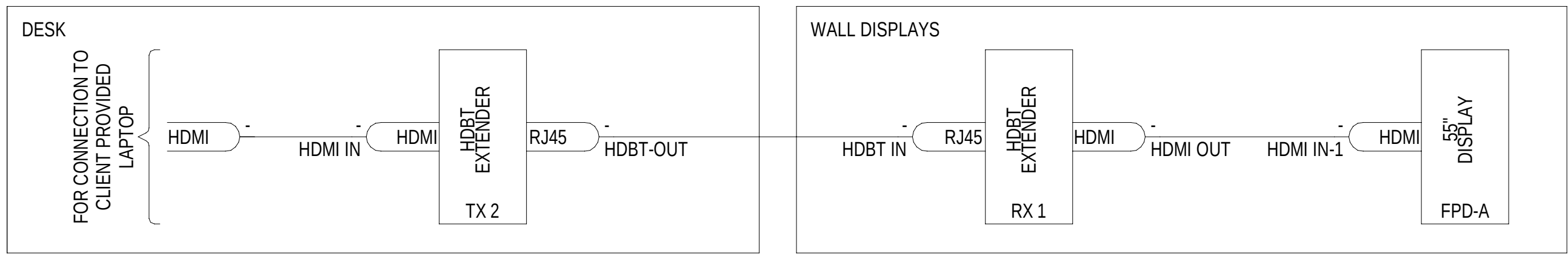
B1 AUDIO VISUAL FLOW DIAGRAM - TRAINING ROOM 131 NTS
