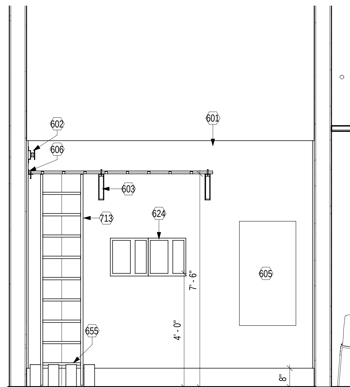
C1 TELECOM 105 - SOUTH ELEVATION 1/2" = 1'-0" (T-102)
