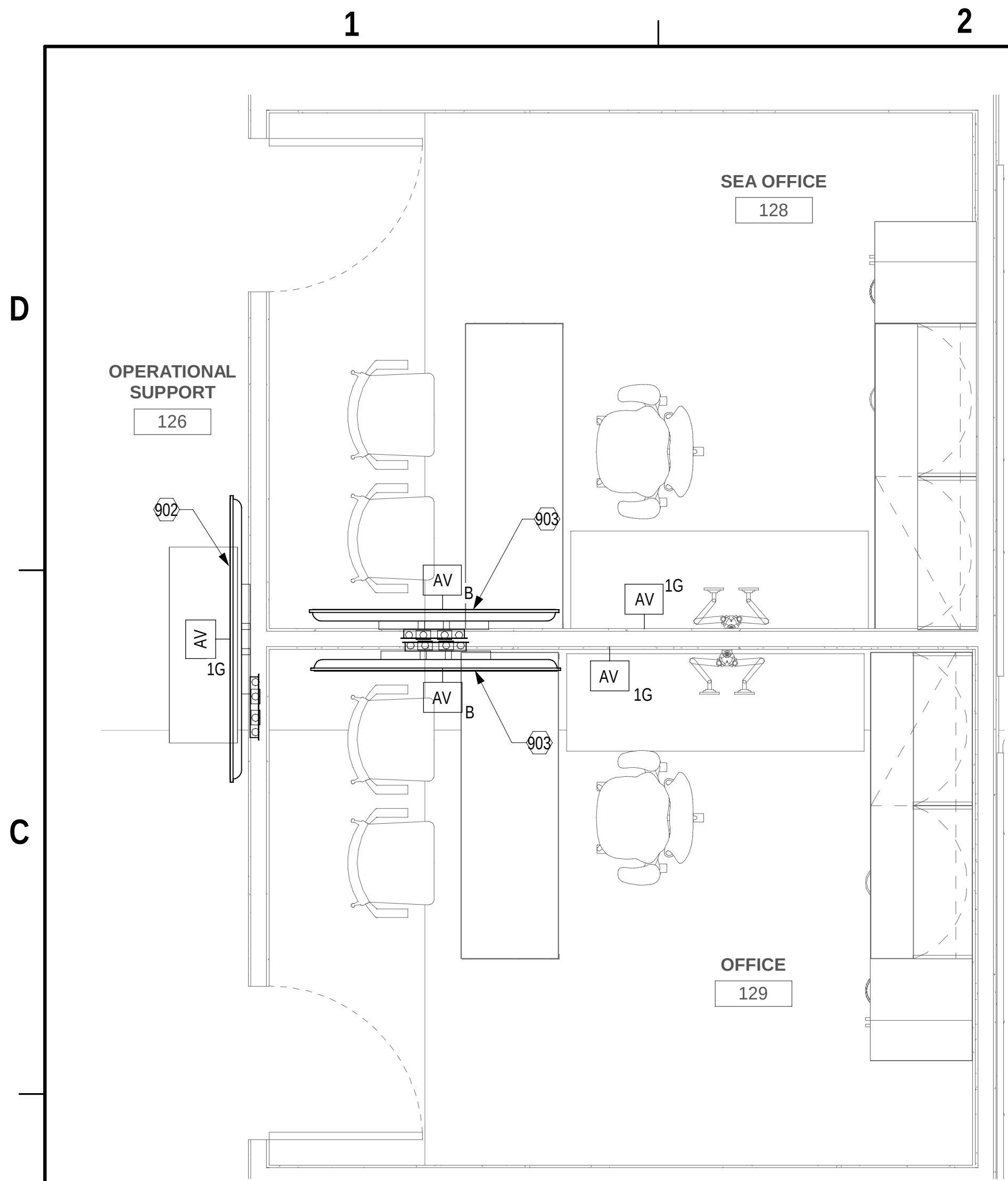
C1 AUDIO VISUAL ENLARGED PLAN - ROOMS 126, 128 & 129 1/2" = 1'-0" (TA101)
