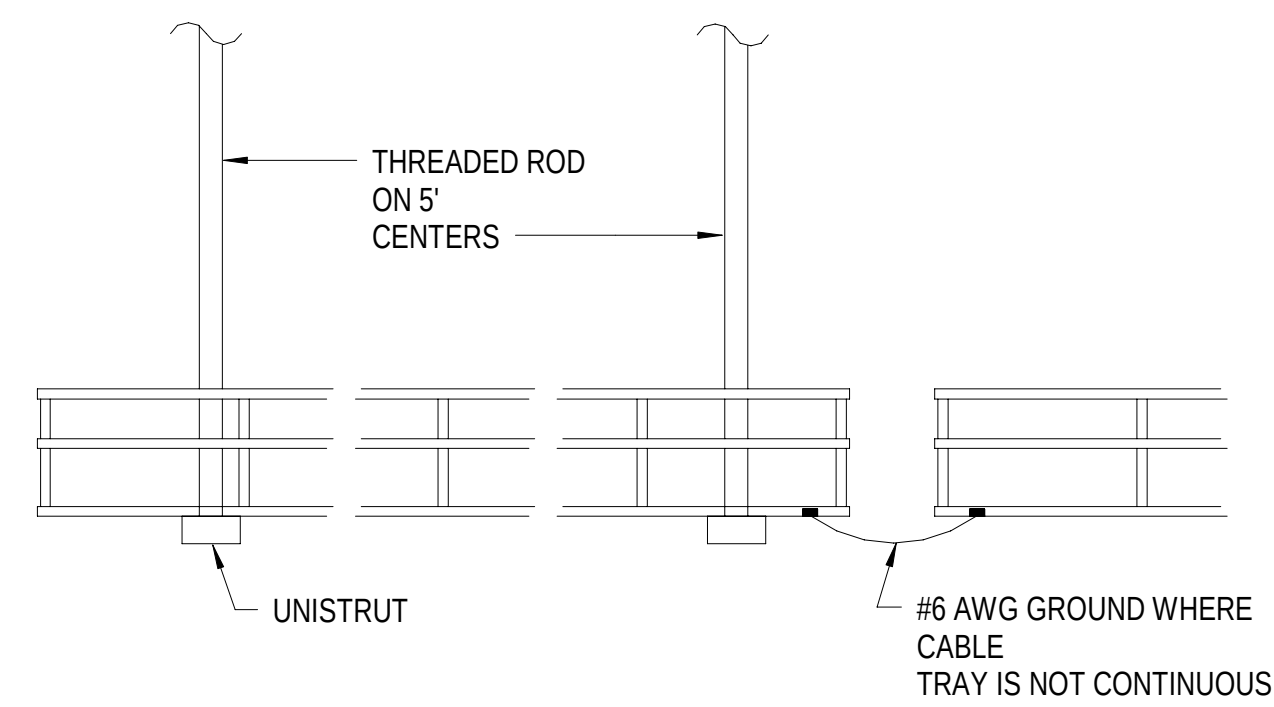
MOUNTING AND BONDING DETAIL
