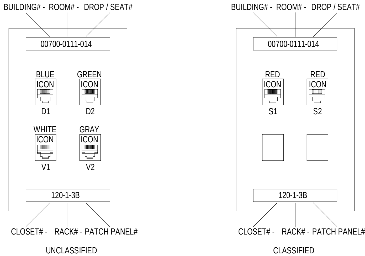
D4 WALL PLATE NTS
