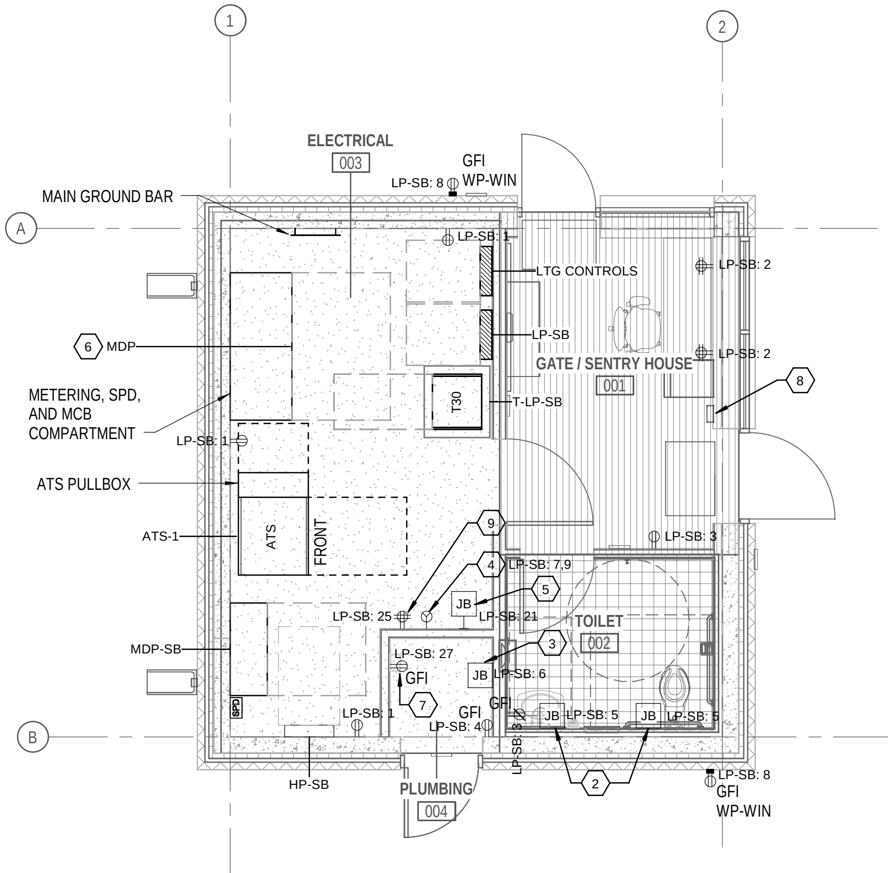
A3 POWER PLAN 1/4" = 1'-0"
