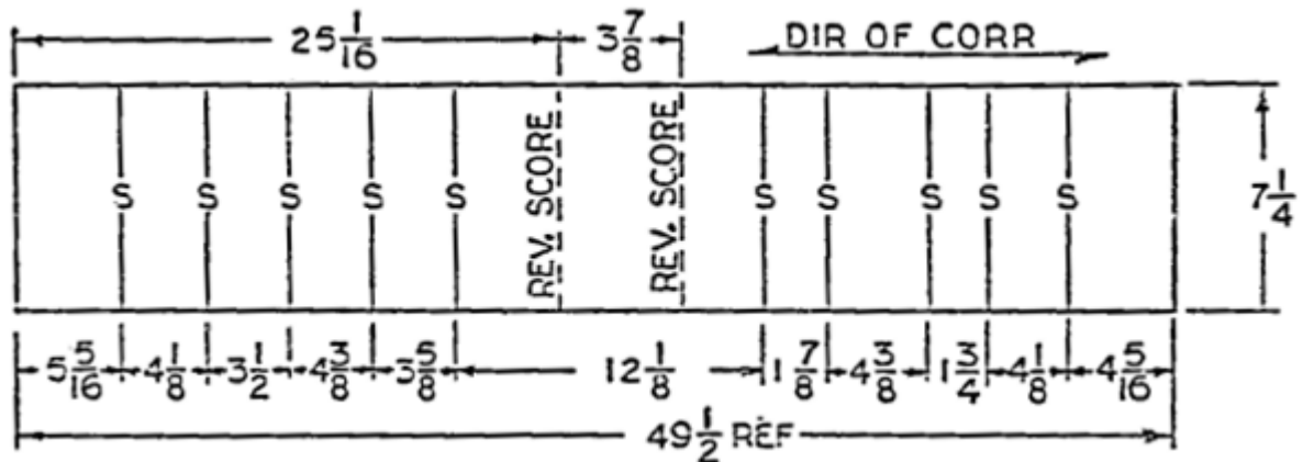
FIGURE 2 – DETAIL B – SIZE AND SCORE DIMENSIONS
