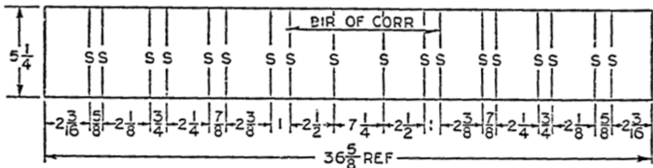
FIGURE 5 – DETAIL E – SIZE AND SCORE DIMENSIONS
