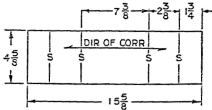
FIGURE 1 – DETAIL A – SIZE AND SCORE DIMENSIONS
