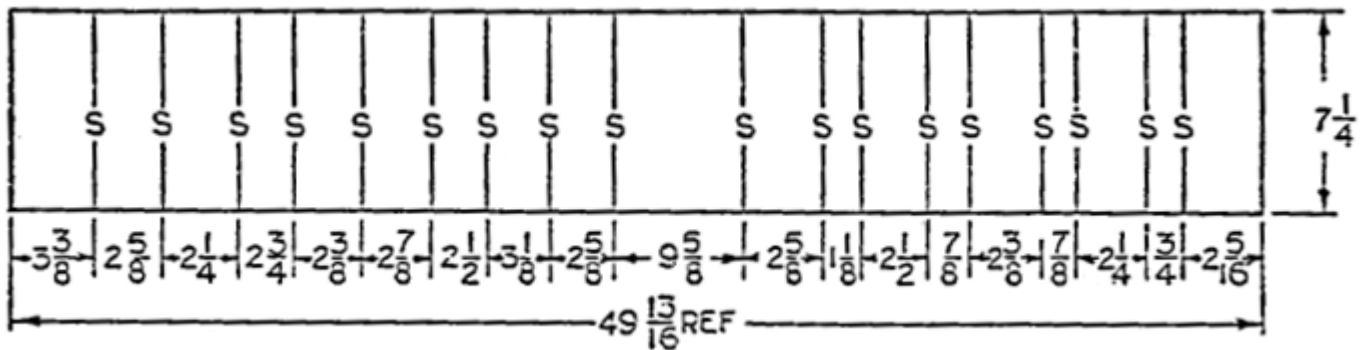
FIGURE 4 – DETAIL D – SIZE AND SCORE DIMENSIONS
