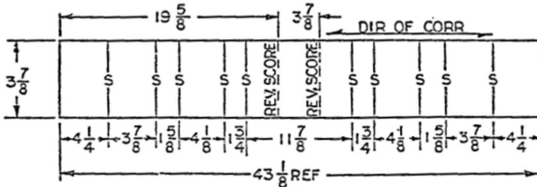
FIGURE 3 – DETAIL C – SIZE AND SCORE DIMENSIONS
