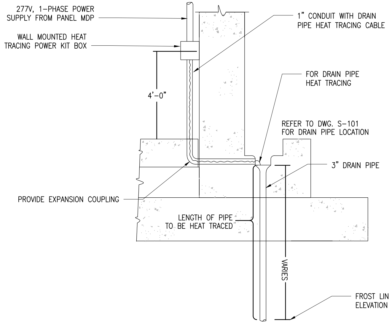
C1 DRAIN PIPE HEAT TRACING DETAIL SCALE: NO SCALE
