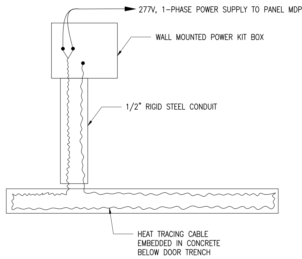
A1 TYPICAL DOOR TRENCH HEAT TRACING WIRING DETAIL SCALE: NO SCALE
