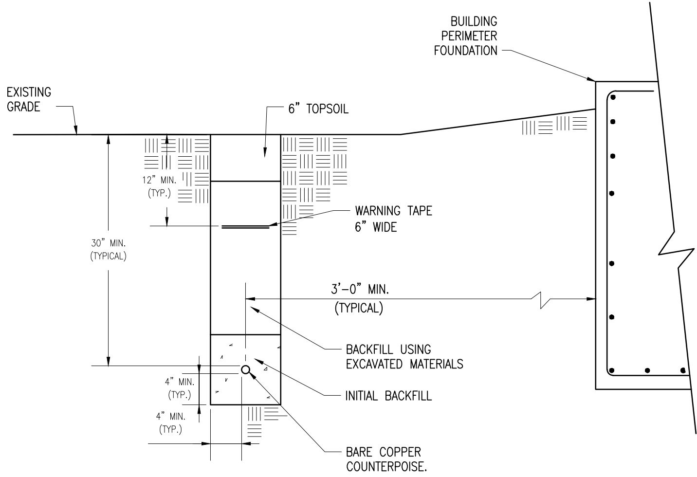
C2 TYPICAL GROUND RING INSTALLATION DETAIL
