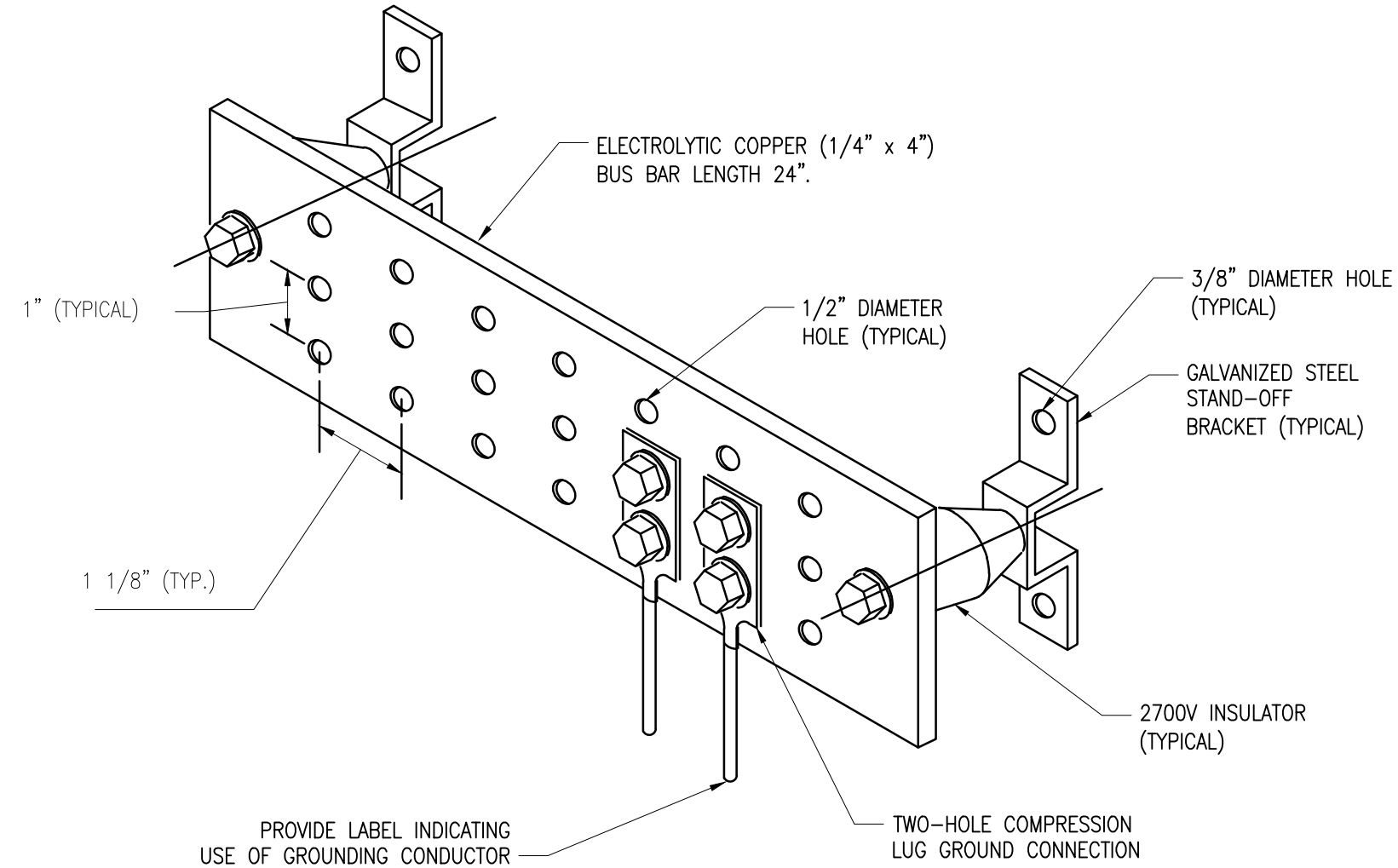
C4 SINGLE POINT GROUNDING BUS BAR (SPGB) BAR DETAIL - TYPICAL
