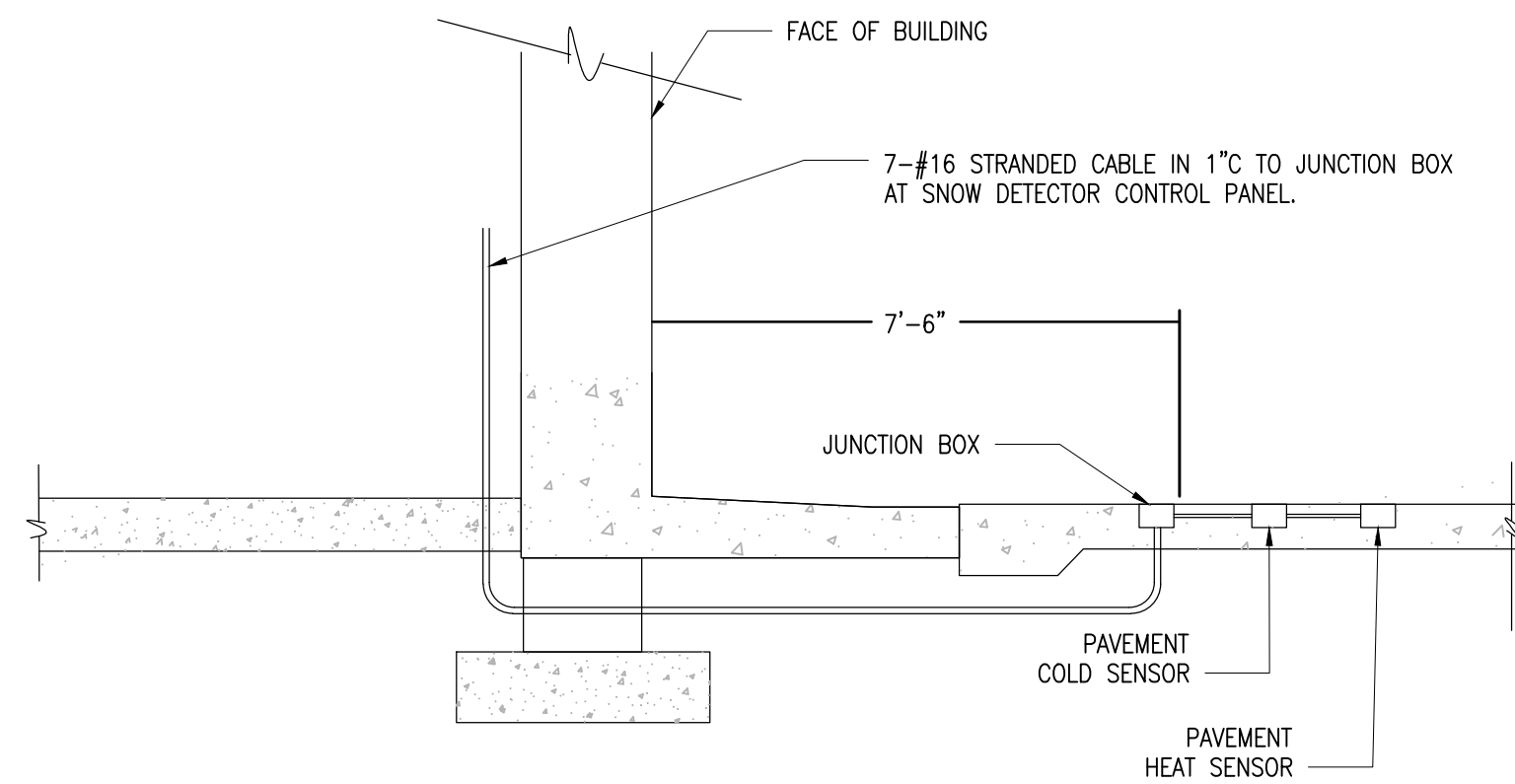
A4 SNOW DETECTOR LOCATION DETAIL SCALE: NO SCALE
