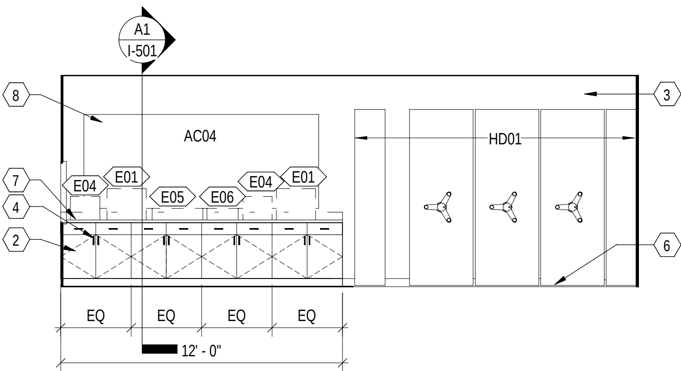
B2 SIPR OIS 107 EAST ELEVATION 1/4" = 1'-0" (I-404)
