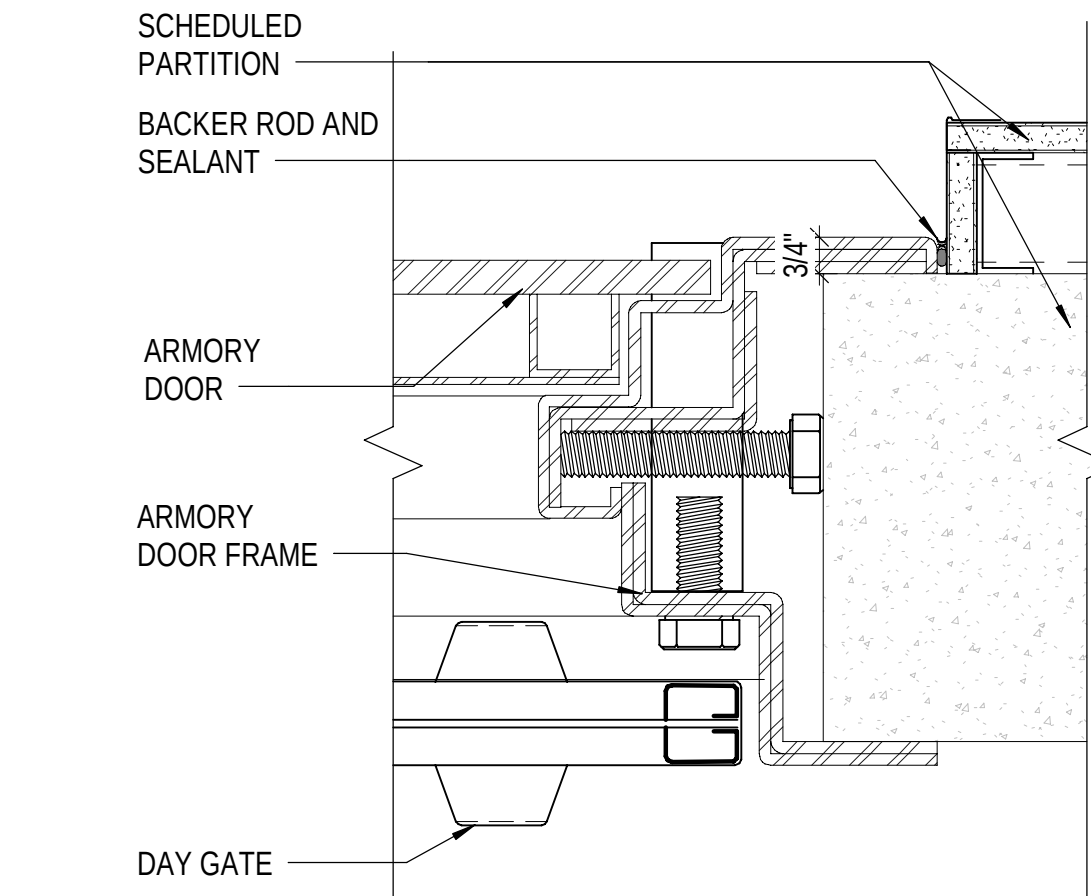
B2 ARMORY DOOR JAMB DETAIL 3" = 1'-0"
