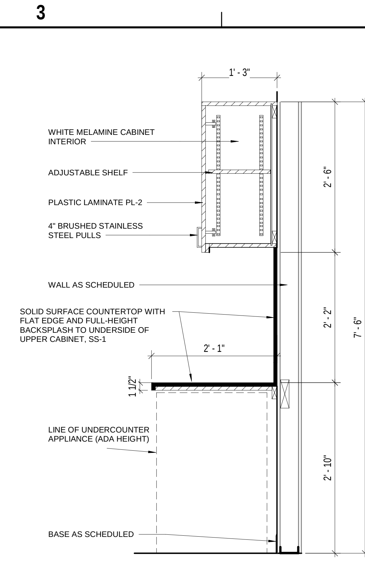
C3 MILLWORK SECTION - UNDERCOUNTER APPLIANCE 1" = 1'-0"
