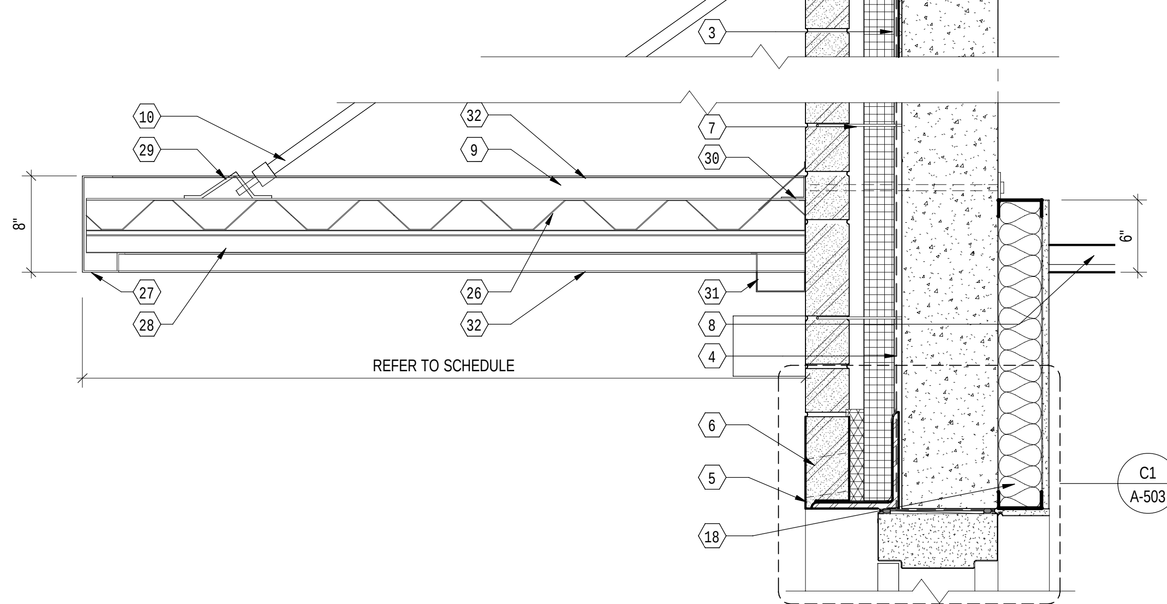
C2 CANOPY/ WALL DETAIL 1 1/2" = 1'-0" (A-302)
