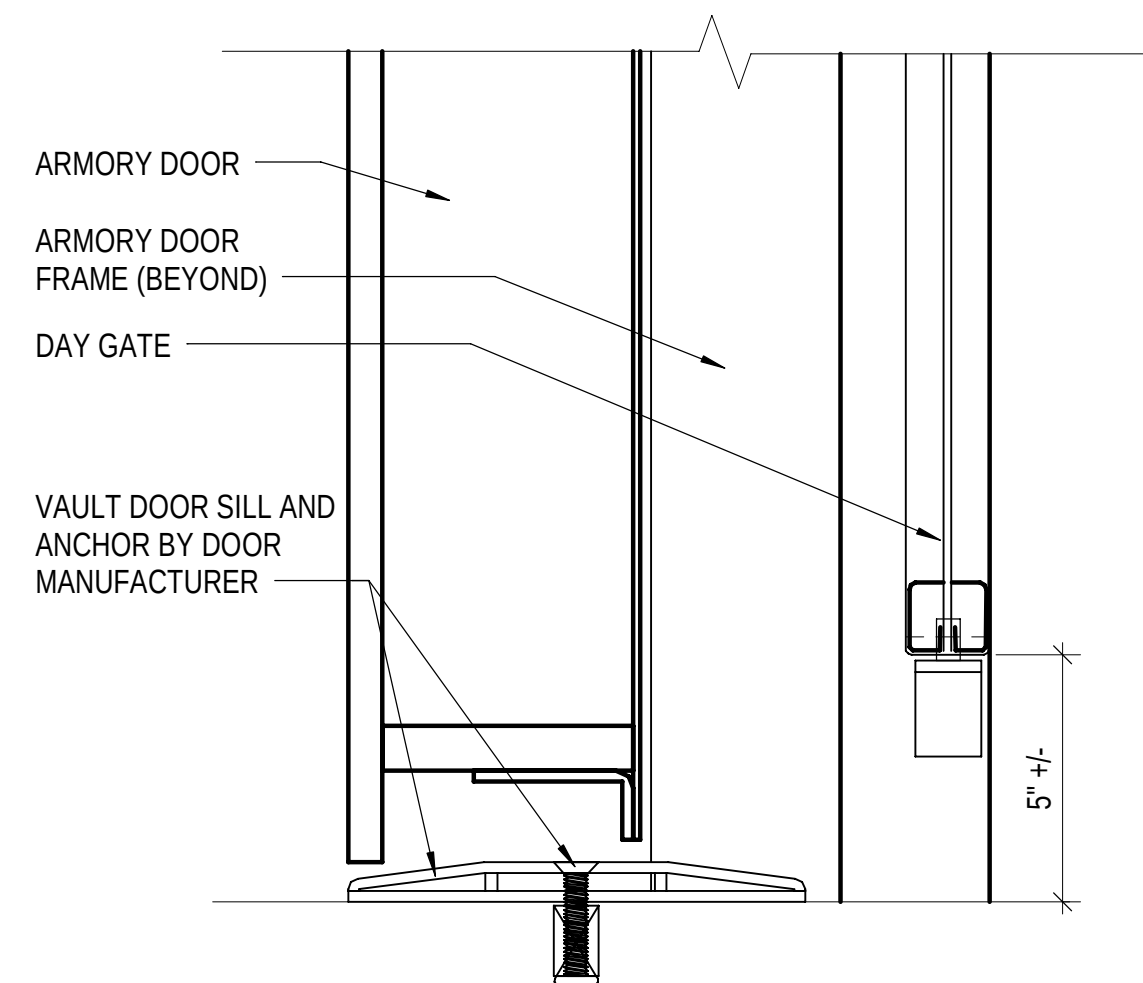
A2 ARMORY DOOR SILL DETAIL 3" = 1'-0"
