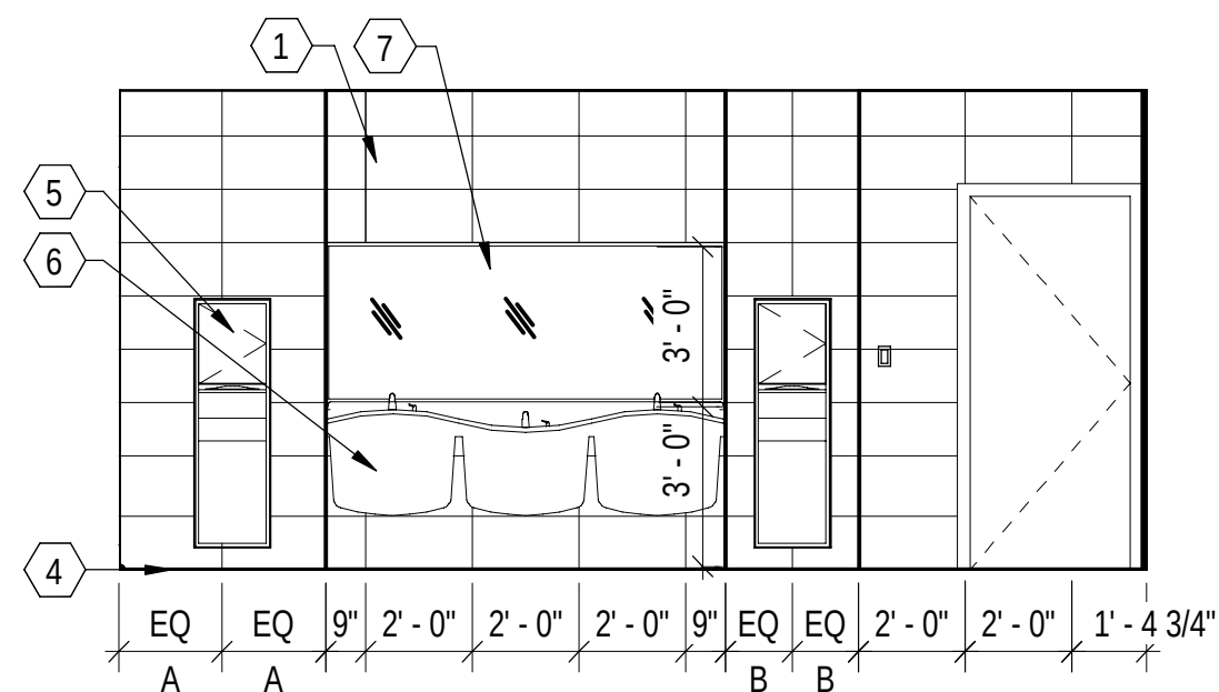
A2 RESTROOM SINK TILE TYPICAL ELEVATION 1/4" = 1'-0" (A-401)
