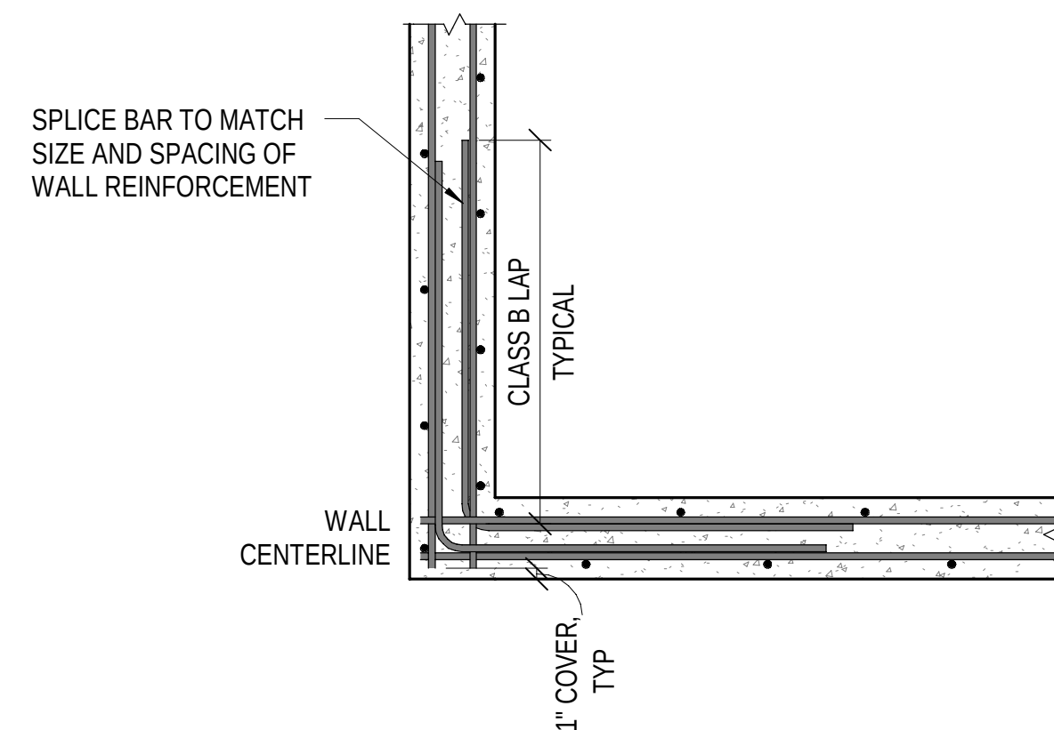
A2 ARMS ROOM WALL CORNER REINFORCEMENT
