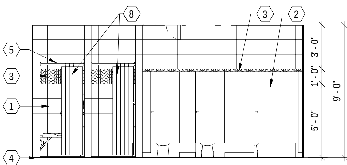
A3 WOMEN'S TOILETS/ SHOWER ROOM 121 ELEVATION 1/4" = 1'-0" (A-401)
