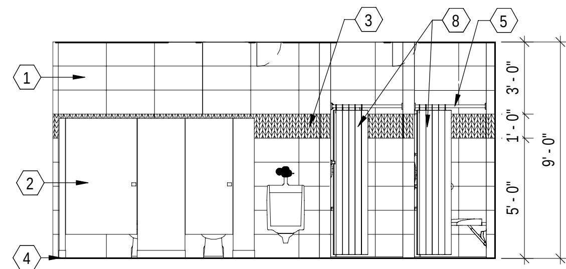
B3 MEN'S TOILETS/ SHOWER ROOM 116 ELEVATION 1/4" = 1'-0" (A-401)
