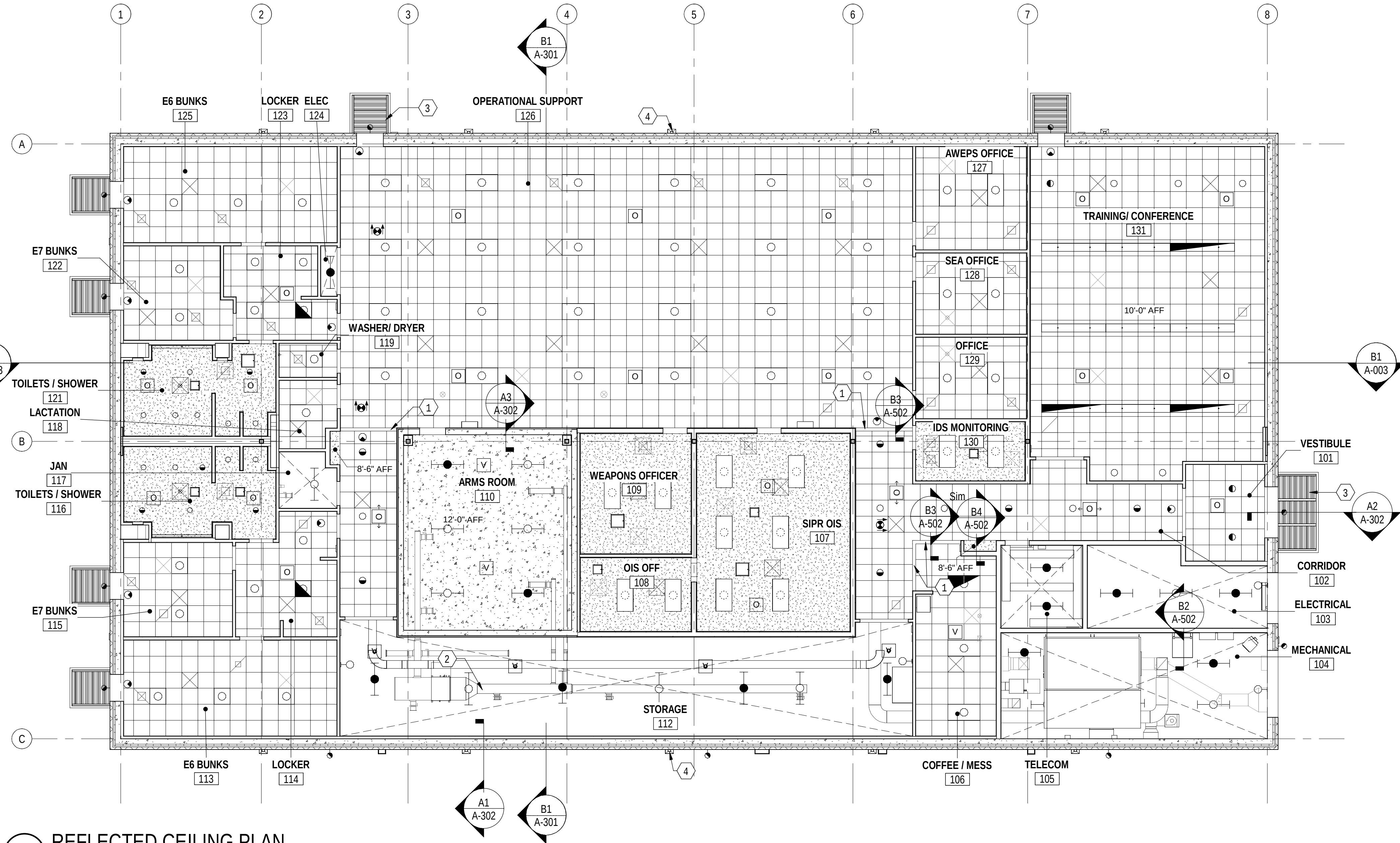
B1 REFLECTED CEILING PLAN 1/8" = 1'-0"
