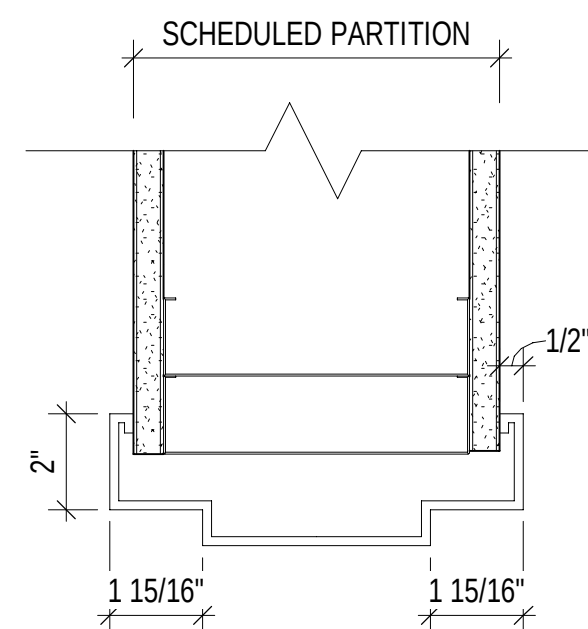
A4 INT. DOOR HEAD/ JAMB DETAIL 3" = 1'-0"
