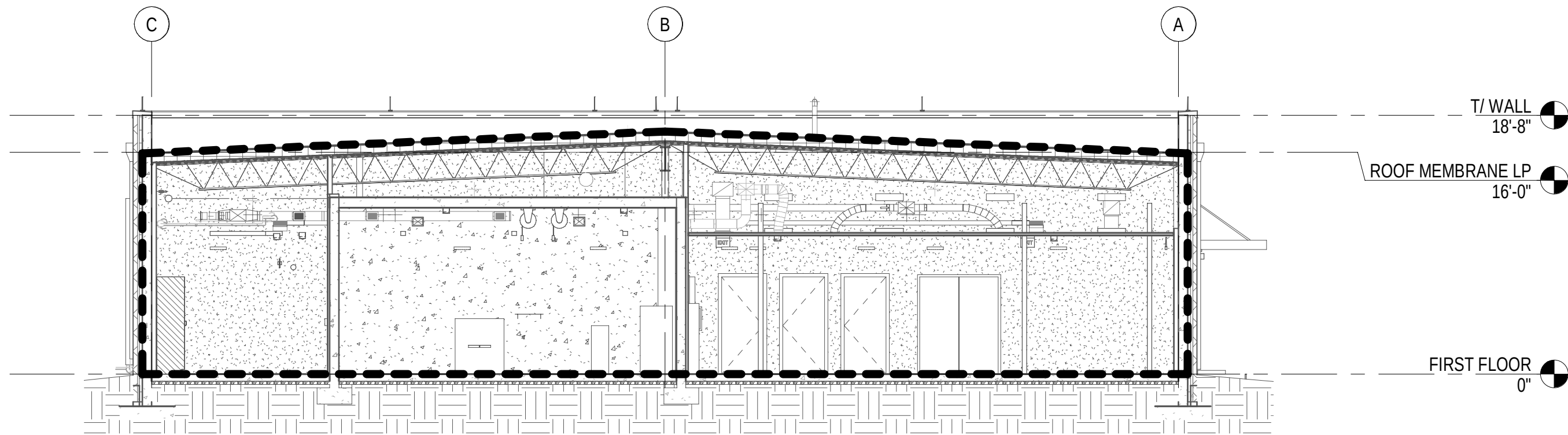
C1 NORTH-SOUTH BUILDING SECTION 1/8" = 1'-0"
