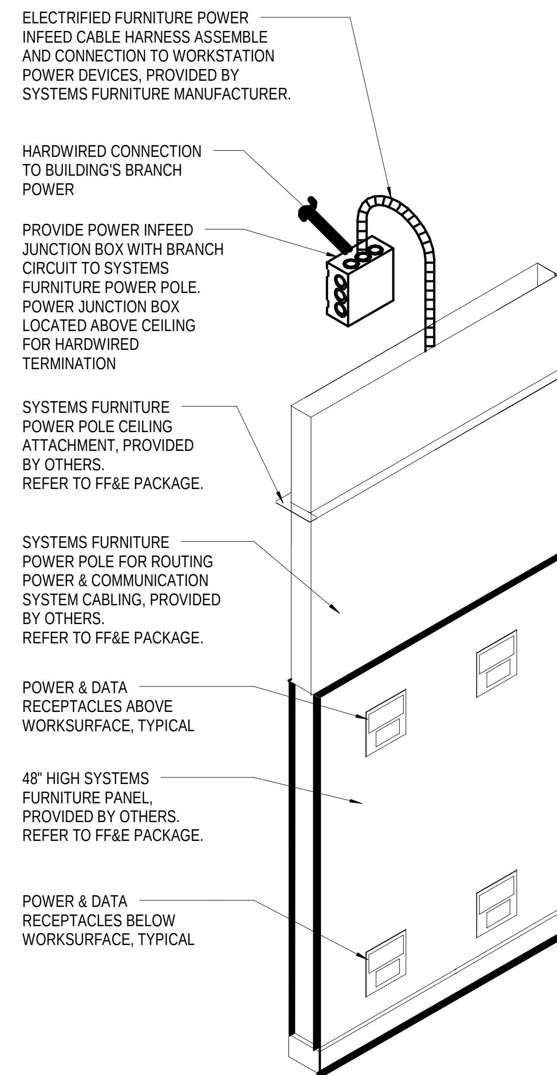
A3 SYSTEMS FURNITURE POWER POLE DETAIL
