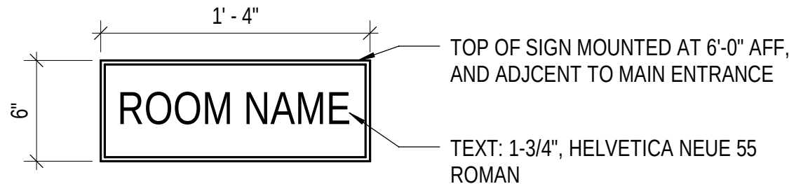
A2 ROOM SIGNAGE 1 1/2" = 1'-0"
