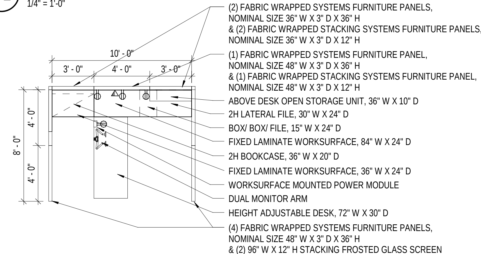
B1 WS03 WORKSTATION PLAN 1/4" = 1'-0"
