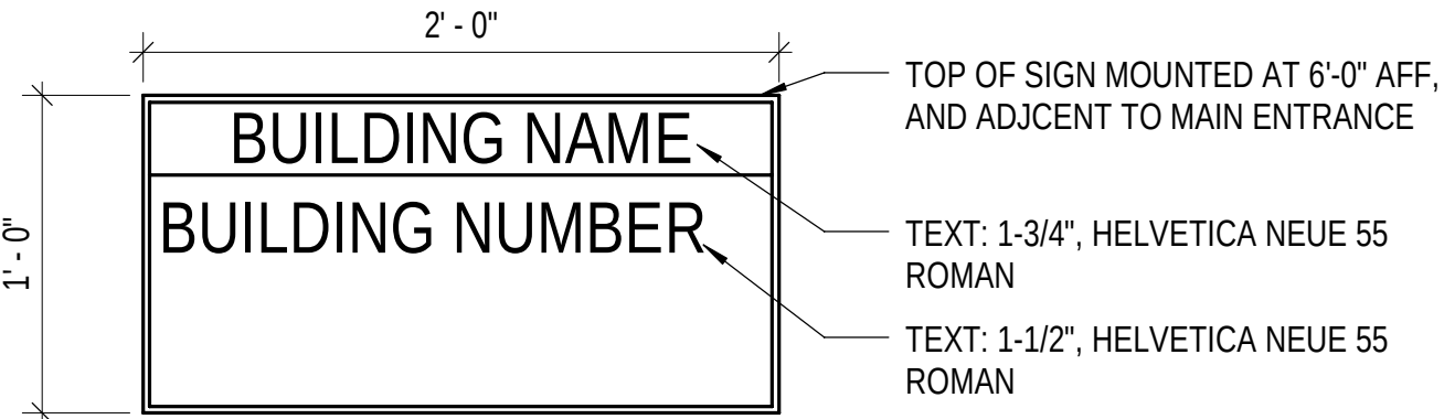
A1 BUILDING SIGNAGE 1 1/2" = 1'-0"
