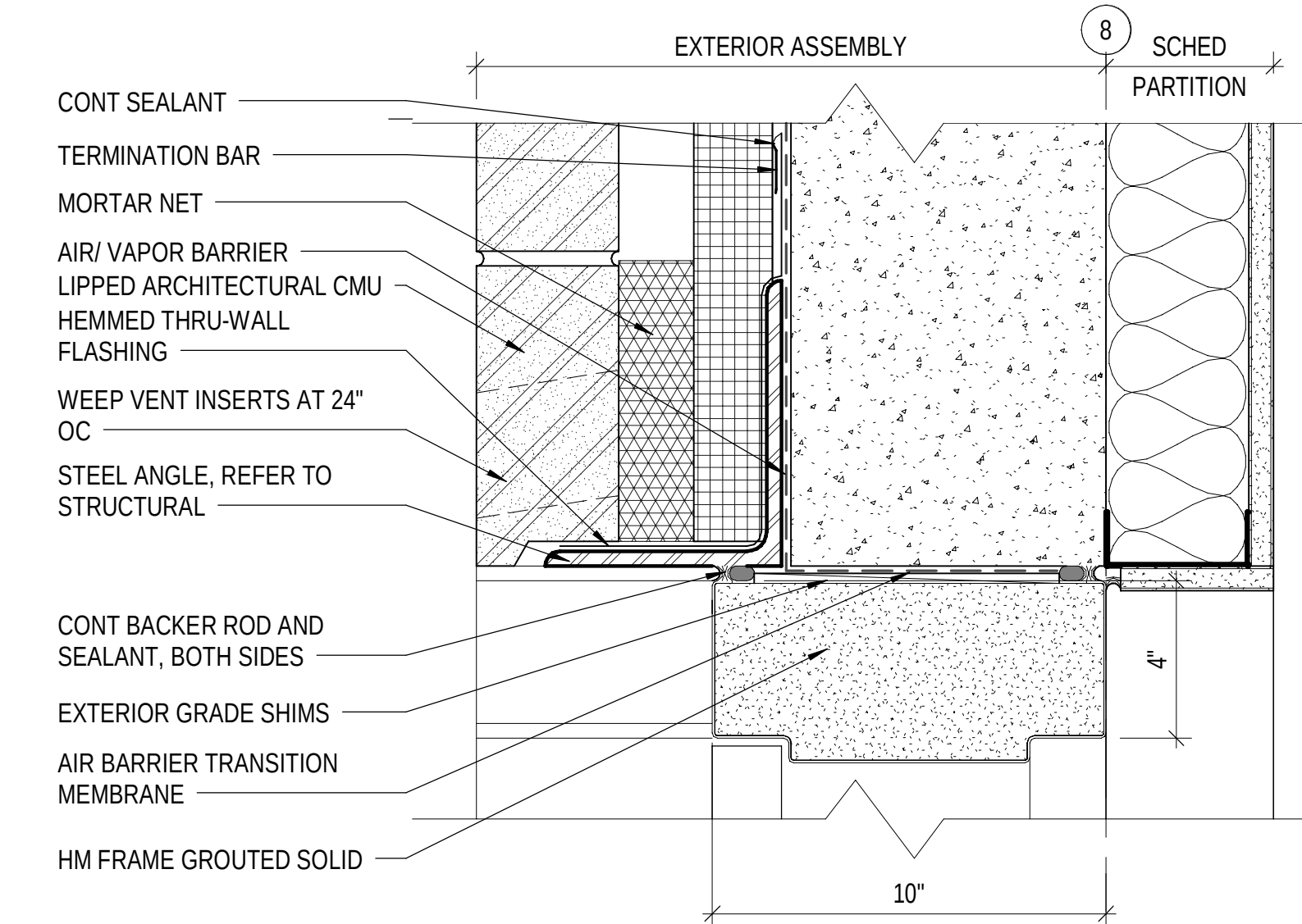
C1 EXT HM DOOR HEAD DETAIL 3" = 1'-0" (A-501)
