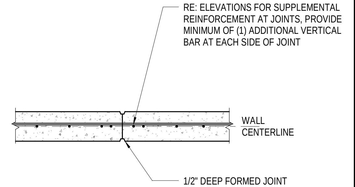
C4 CONCRETE WALL CONSTRUCTION JOINT
