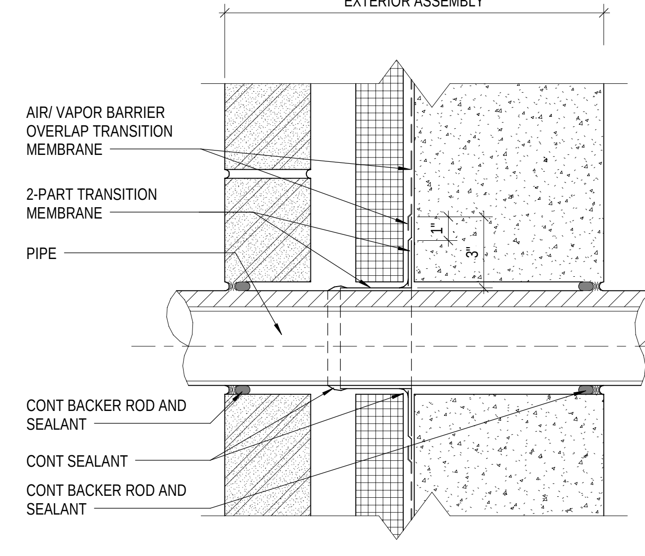
C4 TYPICAL PENETRATION AT AIR BARRIER 3" = 1'-0"
