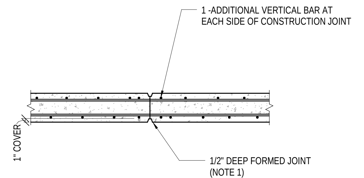
CONCRETE WALL CONSTRUCTION JOINT AT ARMS ROOM
