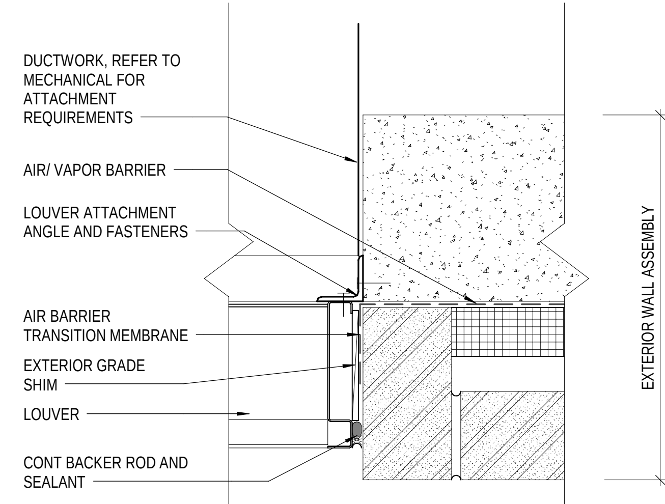
B3 EXT LOUVER JAMB DETAIL 3" = 1'-0"
