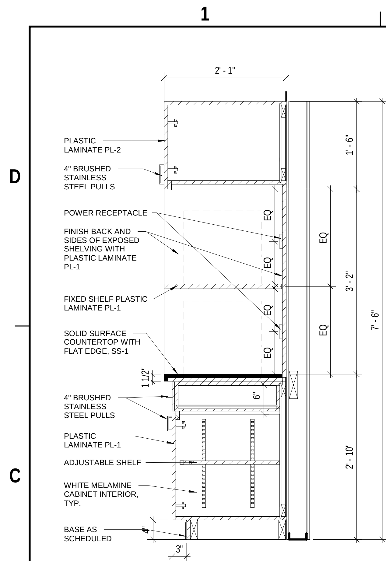
(C1) MILLWORK SECTION - MICROWAVE TOWER 1" = 1'-0"
