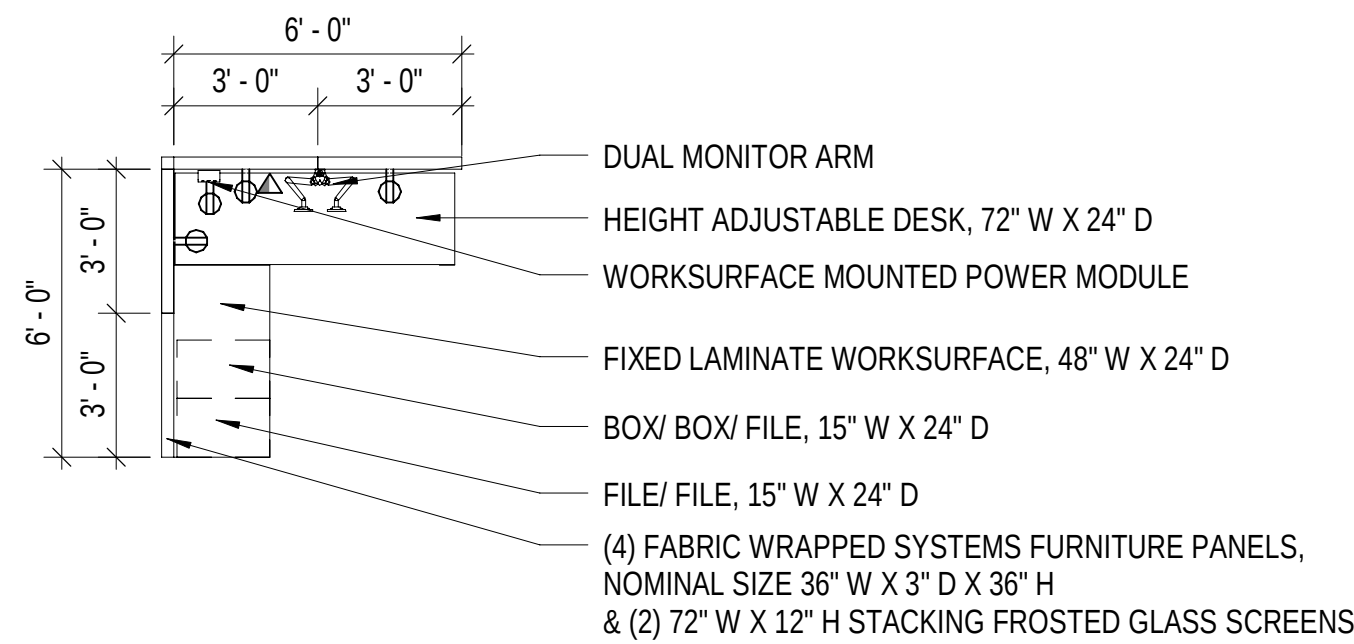
D1 WS01 WORKSTATION PLAN 1/4" = 1'-0"
