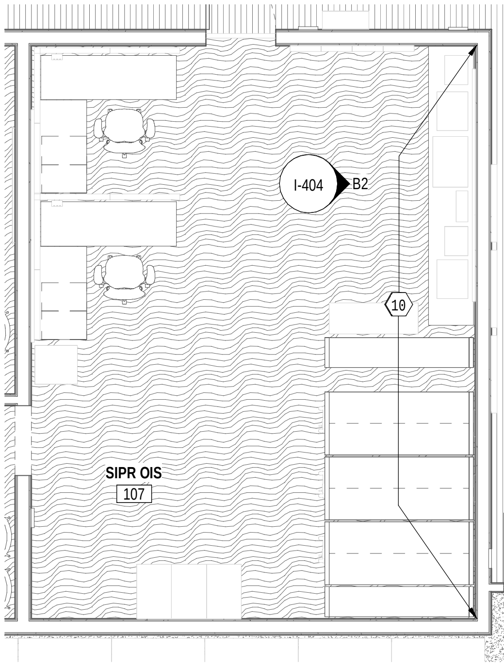
A2 SIPR OIS 107 ENLARGED PLAN 1/4" = 1'-0" (I-102)
