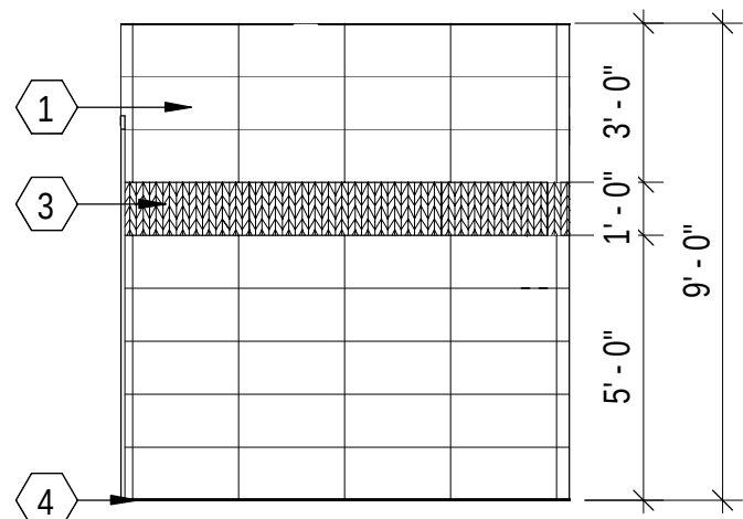
C1 TYPICAL WALL TILE ELEVATION 1/4" = 1'-0" (A-401)
