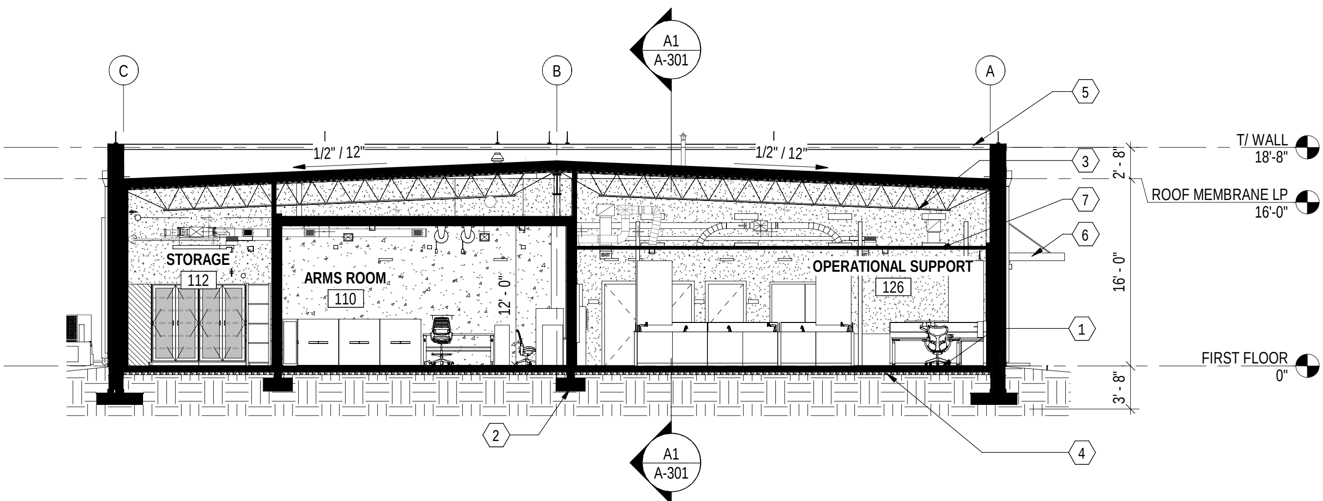
B1 NORTH-SOUTH BUILDING SECTION 1/8" = 1'-0" (A-101)
