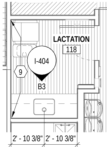
A3 LACTATION 118 ENLARGED PLAN 1/4" = 1'-0" (I-102)
