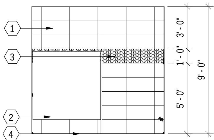
B2 RESTROOM STALL TILE TYPICAL ELEVATION 1/4" = 1'-0"
