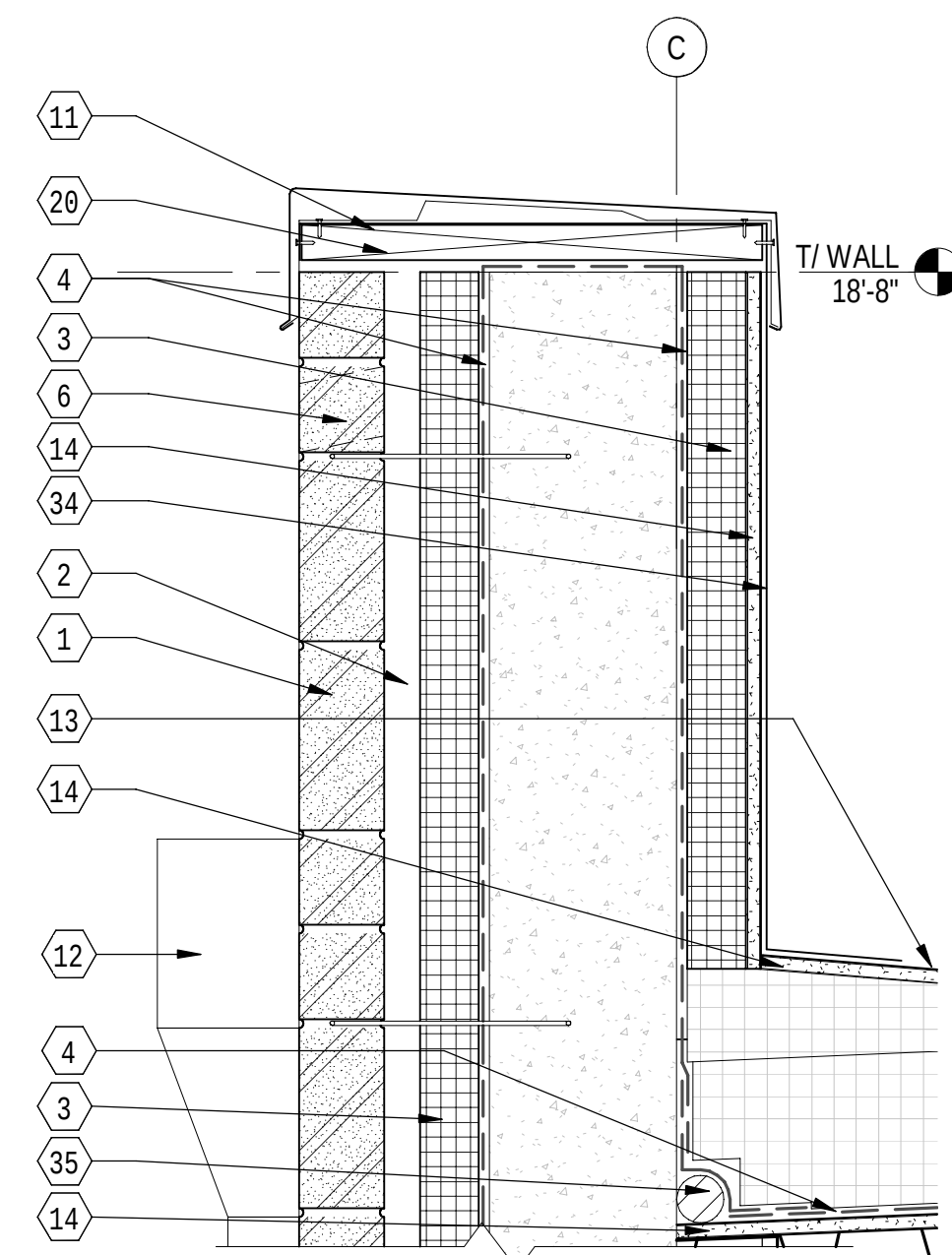
C1 COPING DETAIL 1 1/2" = 1'-0" (A-30)
