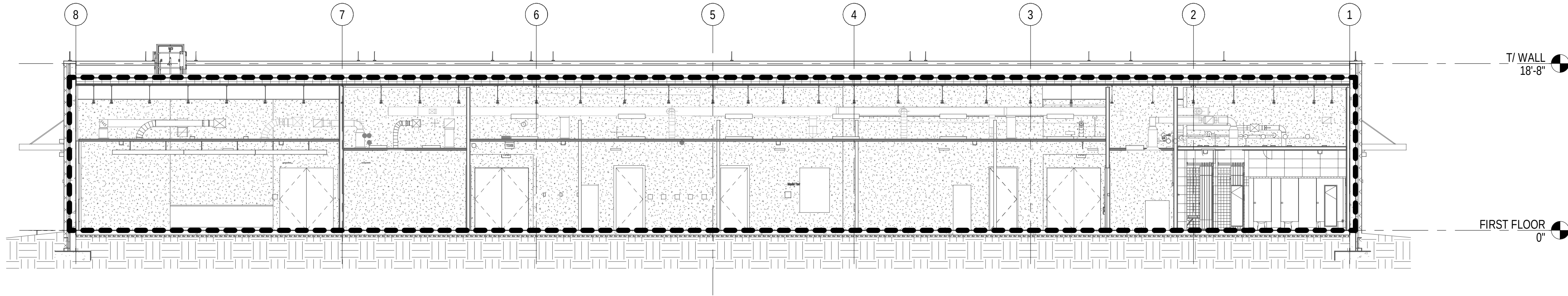
B1 EAST-WEST BUILDING SECTION 1/8" = 1'-0" (A-102)
