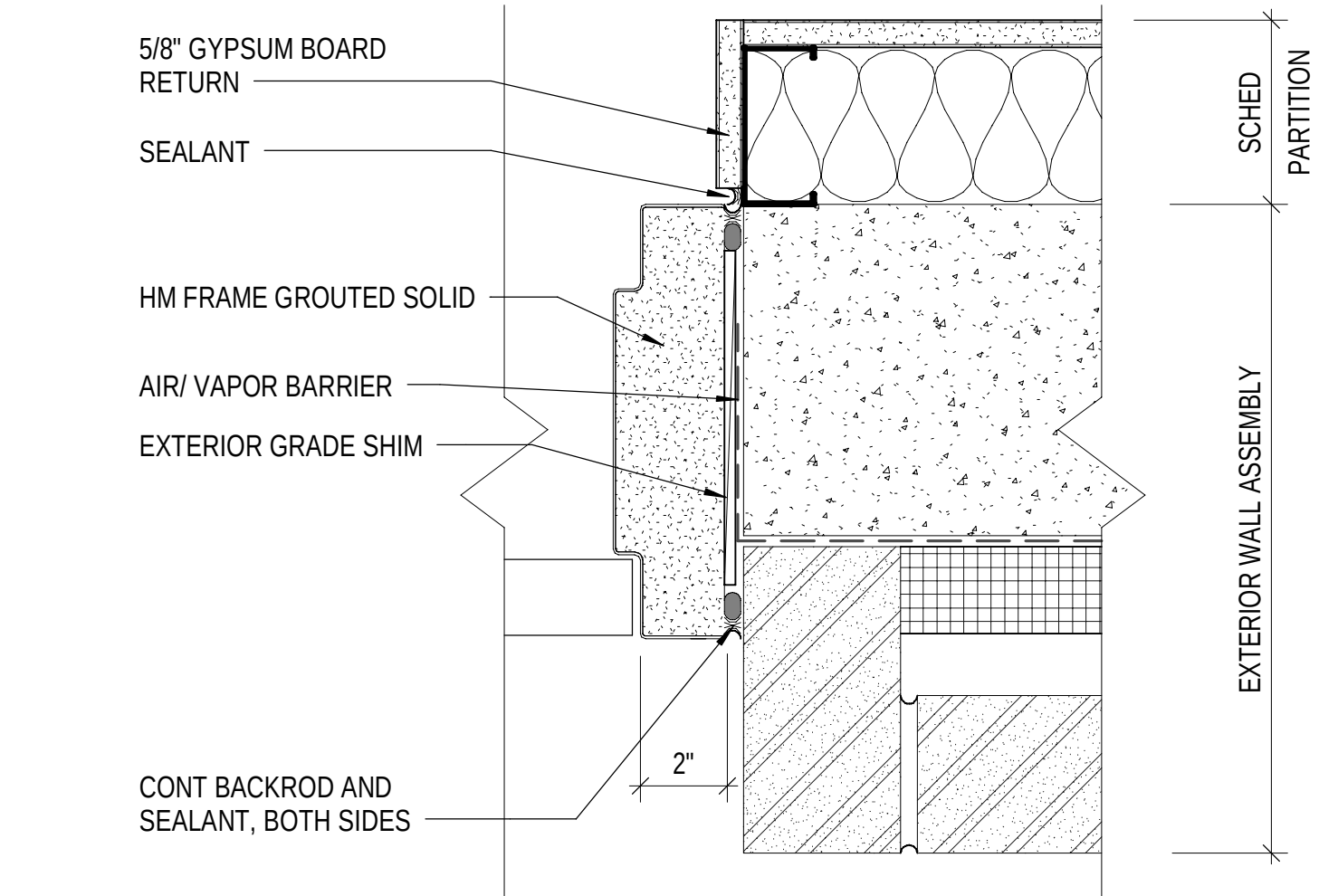
B1 EXT DOOR JAMB DETAIL 3" = 1'-0"
