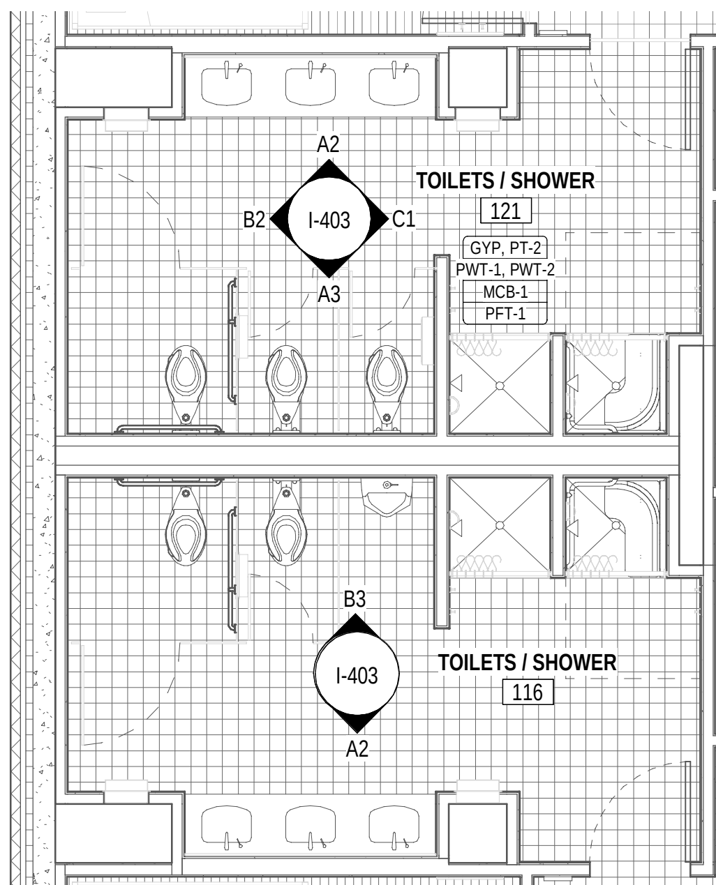
A1 ENLARGED RESTROOMS PLAN 1/4" = 1'-0" (I-102)
