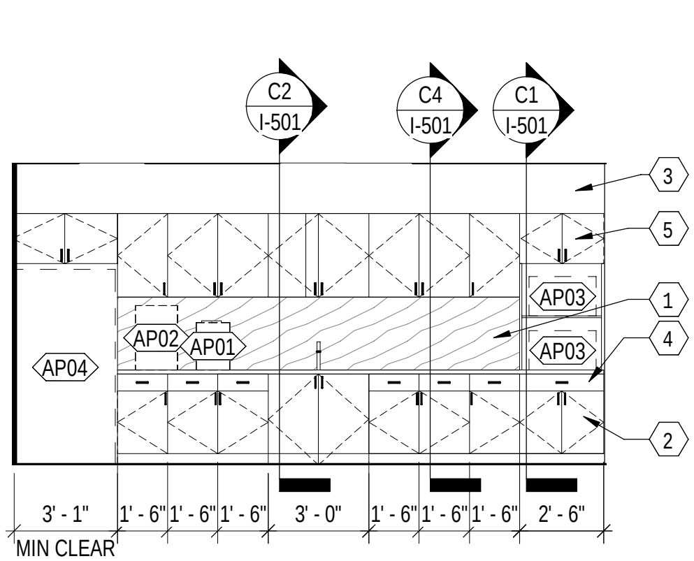
B1 COFFEE/MISC 106 WEST ELEVATION 1/4" = 1'-0" (I-404)
