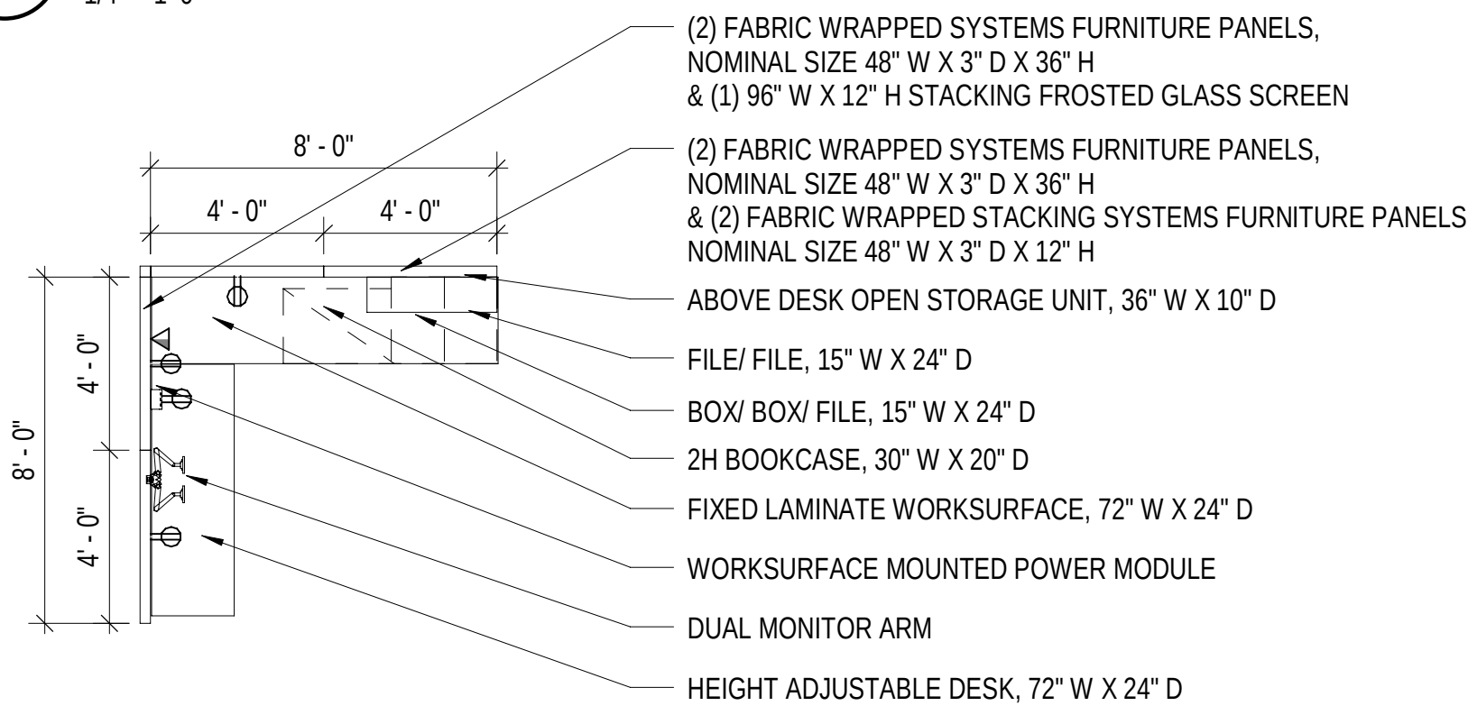
D1 WS01 WORKSTATION PLAN 1/4" = 1'-0"
