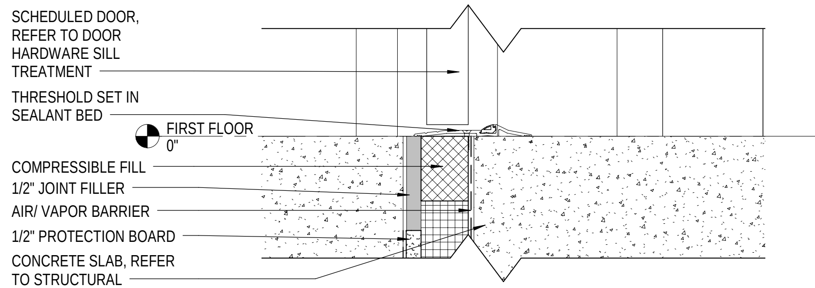
A1 EXT DOOR SILL DETAIL 3" = 1'-0" (A-501)
