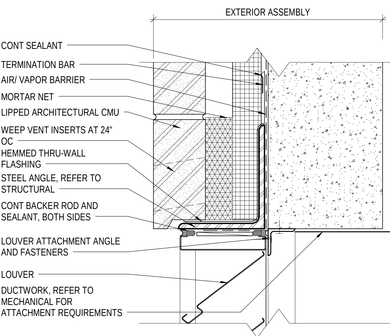
C3 EXT LOUVER HEAD DETAIL 3" = 1'-0"
