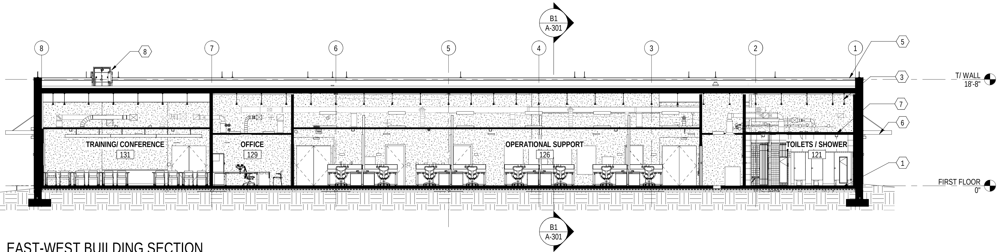
A1 EAST-WEST BUILDING SECTION 1/8" = 1'-0" (A-101)
