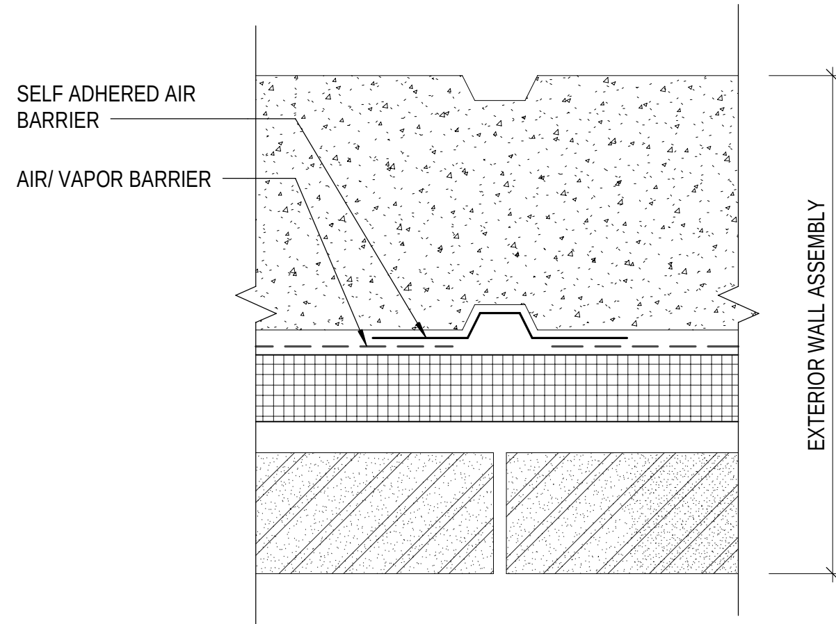
B4 AIR BARRIER AT CONTROL JOINT 3" = 1'-0"
