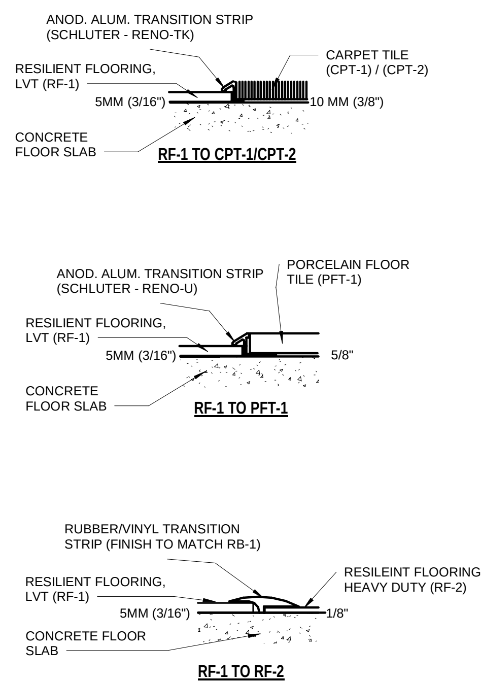
A2 FLOORING TRANSITION DETAILS 6" = 1'-0"
