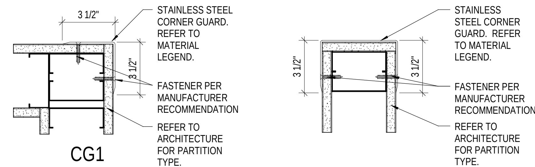
B4 CORNER GUARDS DETAIL 3" = 1'-0"
