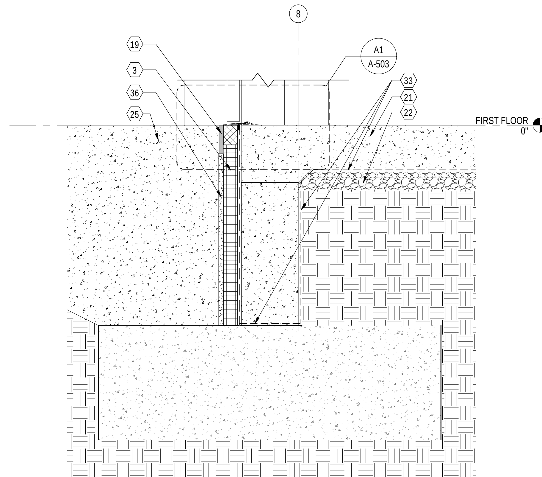
A3 ENTRY/ FOUNDATION DETAIL 1 1/2" = 1'-0" (A-302)
