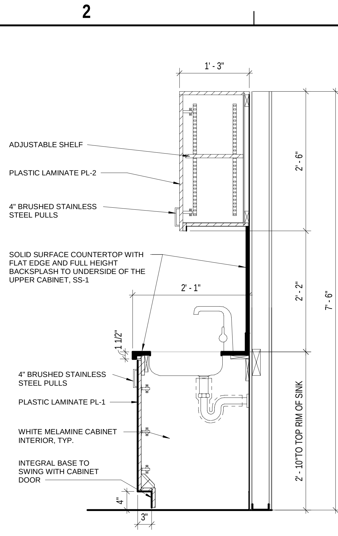
C2 MILLWORK SECTION - CABINET AT SINK 1" = 1'-0"
