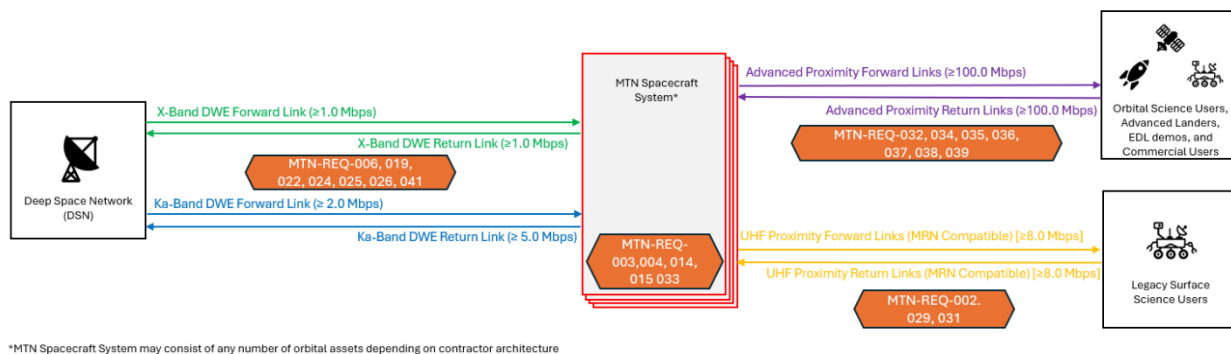
Figure 2 Mars Telecommunications Network (MTN) Goal Configuration
