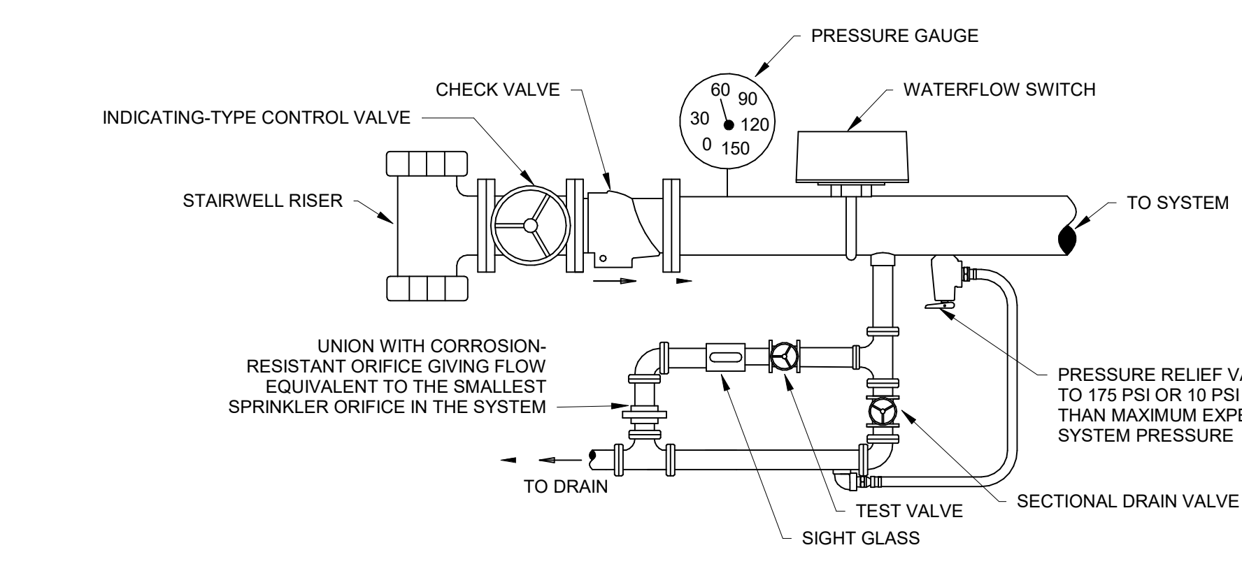
TYPICAL ZONE CONTROL ASSEMBLY (PRESSURE GAUGE) D6 NTS
