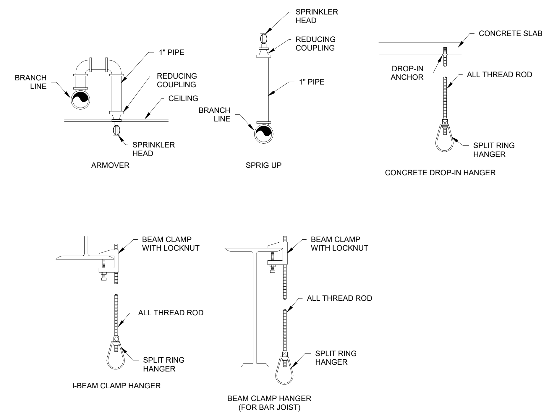
SPRINKLER ARMOVER, SPRIG, AND HANGER DETAILS F6 NTS
