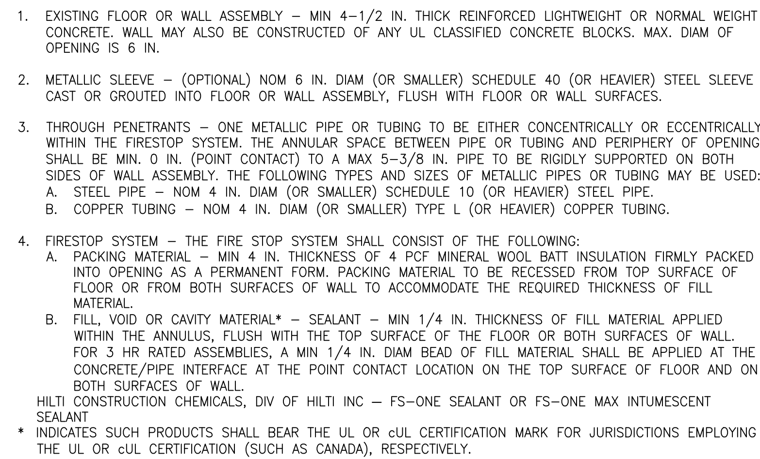
2 TYPICAL CONCRETE OR MASONRY PIPE PENETRATION SCALE: NTS
