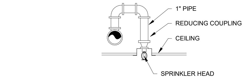
SEMI-RECESSED SPRINKLER HEAD DETAIL D8 NTS
