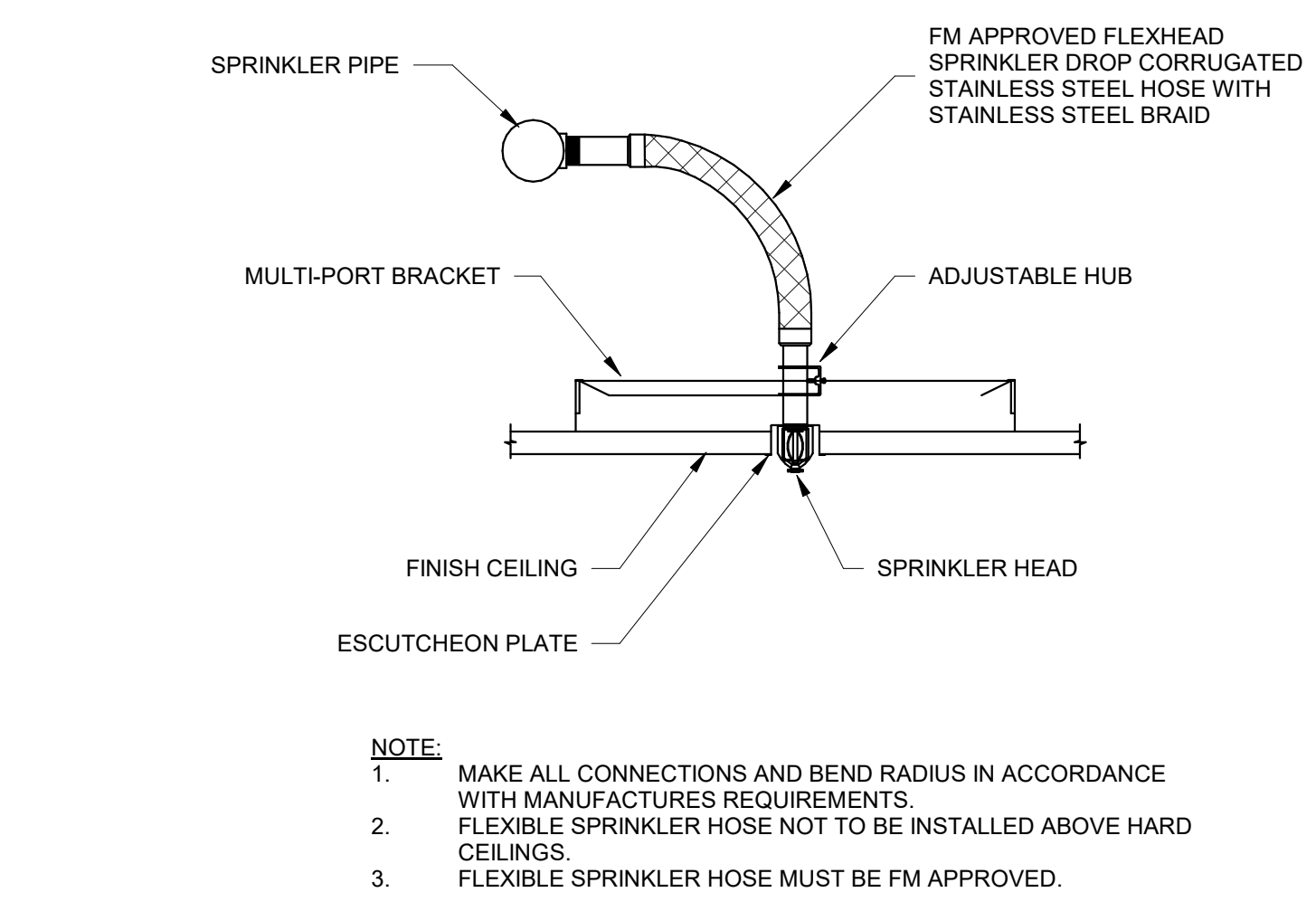
TYPICAL FLEXIBLE SPRINKLER HOSE DETAIL B6 NTS
