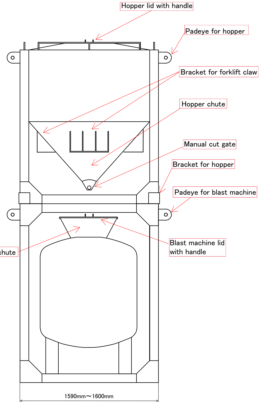
Detail for Blast Machine and Hopper
