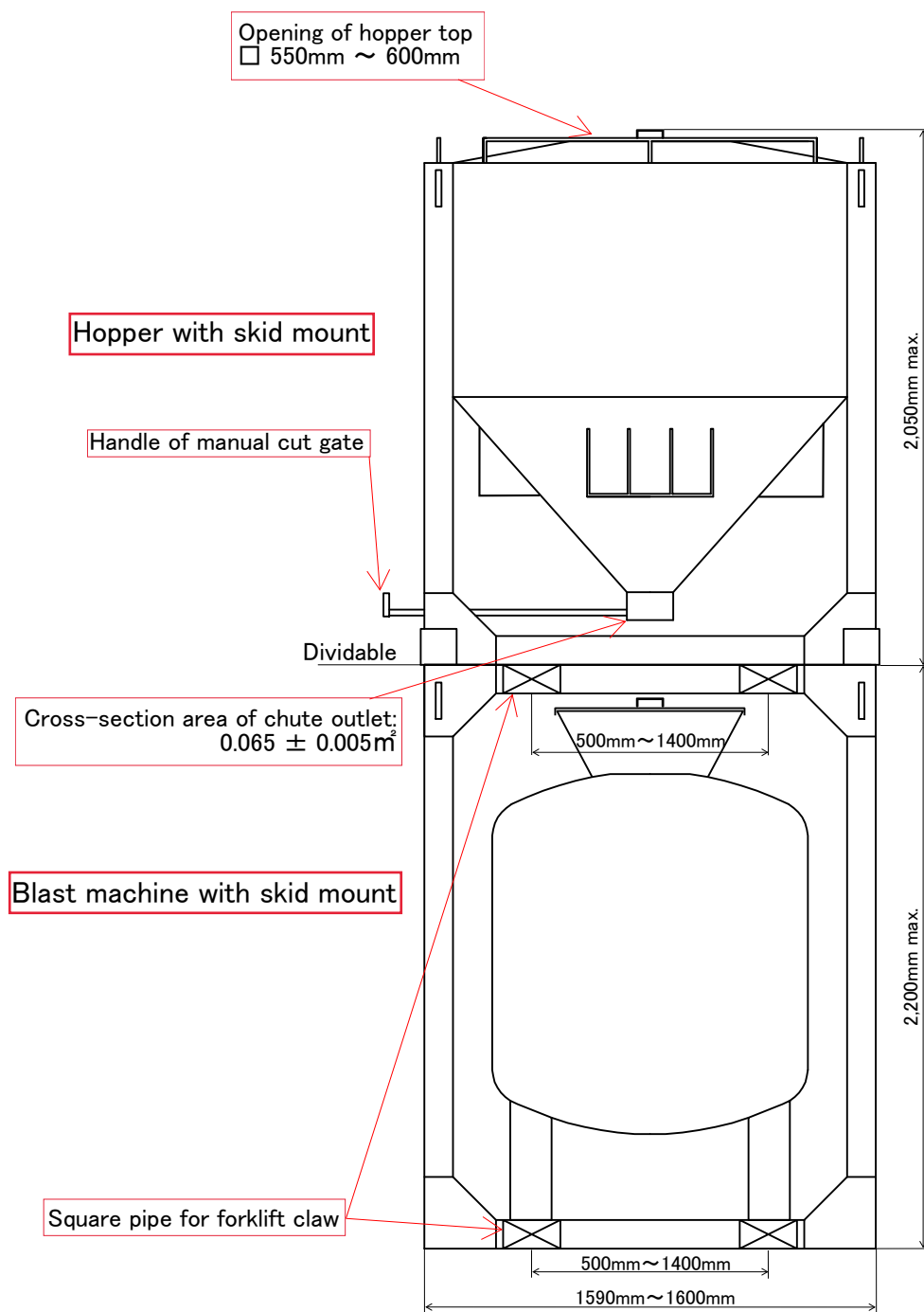
Detail for Blast Machine and Hopper
