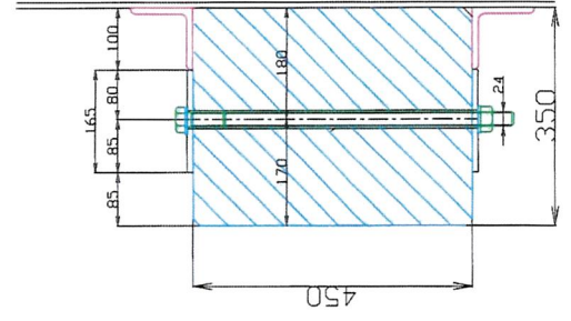
"CVE" WOOD FENDER MOUNT PIECE [EXISTING]
