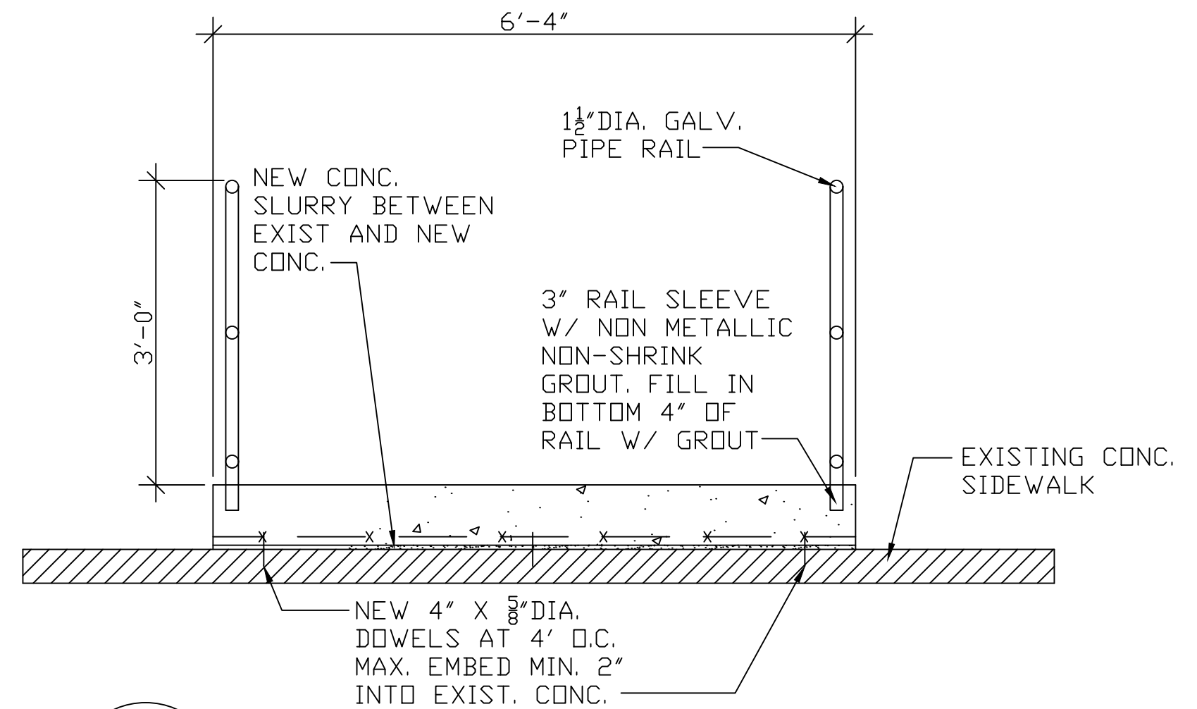
2 NEW RAMP TRANSVERSE SECTION A3 3/4" = 1'-0"
