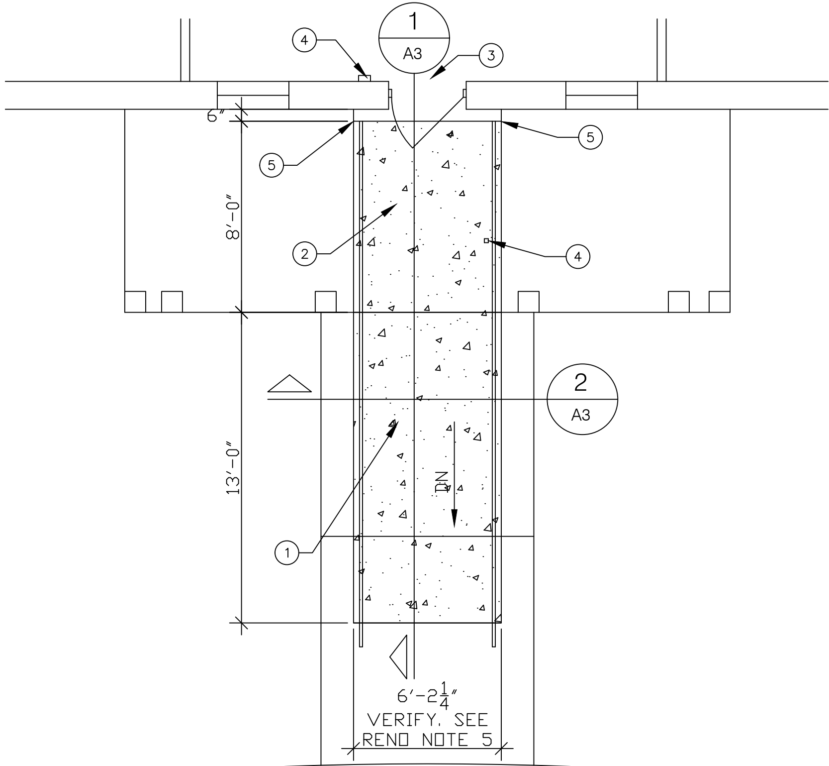
2 A2 NEW H.C. RAMP RENO PLAN 1/4" = 1'-0" 0 5' 10'
