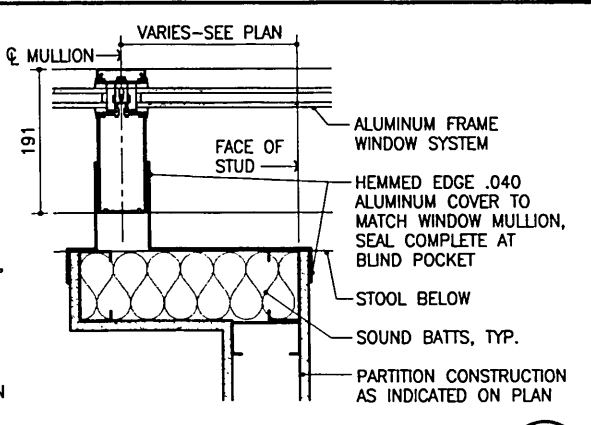
MULLION DETAIL 2
