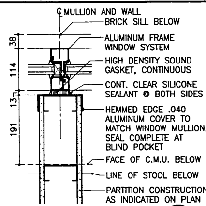
MULLION DETAIL 1
