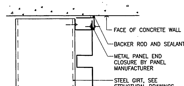
PANEL DETAIL 8
