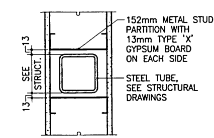
COLUMN DETAIL 7
