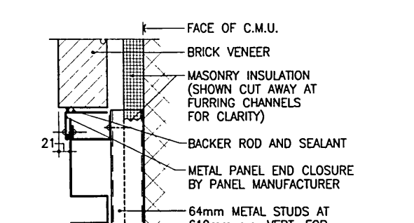
PANEL DETAIL 6
