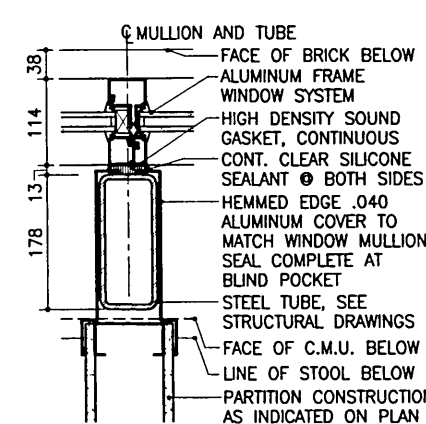
MULLION DETAIL 3
