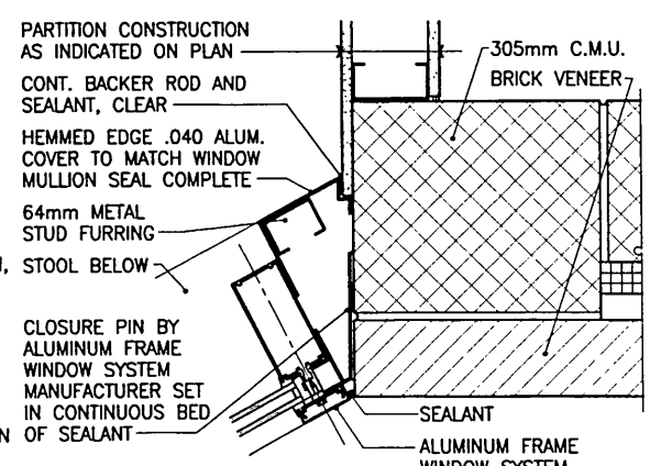
MULLION/JAMB DETAIL 4
